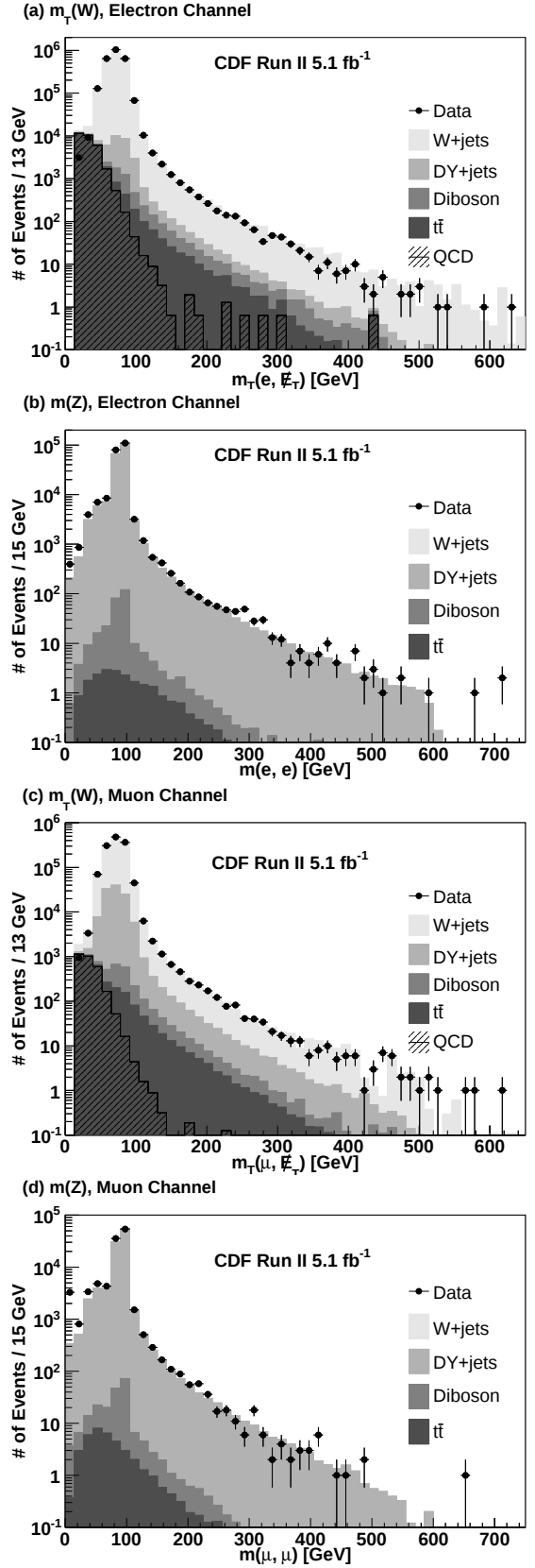
FIG. 2: (a) The transverse mass ( m_T ) of the highest- p_T lepton and the \cancel{E}_T in the electron-triggered W boson sample. (b) The dilepton invariant mass in the electron-triggered Z boson sample. (c) The m_T of the highest- p_T lepton and the \cancel{E}_T in the muon-triggered W boson sample. (d) The dilepton invariant mass in the muon-triggered Z boson sample. The estimation of the QCD contribution to these distributions is described in Section VI A. The points represent the observed data and the filled histograms are the SM estimates.
