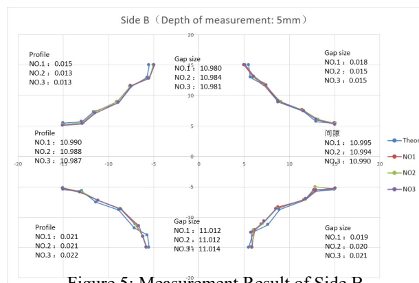
Figure 5: Measurement Result of Side B.
