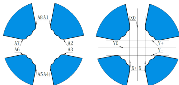
Figure 3: Survey Mark Point and Construction Plane.
