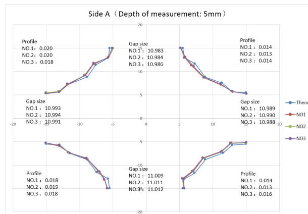
Figure 4: Measurement Result of Side A.
