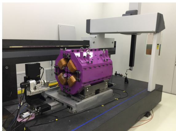
Figure 1: Testing Equipment and Magnet.
