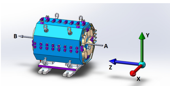
Figure 2: Schematic Diagram of Magnet Coordinate System.
