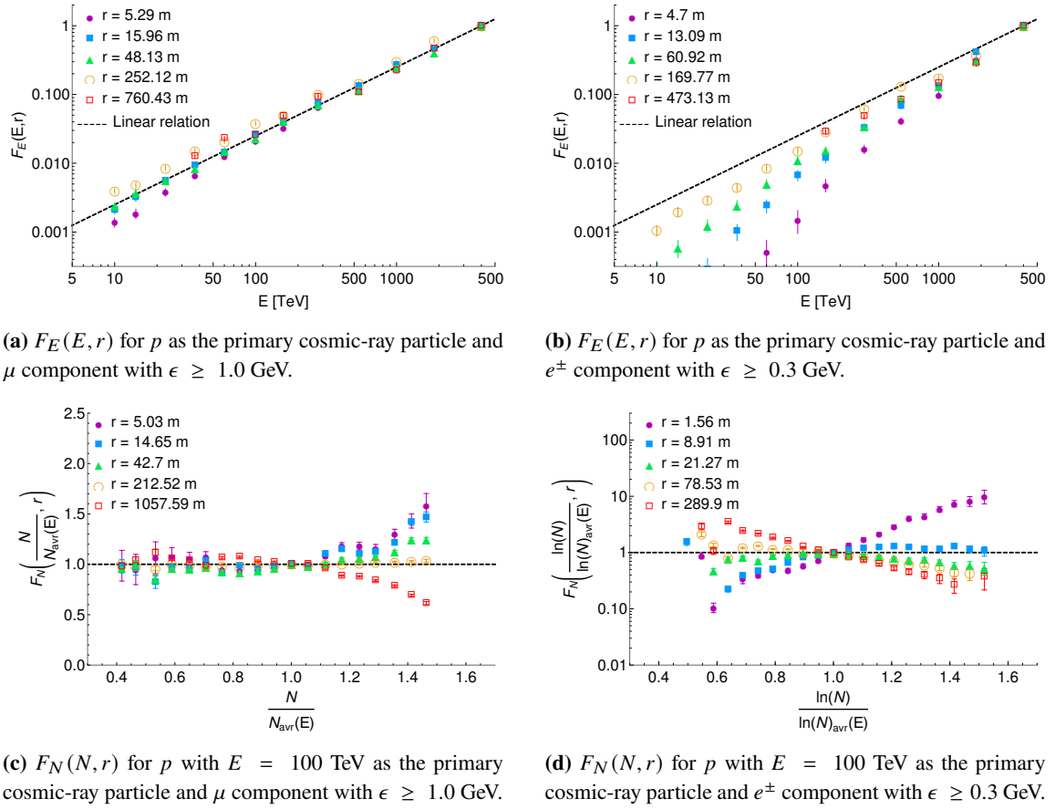
Figure 3: In Fig. 3a and 3b examples of F_E(E, r) are presented. Fig. 3c and 3d present exemplary factors F_N(N, r) .
