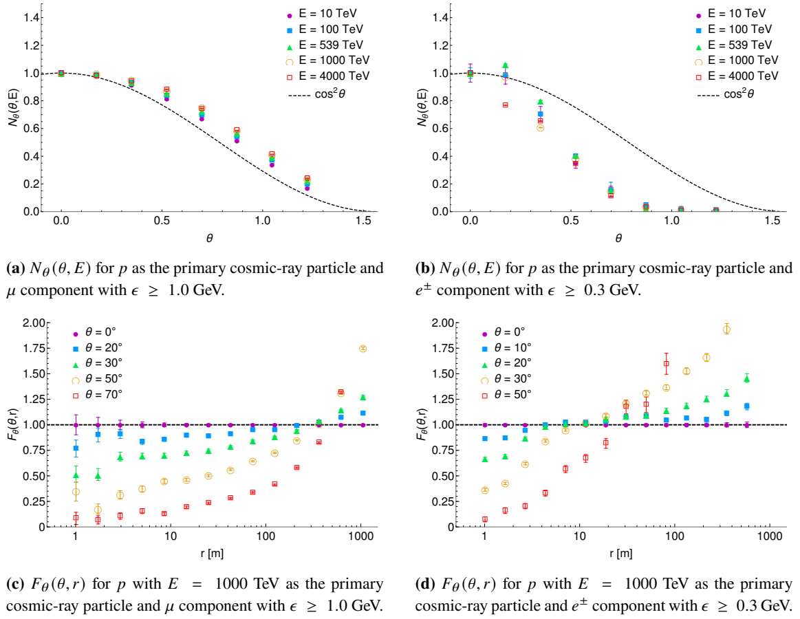
Figure 4: In Fig. 4a and 4b examples of N_\theta(\theta, E) are presented. Fig. 4c and 4d present exemplary factor F_\theta(\theta, r) .
