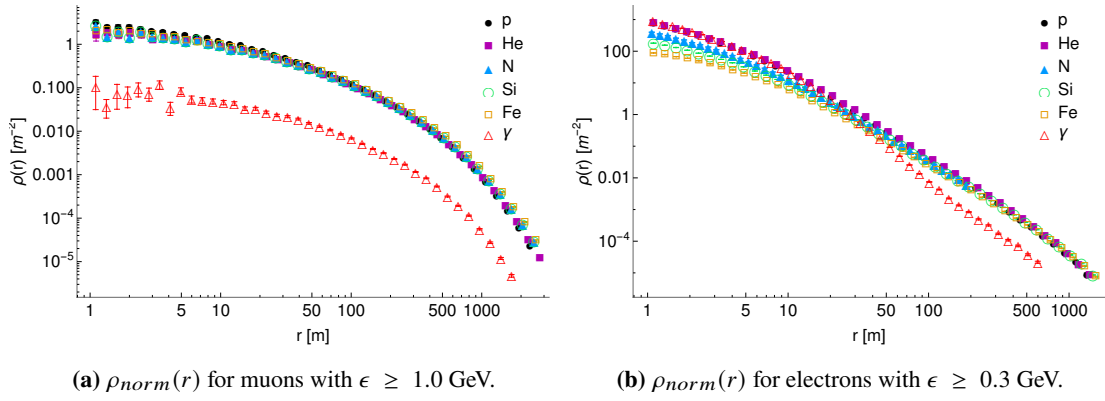
Figure 2: Density profile \rho_{norm}(r) of muons (a) and electrons (b) for vertical cascades for different primaries at energy E = 4000 TeV. Density profile of photons is not presented but it is very similar to that of electrons.
