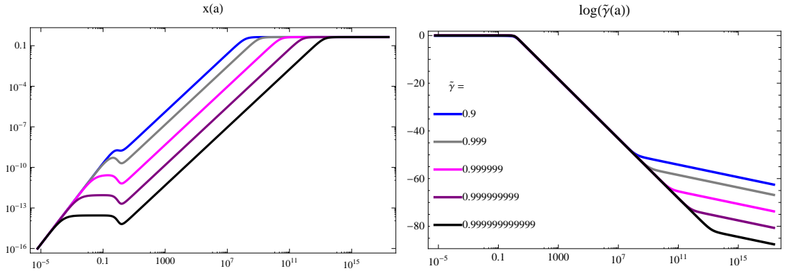
Figure 5.3: The evolution of the “kinetic term” x (left panel) and the brane Lorentz factor in the form of \log \tilde{\gamma} (right panel) as functions of the scale factor a when \Gamma_0 = 30 . The results are presented for five different initial conditions (set at a = 10^{-12} ) as given in the legend of the right panel. We see that x , initially set to a small value, grows until it reaches the attractor value given by Eq. (5.2.82). For sufficiently non-relativistic initial conditions ( \tilde{\gamma} very close to unity), x can be frozen during the matter dominated era but starts growing as the universe enters into the accelerating scaling saddle point solution Eq. (5.2.79). For sufficiently relativistic initial conditions ( \tilde{\gamma} very close to zero) this does not occur. During the matter dominated era \gamma is constant, but begins to evolve at a constant rate towards relativistic values \gamma \rightarrow \infty as the accelerating era begins. When the attractor is reached, this rate changes. The rate is given by \Gamma_0 in such a way that \gamma\phi \sim a^{-3w} where w is the equation of state parameter in Eq. (5.2.80), as expected from considerations in Section 5.2.1.
