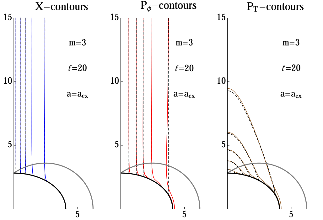
Figure 4.3: Approximate vs. numerical solution: In each case the numerical solution is shown in solid colour, and the approximation in dashed black. Contours of 0.1 - 0.9 (in steps of 0.2 ) of the range of each field are shown. From left to right: The Higgs field in blue, the P_\phi field in red, and P_T (the component with respect to the nonrotating frame at infinity) in brown. For P_T , we show contours of 0.1 - 0.9 of the maximal negative value, which is attained on the poles of the horizon. The outer grey curve represents the boundary of the ergosphere.
