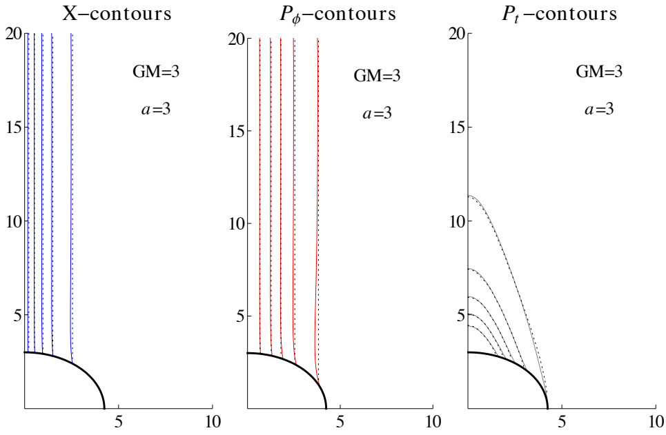
Figure 3.1: A comparison of the approximate and exact numerical solutions for an extremal GM = a = 3 Kerr black hole. In spite of the low value of black hole mass, (3.1.15) is still an extremely good approximation to the actual result. Here, the Higgs contours are in blue, the P_\phi contours in red, the P_t contours in grey, and all the corresponding approximate solution contours in dashed black. Contours are shown for X, P_\phi = 0.1, 0.3, 0.5, 0.7, 0.9 , and for P_t = -0.099, -0.077, -0.055, -0.033, -0.011 .
