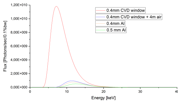
Figure 2: XOP results for bending magnet radiation behind.
