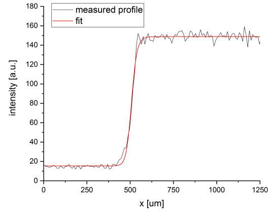
Figure 4: Resolution of the CCD camera with mirror and LuAG:Ce screen.
