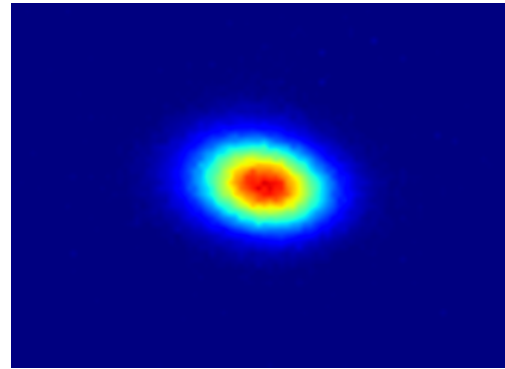
Figure 5: The image of the electron beam at 250 mA, horizontal/vertical emittances are 7.893/0.0626 nm respectively.
