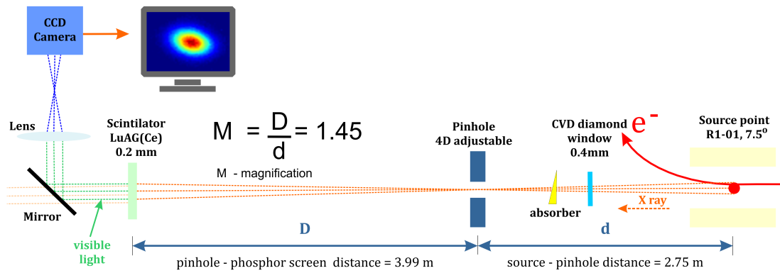
Figure 1: X-ray pinhole beamline schematic.
