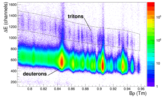
Figure 2. B\rho - \Delta E identification of the light particles using the split-pole focal-plane detectors. One can see the deuteron loci extending into the triton region.
