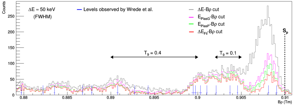
Figure 3. Focal-plane triton spectra from the ^{31}\text{P}(^3\text{He}, t)^{31}\text{S} reaction at 25 MeV and \theta_{\text{lab}} = 10^\circ , for 7% of all statistic. The effect of the different cuts using combination of focal-plane detectors signals are shown and the final spectrum (in red) can be compared to the levels observed by Wrede et al. (in blue).
