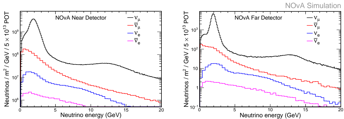
Figure 2.14: Predicted PPFX/-based composition of the NuMI beam in the FHC beam mode (neutrino-enhanced) at the ND (left) and the FD (right). Curves from top to bottom: \nu_\mu , \bar{\nu}_\mu , \nu_e , \bar{\nu}_e . The Table 2.1 gives the fractional composition for each neutrino flavor integrated from 1-5 GeV. From [33].
