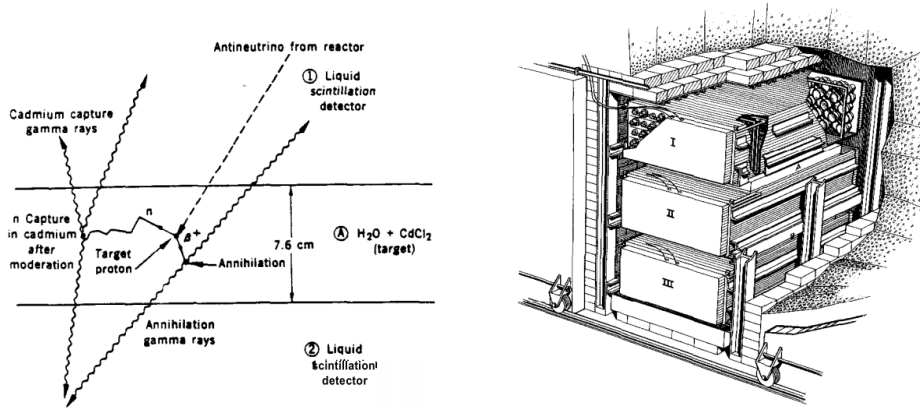
Figure 1.3: The Savannah River experiment by Reines and Cowan. Left: Diagram of the detection technique. An antineutrino from the reactor interacts in the detector producing a positron and a neutron. The positron annihilation creates photons that are detected in the scintillator. The delayed capture of the neutron after it slows down also generates scintillation light. Right: experimental setup. Tanks A and B contain water and dissolved \text{CdCl}_2 . Tanks I, II and III are filled with scintillators and instrumented with PMTs. From [11].
