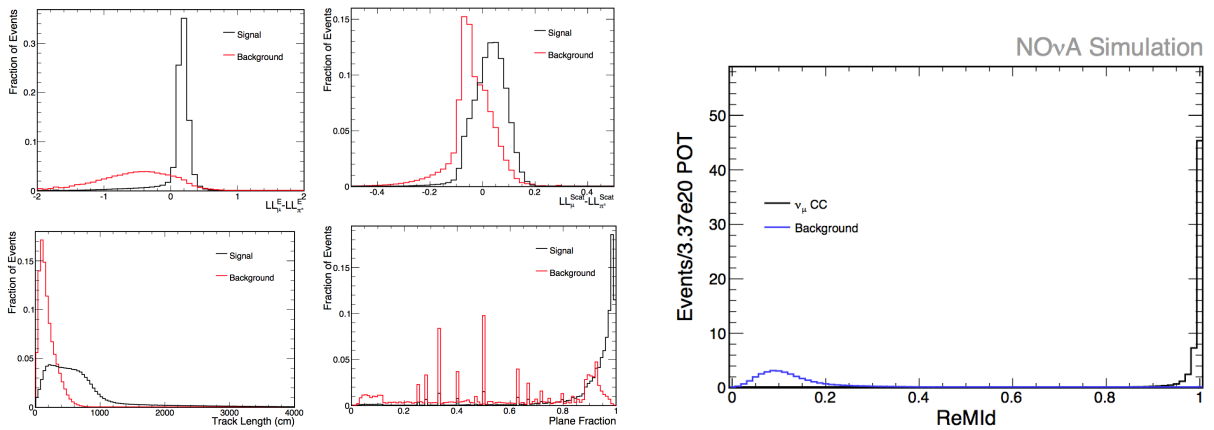
(a) Input variables for the kNN training: dE/dx likelihood (top left), scattering likelihood (top right), track length FD. (bottom left), plane fraction (bottom right). (b) ReMId score for a \nu_\mu -selected sample in the
