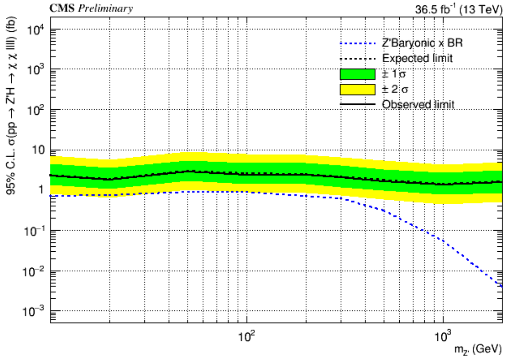
Figure 6.4: One-dimensional cross section times branching fraction limits for the Z_p Baryonic simplified model using the cut-and-count based event selection strategy.
