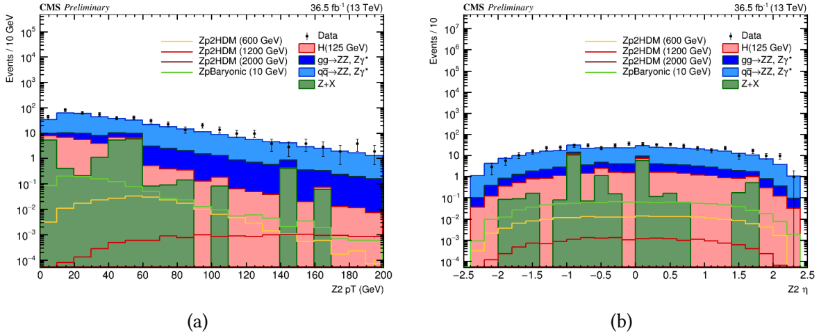
Figure 5.7: Kinematic distributions for the Z_2 at the ZZ candidate selection step: (a) p_T and (b) \eta .
