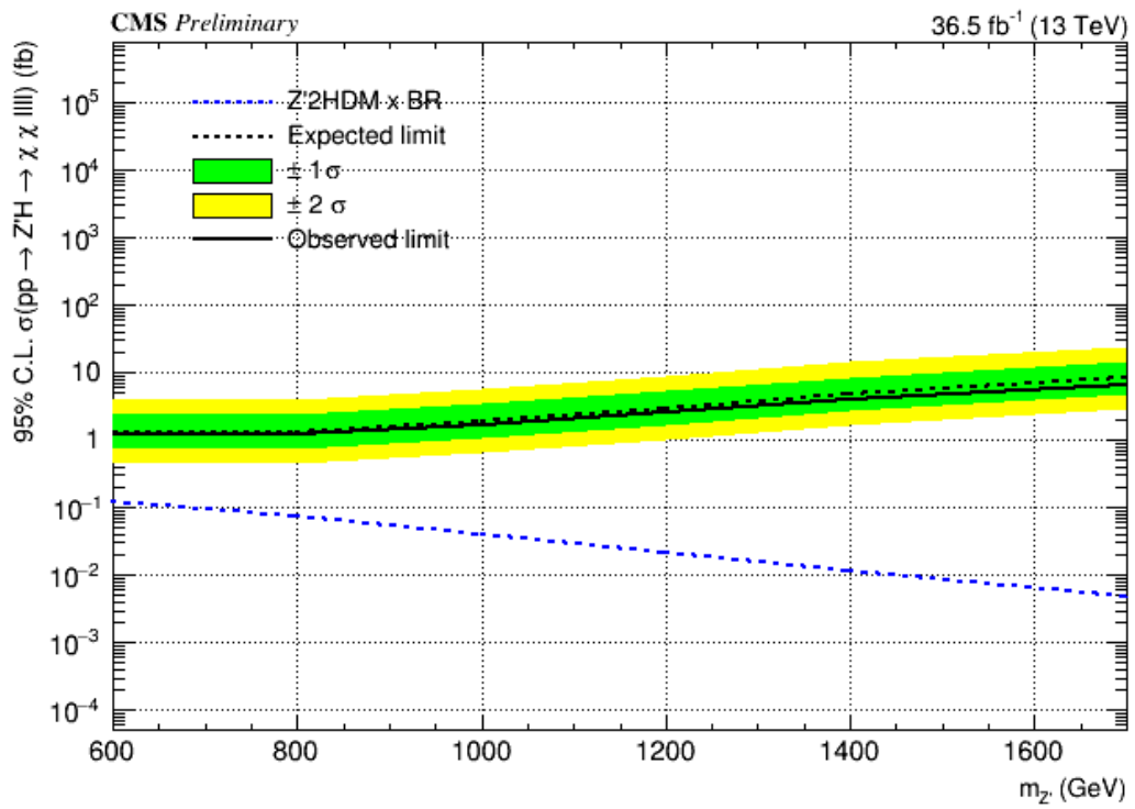
Figure 6.5: One-dimensional cross section times branching fraction limits for the Zp2HDM simplified model using the MVA-based event selection strategy.
