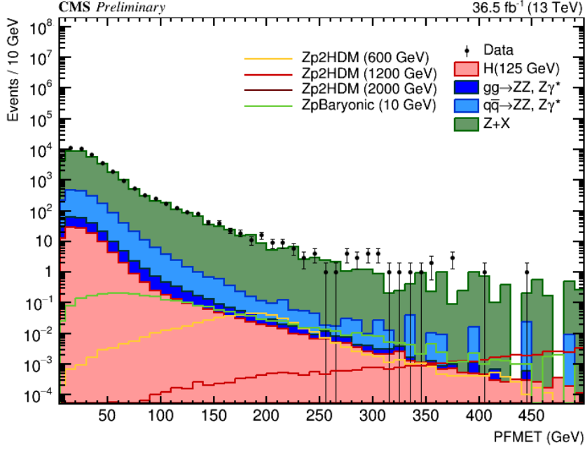
Figure 4.12: Missing transverse energy (MET) after the first Z selection step before removal of fake MET.
