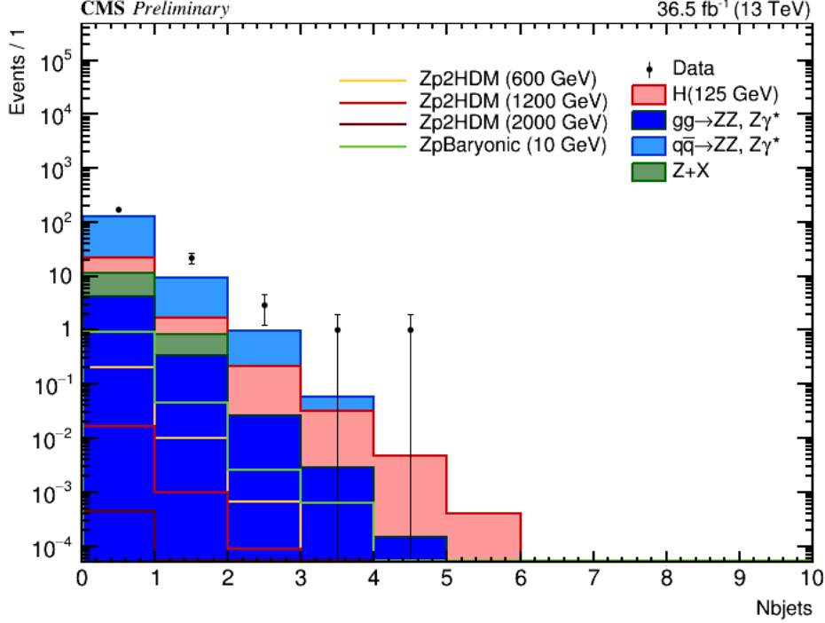
Figure 5.18: b-jet multiplicity after the final SM selection.
