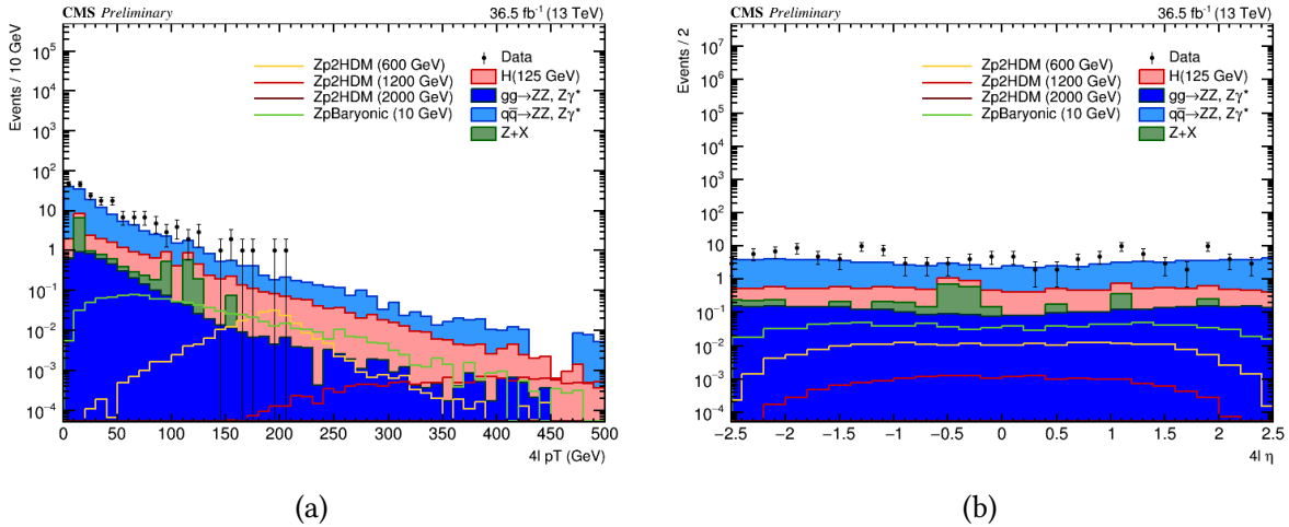
Figure 5.11: Kinematics of the four-muon object after the final SM selection: (a) transverse momentum and (b) \eta .
