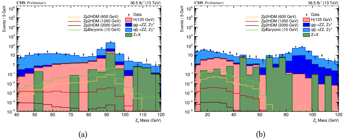
Figure 5.5: Dimuon invariant mass at the ZZ candidate selection step for (a) Z_1 and (b) Z_2 .
