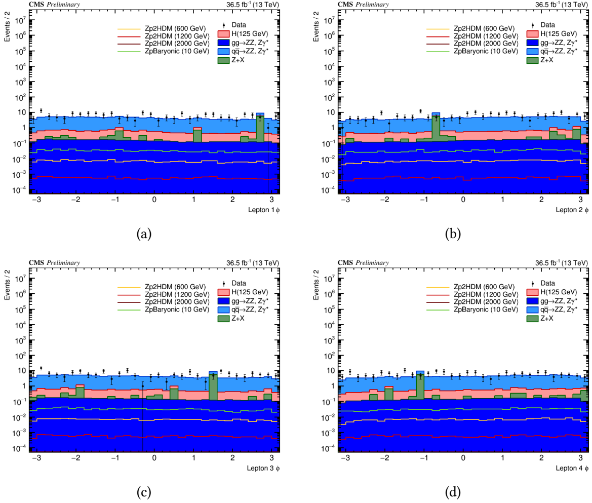
Figure 5.15: \phi distributions for the constituent leptons of the Z_1 , (a) and (b), and of the Z_2 , (c) and (d) after the final SM selection step.
