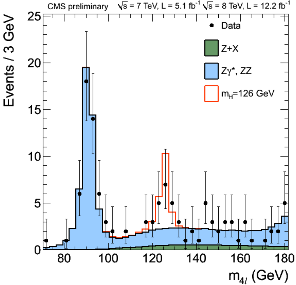
Figure 1.2: Four-lepton invariant mass distribution showing H discovery in the ZZ^* decay channel. The red line shows the signal distribution for m_H = 126 \text{ GeV} [1].
