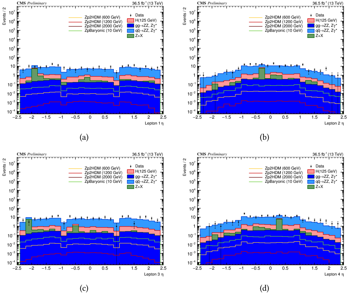
Figure 5.14: \eta distributions for the constituent leptons of the Z_1 , (a) and (b), and of the Z_2 , (c) and (d) after the final SM selection step.
