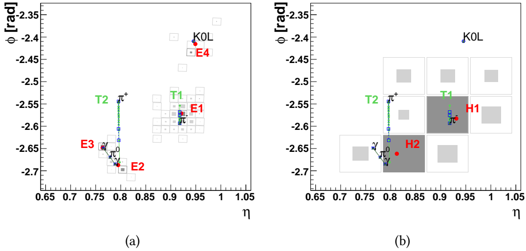
Figure 3.2: Event display of hadronic jet in the \eta - \phi plane for the ECAL (a) and HCAL (b). The locations of clusters are given by the solid dots [4].
