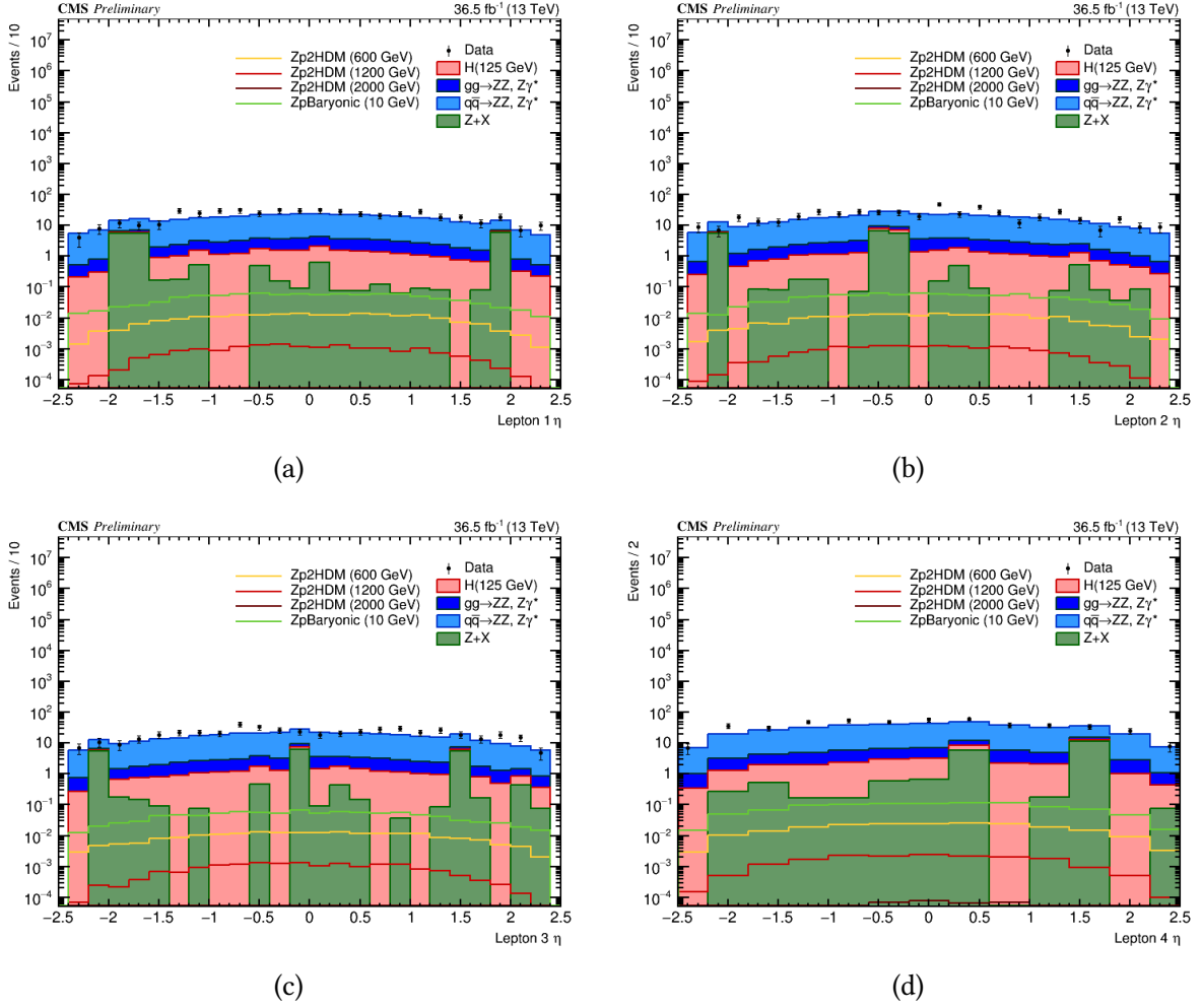
Figure 5.9: \eta distributions for the constituent leptons of the Z_1 , (a) and (b), and of the Z_2 , (c) and (d) at the ZZ candidate selection step.
