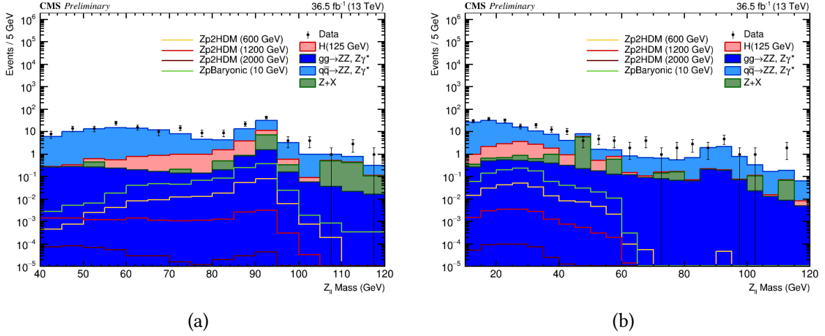
Figure 5.12: Dimuon invariant mass distributions after the final SM selection for (a) Z_1 and (b) Z_2 .
