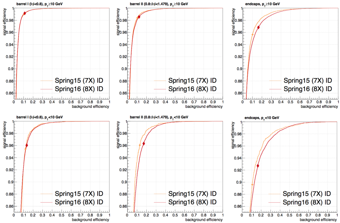
Figure 4.2: Performance comparison of the MVA trained for the 2015 analysis and the retraining for 2016 conditions. The respective working points are indicated by the markers.
