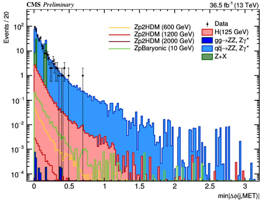
Figure 4.14: Minimum azimuthal angle difference between MET and jets.
