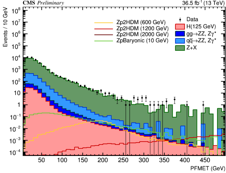
Figure 5.4: Missing transverse energy distribution at the Z candidate selection step.
