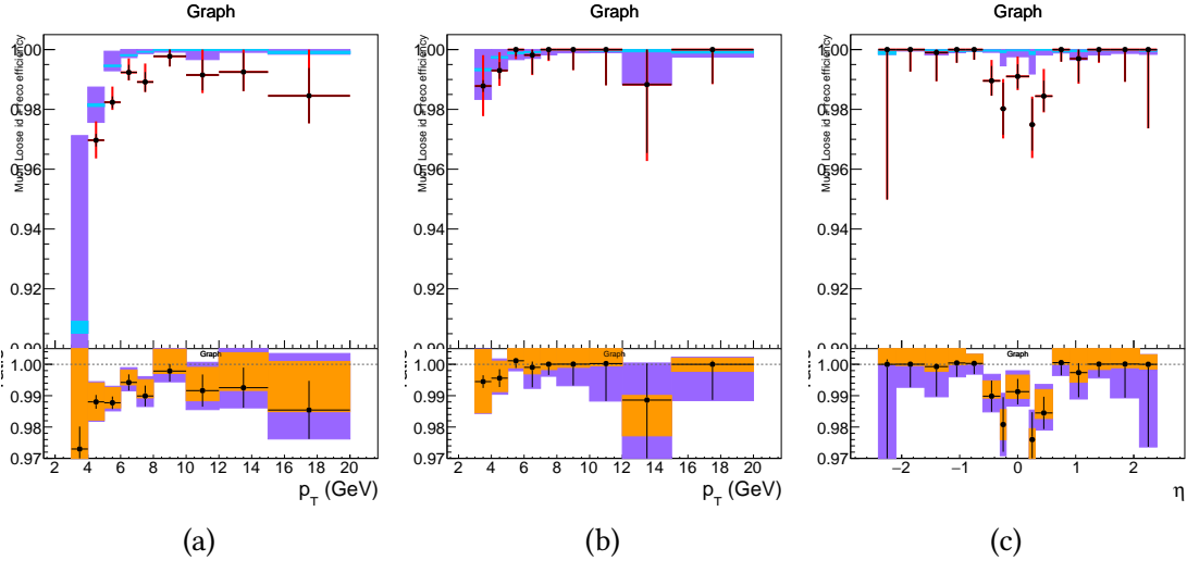
Figure 4.7: Muon reconstruction and identification efficiency at low p_T , measured with the tag-and-probe method on J/\Psi events, as function of p_T in the barrel (a) and end caps (b), and as function of \eta for p_T > 7 GeV (c). In the upper panel of each graph, the larger error bars include also the systematical uncertainties, while the smaller ones are purely statistical. Each graph's lower panel shows the ratio of the two efficiencies, the black error bars are for the statistical uncertainty, the orange rectangles for the systematic uncertainty, and the violet rectangles include both uncertainties.
