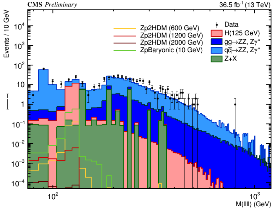
Figure 5.10: Four-muon invariant mass distribution at the ZZ selection step in log scale.
