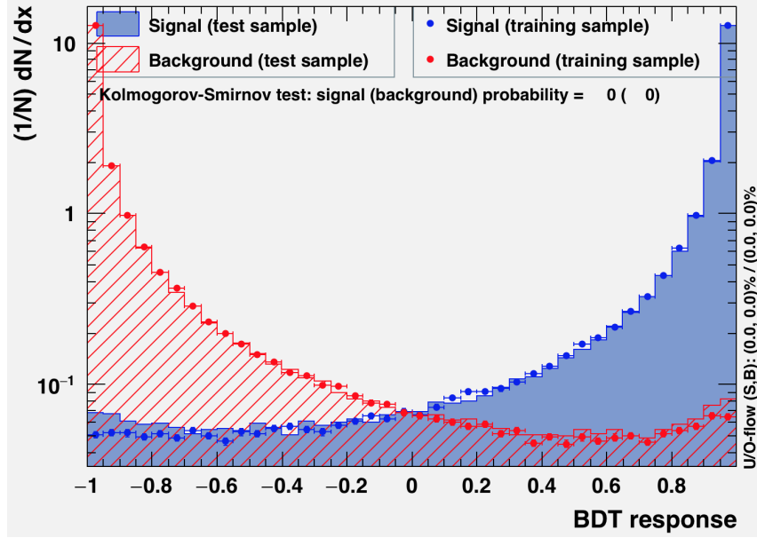
Figure 4.3: Boosted decision tree output for the training and testing sample for true and fake electrons in the high- p_T end cap training bins.
