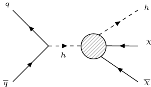
Figure 1.4: Collider production diagram for mono-Higgs effective field theories.
