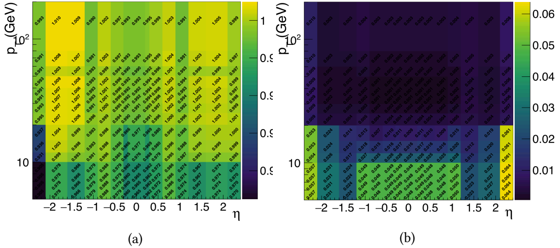
Figure 4.11: (a) Overall data to simulation scale factors for muons, as function of p_T and \eta . (b) Uncertainties on data to simulation scale factors for muons, as function of p_T and \eta .
