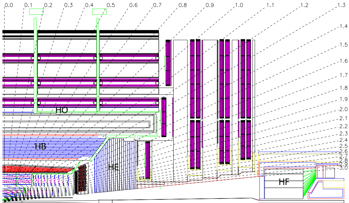
Figure 2.7: Cross sectional view of one quadrant of CMS. The labeled sections are the sub-systems of the hadronic calorimeter [2].
