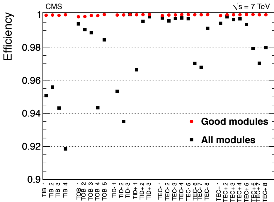
Figure 2.4: Average hit efficiencies of the strip tracker layers [2].
