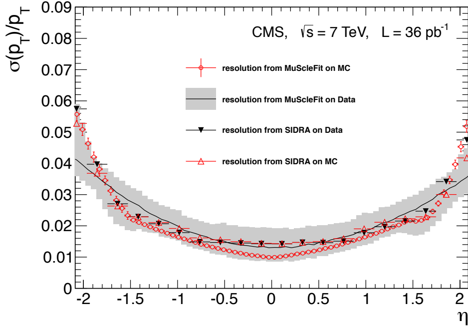
Figure 2.12: Transverse momentum resolution versus pseudorapidity for muons from Z decays [3].
