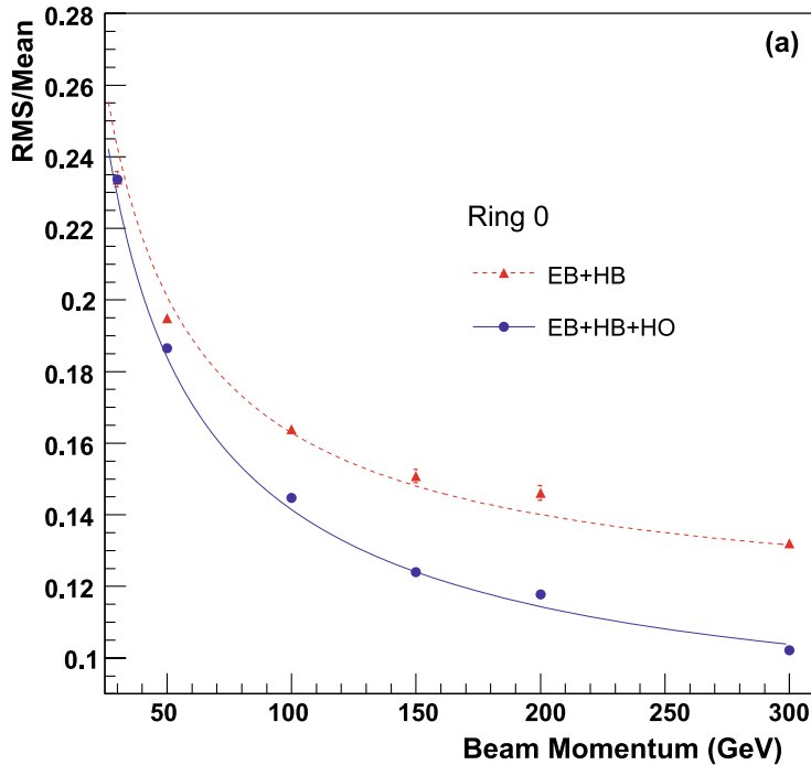
Figure 2.8: Energy resolution of HCAL systems for test beam pions [2].
