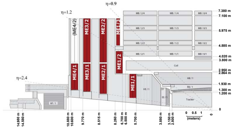
Figure 2.10: Schematic diagram showing CSC locations in red in a quadrant cutout of CMS [2].
