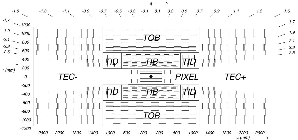
Figure 2.2: Schematic diagram of tracking detectors with radial distance of modules, shown as black lines, from center on the left axis, z -dimension on the bottom axis, and \eta across the top [2].
