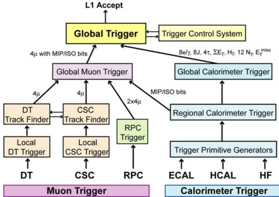
Figure 2.13: CMS L1 trigger system schematic diagram [2].
