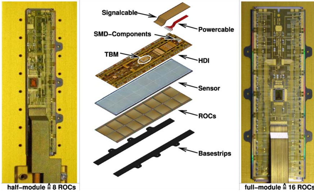
Figure 2.3: Deconstructed barrel pixel module showing module components [2].
