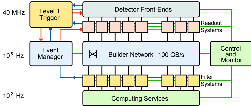
Figure 2.14: CMS data acquisition system schematic diagram [2].
