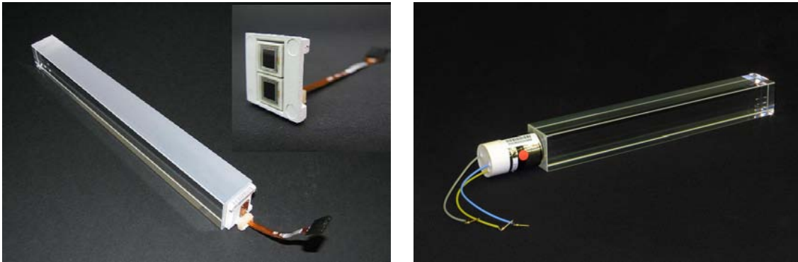
Figure 2.6: ECAL barrel crystal with one depolished face attached to avalanche photodiode photodetector (left) and ECAL end cap crystal attached to vacuum phototriode (right) [2].
