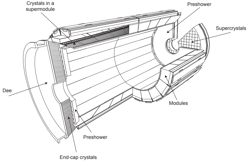
Figure 2.5: Schematic layout of the ECAL crystal modules [2].
