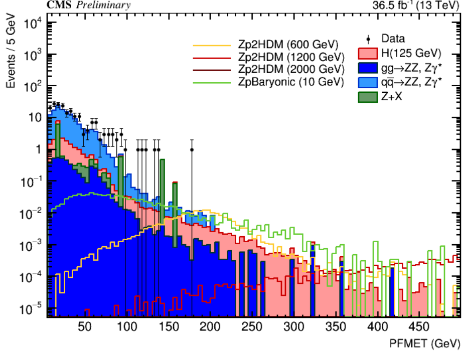
Figure 5.16: Missing transverse energy after the final SM selection step.
