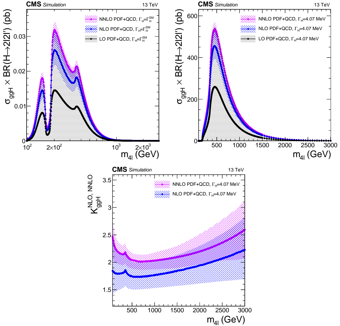
Figure 5.21: gg \rightarrow H \rightarrow 2\ell 2\ell' cross sections at NNLO, NLO and LO at each H pole mass using the SM H decay width (top left) or at the fixed and small decay width of 4.07 MeV (top right). The cross sections using the fixed value are used to obtain the k -factor for both the signal and the continuum background contributions as a function of m_{4\ell} (bottom).
