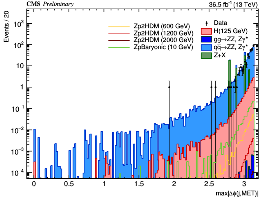
Figure 4.13: Maximum azimuthal angle difference between MET and jets.
