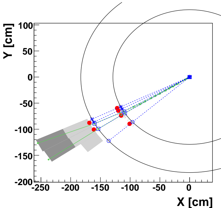
Figure 3.1: Event display of hadronic jet in the x - y plane, with solid arcs at the ECAL and HCAL surfaces. The locations of clusters are given by the solid dots [4].
