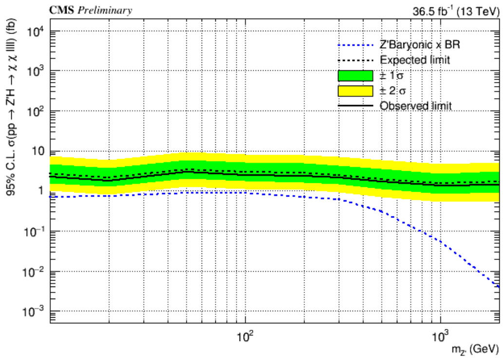
Figure 6.6: One-dimensional cross section times branching fraction limits for the ZpBaryonic simplified model using the MVA-based event selection strategy.
