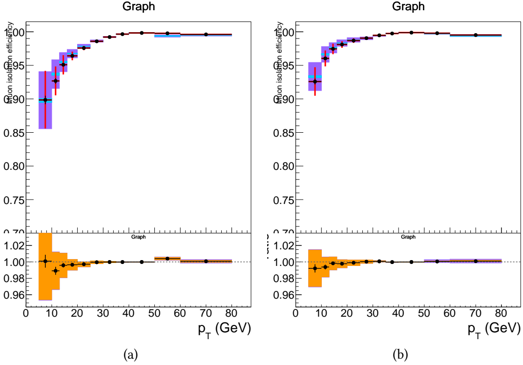
Figure 4.9: Efficiency of the muon isolation requirement, measured with the tag-and-probe method on Z events, as function of p_T in the barrel (left) and end caps (right). In the upper panel of each graph, the larger error bars include also the systematical uncertainties, while the smaller ones are purely statistical. The lower panel of each graph shows the ratio of the two efficiencies, the black error bars are for the statistical uncertainty, the orange rectangles for the systematical uncertainty, and the violet rectangles include both uncertainties.
