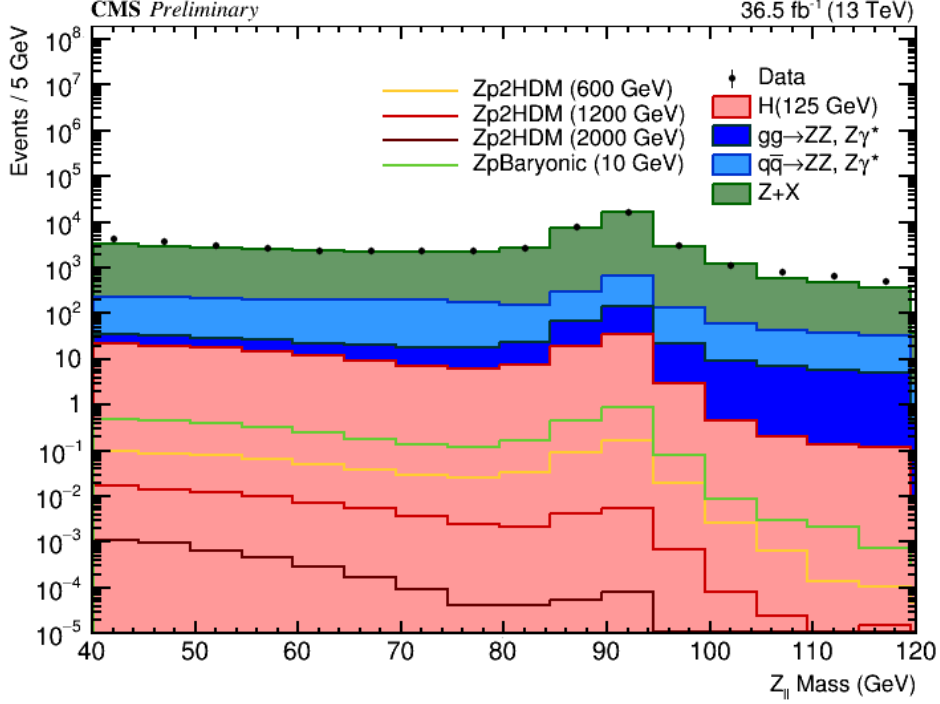
Figure 5.3: Dimuon invariant mass distribution for Z candidates.
