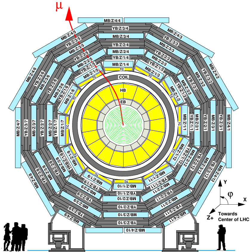
Figure 2.9: Schematic diagram showing DT chambers in light blue [2].
