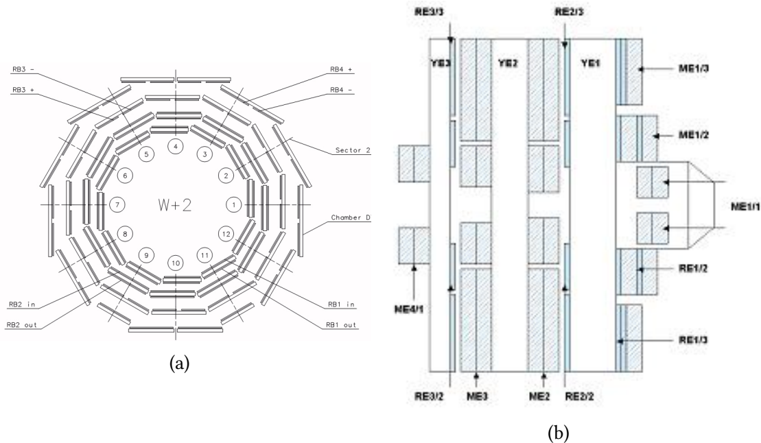
Figure 2.11: Schematic diagram showing barrel RPC locations (left) and end cap RPCs (right) in a cross sectional cutout of CMS [2].
