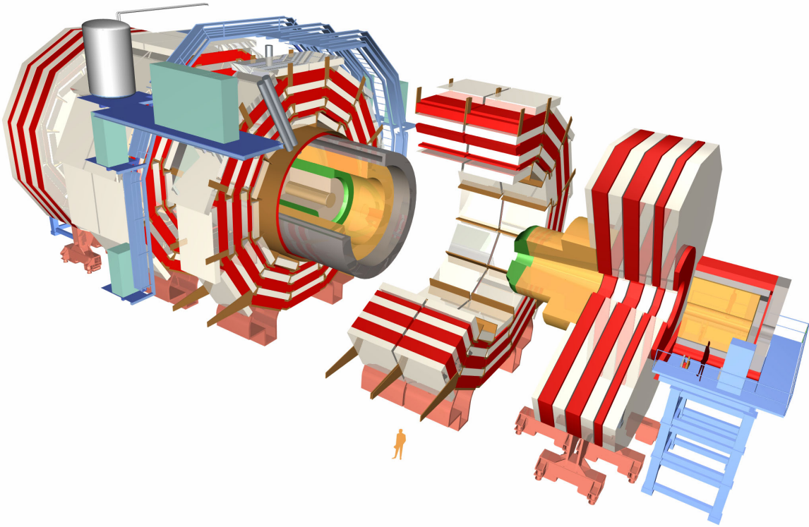
Figure 2.1: Deconstructed view of the CMS subdetectors, with human figure for scale. From inside to out, the colored segments correspond to the following systems: light brown is the pixel tracker, cream is the strip tracker, green is the EM calorimeter, orange is the hadronic calorimeter, grey is the solenoid, red is the yoke with white muon chambers [2].
