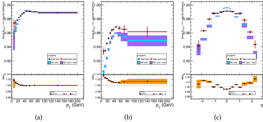
Figure 4.8: Efficiency of the muon impact parameter requirements, measured with the tag-and-probe method on Z events, as function of p_T in the barrel (a) and end caps (b), and as function of \eta for p_T > 20 GeV (c). In the upper panel of each graph, the larger error bars include also the systematical uncertainties, while the smaller ones are purely statistical. Each graph's lower panel shows the ratio of the two efficiencies, the black error bars are for the statistical uncertainty, the orange rectangles for the systematical uncertainty, and the violet rectangles include both uncertainties.
