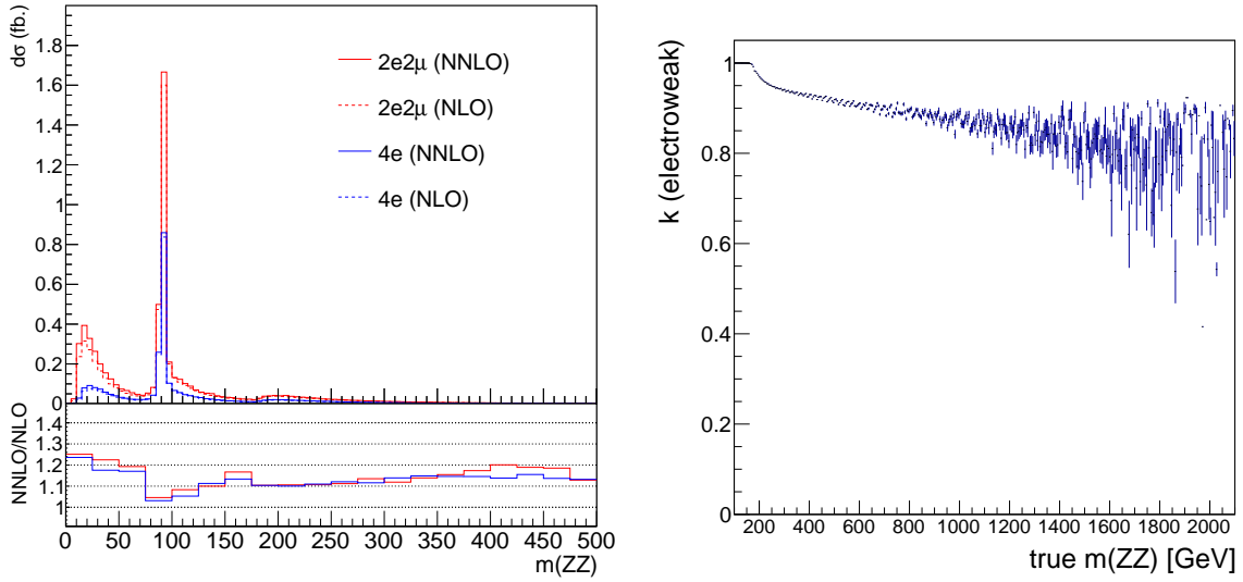
Figure 5.20: Left: NNLO/NLO QCD k -factor for the q\bar{q} \rightarrow ZZ background as a function of m(ZZ) for the 4\ell and 2\ell 2\ell' final states. Right: NLO/NLO electroweak k -factor for the q\bar{q} \rightarrow ZZ background as a function of m(ZZ) .
