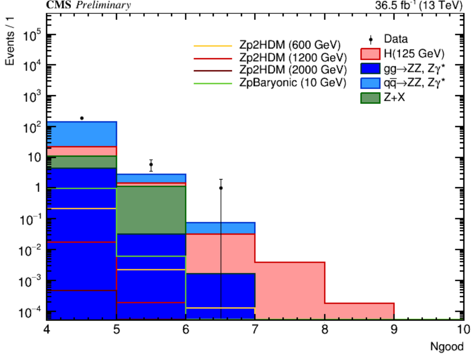
Figure 5.17: Tight-lepton multiplicity after the final SM selection.
