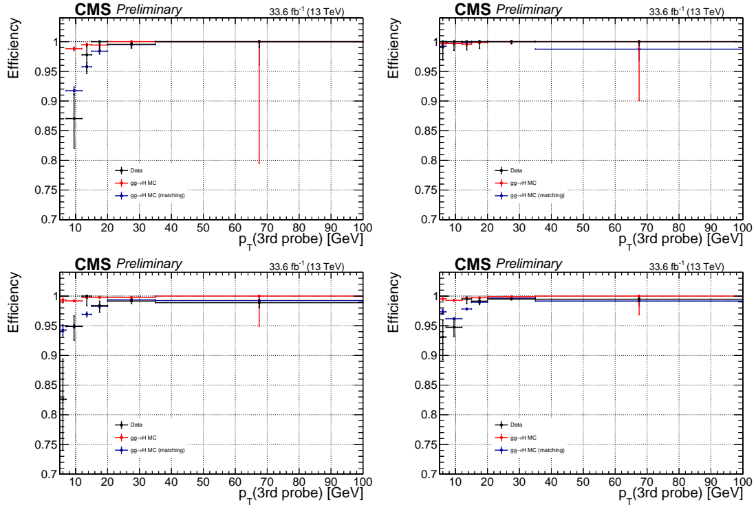
Figure 3.4: Trigger efficiency measured in data using 4\ell events collected by single lepton triggers for the 4e (top left), 4\mu (top right), 2e2\mu (bottom left) and 4\ell (bottom right) final states.
