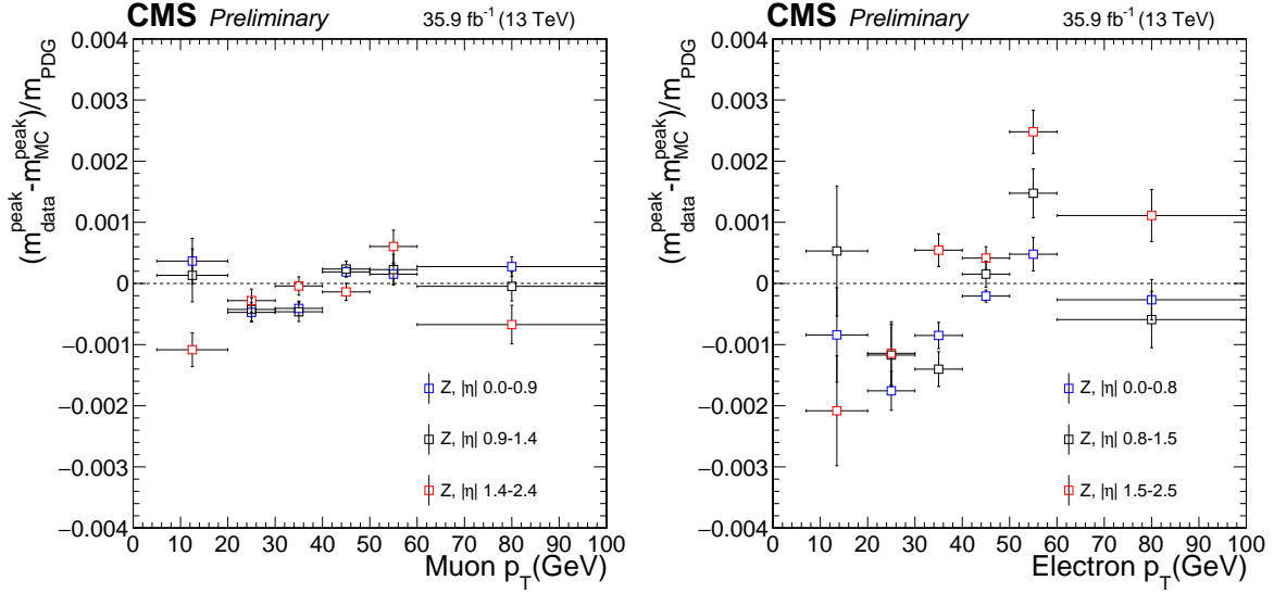
Figure 6.1: Difference between the Z \rightarrow \ell\ell mass peak positions in data and simulation normalized by the nominal Z boson mass obtained as a function of the p_T and |\eta| of one of the leptons, regardless of the second, for muons (left) and electrons (right).
