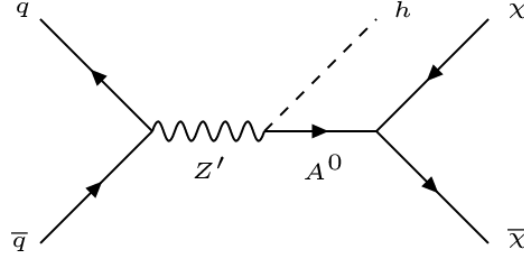
Figure 1.5: Collider production diagram for Zp2HDM.
