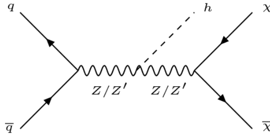
Figure 1.6: Collider production diagram for Z' models.
