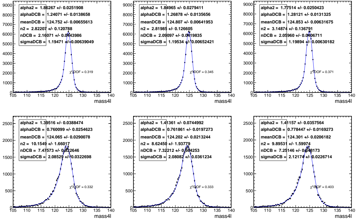
Figure 6.2: Different m_{4\ell} distributions after propagating the biases in Fig. 6.1 to Higgs boson events. The change in the mean of the double Crystal-Ball is used to determine the systematic uncertainty due to the lepton momentum scale. The middle plot shows the nominal distribution, while the left (right) plots show the down (up) systematic variations. The 4\mu channel is shown in the top row and the 4e channel is shown in the bottom row.
