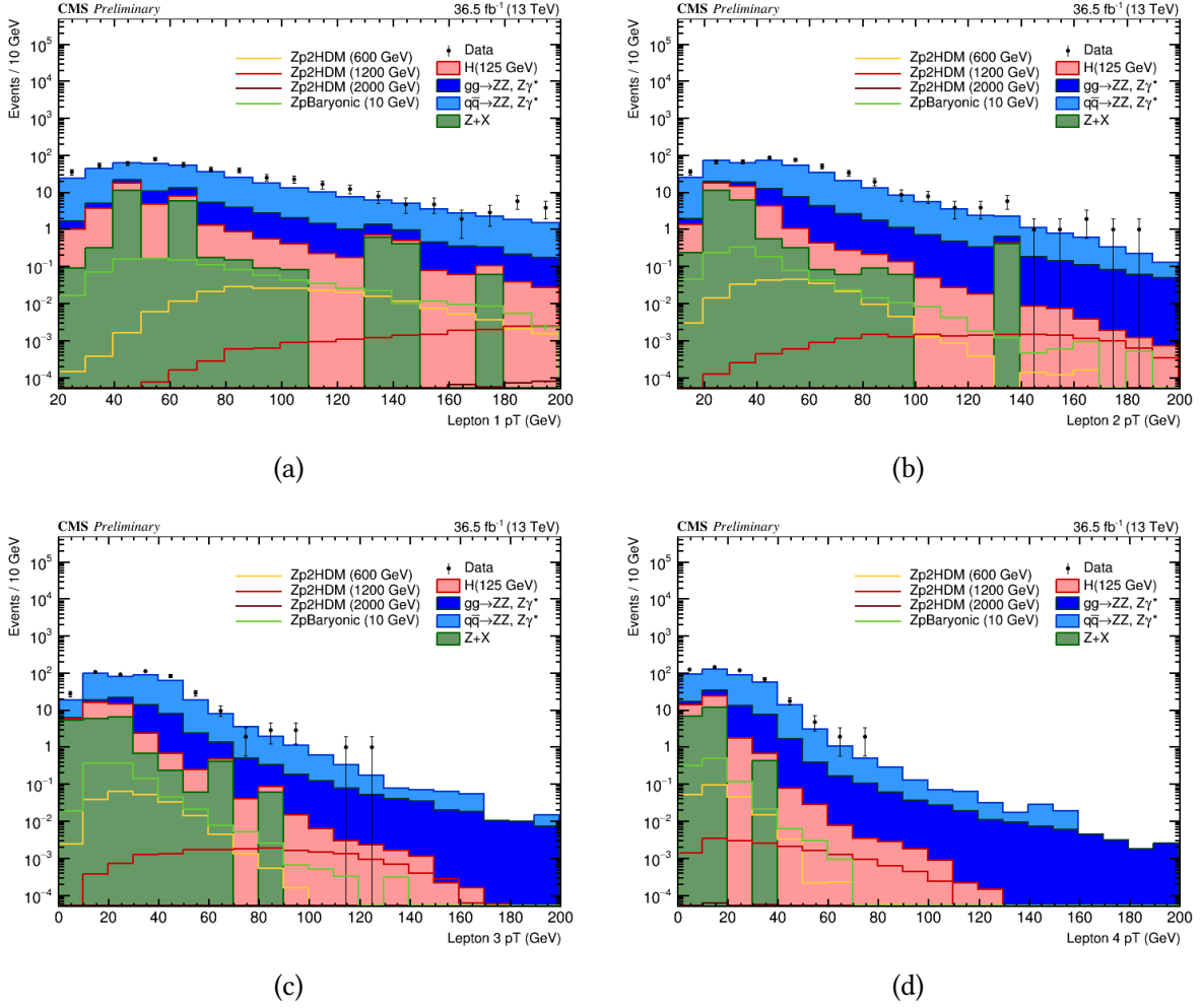
Figure 5.8: Transverse momentum distributions for the constituent leptons of the Z_1 , (a) and (b), and of the Z_2 , (c) and (d) at the ZZ candidate selection step.
