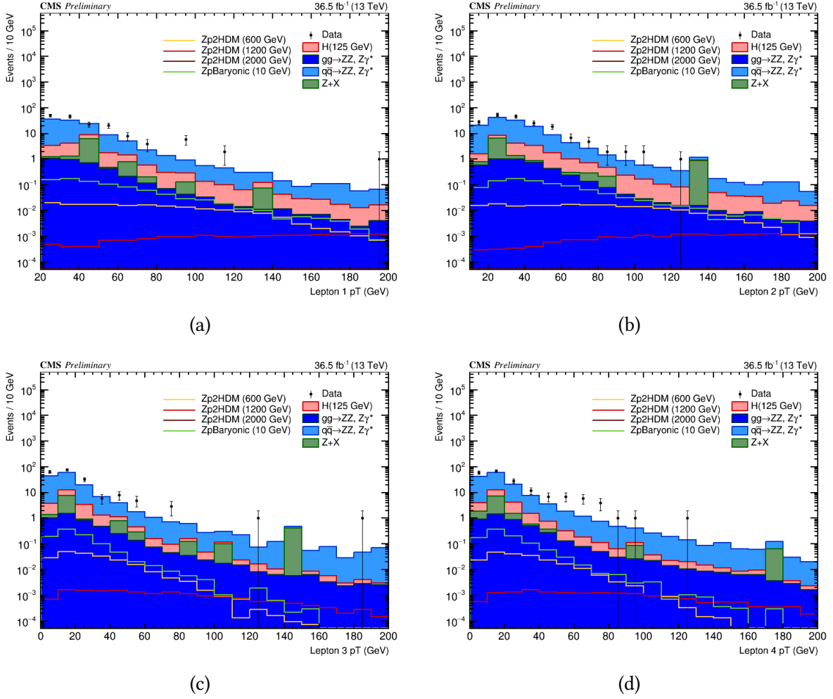
Figure 5.13: Transverse momentum distributions for the constituent leptons of the Z_1 , (a) and (b), and of the Z_2 , (c) and (d) after the final SM selection step.
