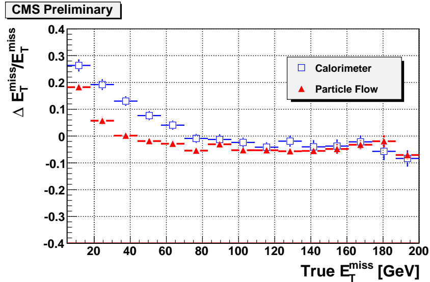
Figure 3.3: Missing transverse energy reconstruction resolution using the particle flow algorithm [4].
