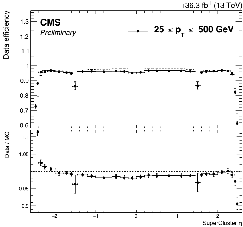
Figure 4.1: Electron reconstruction efficiencies in data (top) and data to simulation scale factors (bottom).
