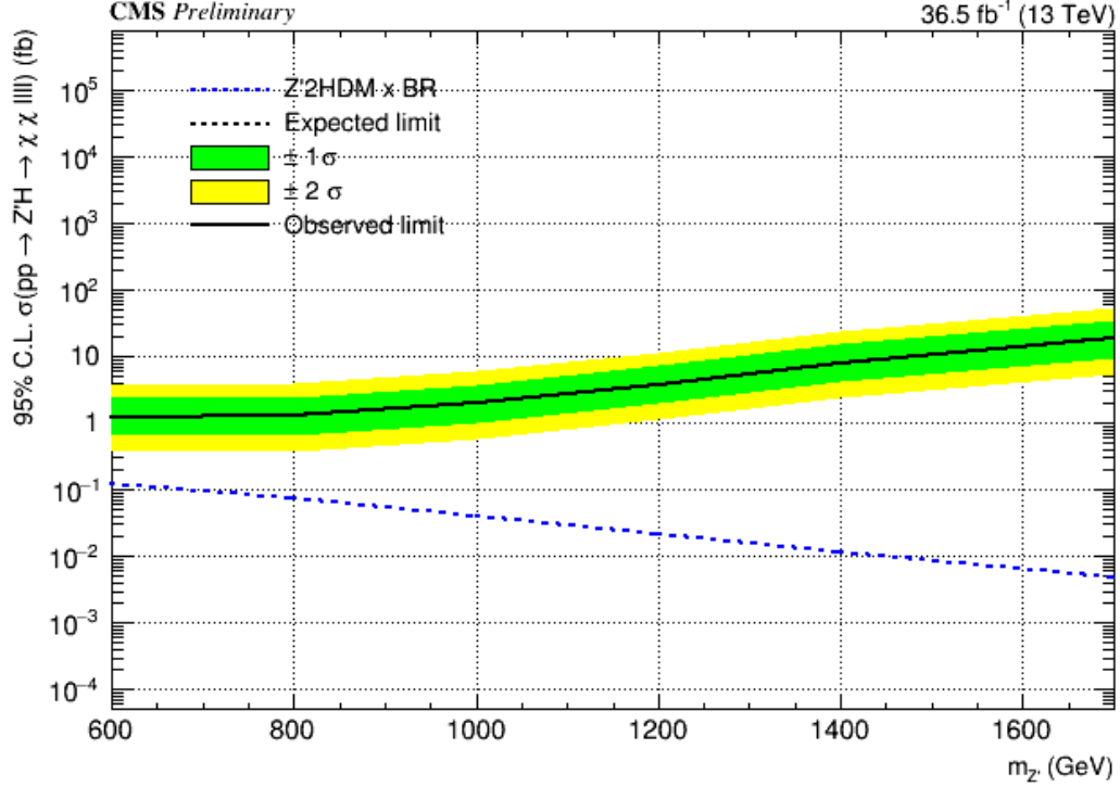
Figure 6.3: One-dimensional cross section times branching fraction limits for the Zp2HDM simplified model using the cut-and-count based event selection strategy.
