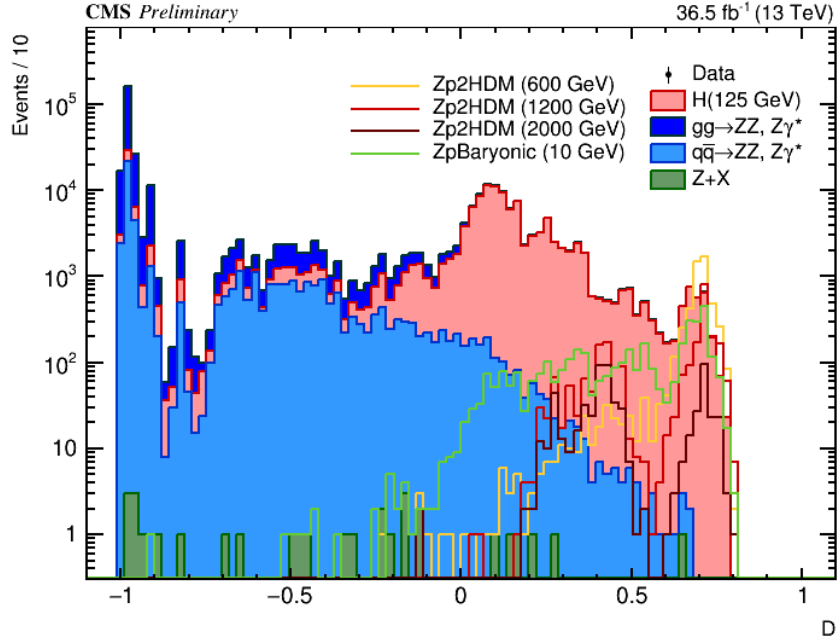
Figure 5.19: MVA response trained on a weighted background sample and admixture of signal samples with input variables m_{4\ell} and E_T^{\text{MISS}} .
