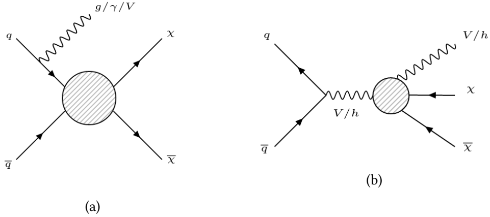
Figure 1.3: (a) Mono- X production topology for signatures with X emitted as ISR. (b) Mono- X production topology for signatures with X emitted from new physics vertex.
