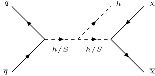
Figure 1.7: Collider production diagram for Scalar model.
