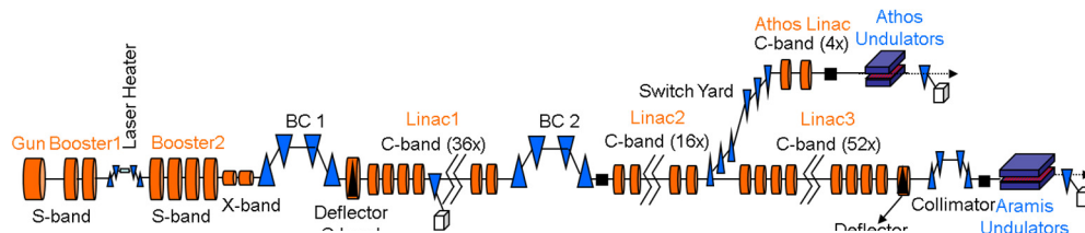
Figure 1: Layout of SwissFEL
