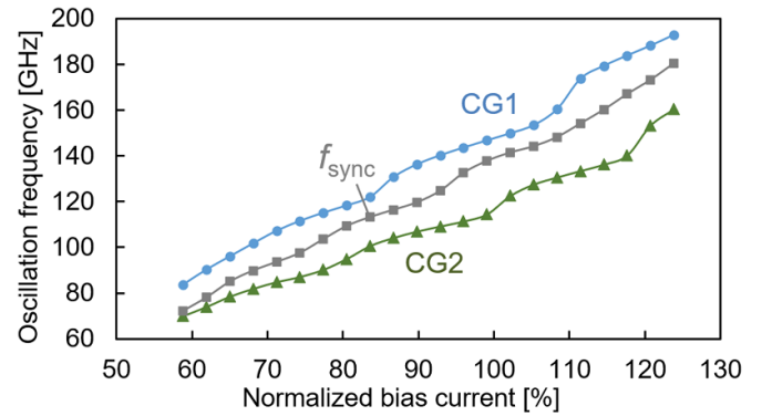
Figure 7. Measured dependences of the oscillation frequencies of test circuits. f_{\text{sync}} is the measured result for the test circuit in figure 6. CG1 and CG2 refer to the individual test results of CG1 and CG2, respectively.
