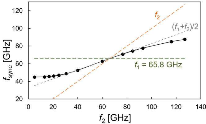
Figure 5. Simulated dependence of the synchronization frequency on the oscillating frequency of CG2. The dots represent the simulated f_{\text{sync}} . The dashed lines are inserted to discuss the simulation result. The oscillation frequency of CG1 ( f_1 ) is fixed at 65.8 GHz.
