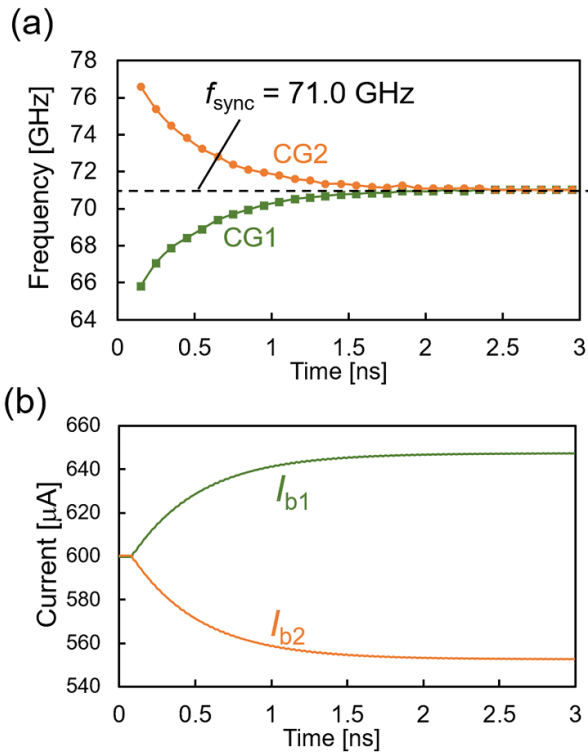
Figure 4. Simulated transition of (a) oscillating frequencies of CG1 and CG2 and (b) bias currents supplied to CG1 and CG2. L_c = 100 pH. The oscillations of both CG1 and CG2 commence at 100 ps.
