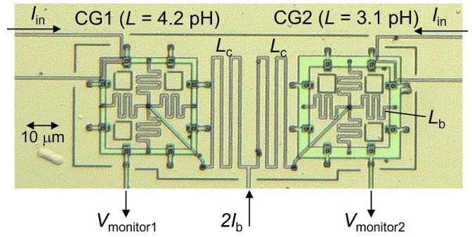
Figure 6. Photomicrograph of the test circuit used to demonstrate frequency synchronization. V_{\text{monitor1}} and V_{\text{monitor2}} are terminals for measuring the average voltage of the Josephson junctions in the corresponding SFQ oscillators. The Josephson junctions are shunted using 11.32 \Omega in order to set the McCumber–Stewart parameter to 2. L_c = 100 pH and L_b = 25.0 pH.
