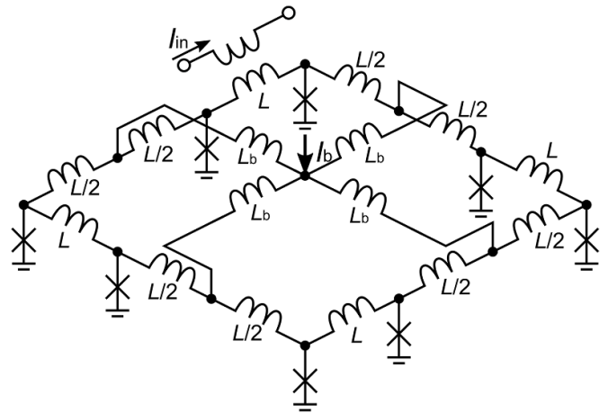
Figure 1. Equivalent circuit of the SFQ oscillator. The cross symbols in the figure represent Josephson junctions. The critical currents of all the Josephson junctions are 100 \mu\text{A} ; L_b = 25.0 \text{ pH} , and I_b = 600 \mu\text{A} . I_{in} is used to inject the flux quantum into the SFQ oscillator and start oscillation. The McCumber–Stewart parameter [24, 25] for all the Josephson junctions is 0.89, which is the standard value in the CONNECT cell library [26].
