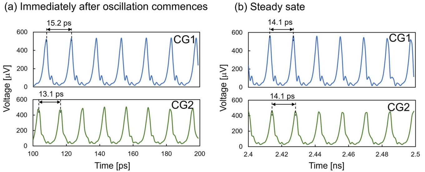
Figure 3. Transient analysis results for the frequency synchronization of CG1 and CG2.
