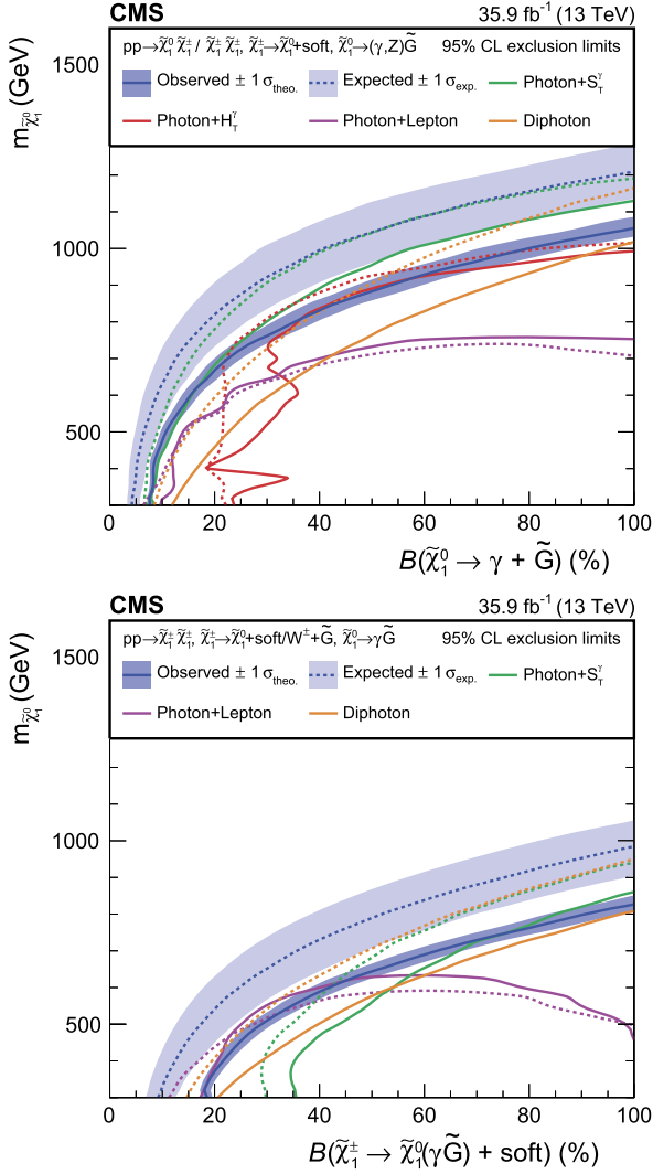
Fig. 5. The combined 95% CL NLSM mass exclusion limits for EW SMS production above 300 GeV. For the neutralino branching fraction scenario (upper), the limit is shown as a function of the branching fraction \tilde{\chi}_1^0 \rightarrow \gamma + \tilde{G} , the other decay channel being \tilde{\chi}_1^0 \rightarrow Z + \tilde{G} . For the chargino branching fraction scenario (lower), the limit is shown as a function of the branching fraction \tilde{\chi}_1^\pm \rightarrow \tilde{\chi}_1^0(\gamma\tilde{G}) + \text{soft} , the other decay channel being \tilde{\chi}_1^\pm \rightarrow W + \tilde{G} . The full lines represent the observed and the dashed lines the expected exclusion limits, where the phase space below the lines is excluded. The band around the expected limit of the combination indicates the region containing 68% of the distribution of limits expected under the background-only hypothesis. The band around the observed limit of the combination shows the spread in the observed limit from variation of the signal cross sections within their theoretical uncertainties.
