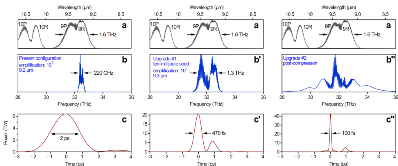
Figure 2. Simulations of short LWIR pulse amplification in the ATF laser system: (a) the normalized gain spectrum of the final amplifier; (b) the normalized spectrum of the pulse amplified from a 1 \mu\text{J} , 1 ps seed using the combination of a regenerative pre-amplifier and the final amplifier; (c) the temporal profile at the system's output for a 1 \mu\text{J} , 1 ps seed; (b') the normalized spectrum of the amplified pulse starting from a 10 mJ, 300 fs pulse seeded into the final amplifier; (c') the temporal profile at the system's output for a 10-mJ, 300-fs seed; (b'') the normalized spectrum of the post-compressed pulse; and (c'') the temporal profile of the post-compressed pulse [18].
