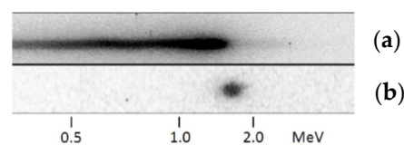
Figure 8. Comparison of (a) the TNSA proton spectrum with (b) the RPA proton spectrum obtained in ATF experiments with solid and gaseous targets, correspondingly.
