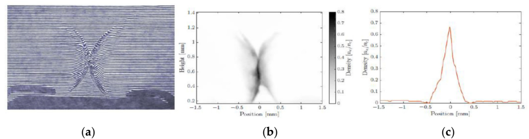
Figure 7. Interferometry of colliding blast waves (a,b), its plasma density reconstruction, and (c) its density profile taken at the 0.6 mm height over the nozzle edge [94].
