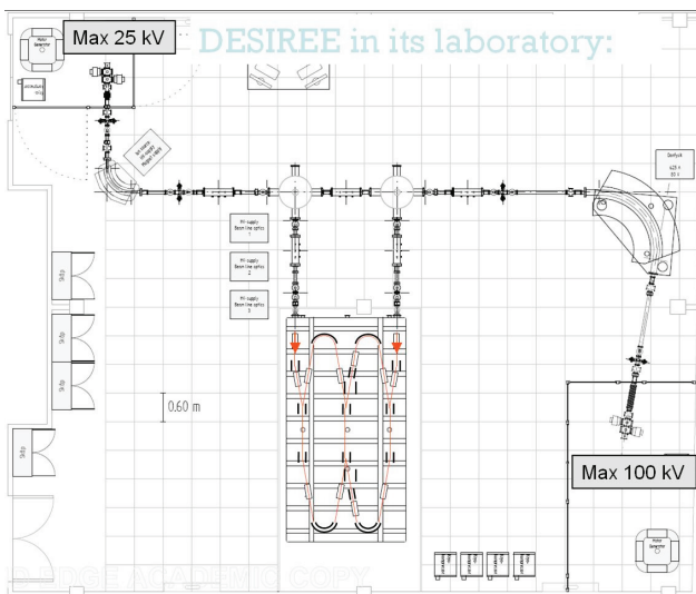
Figure 1: Layout of the DESIREE lab.
