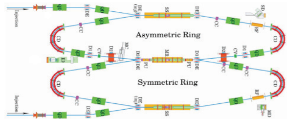
Figure 2: Drawing of the DESIREE optics.
