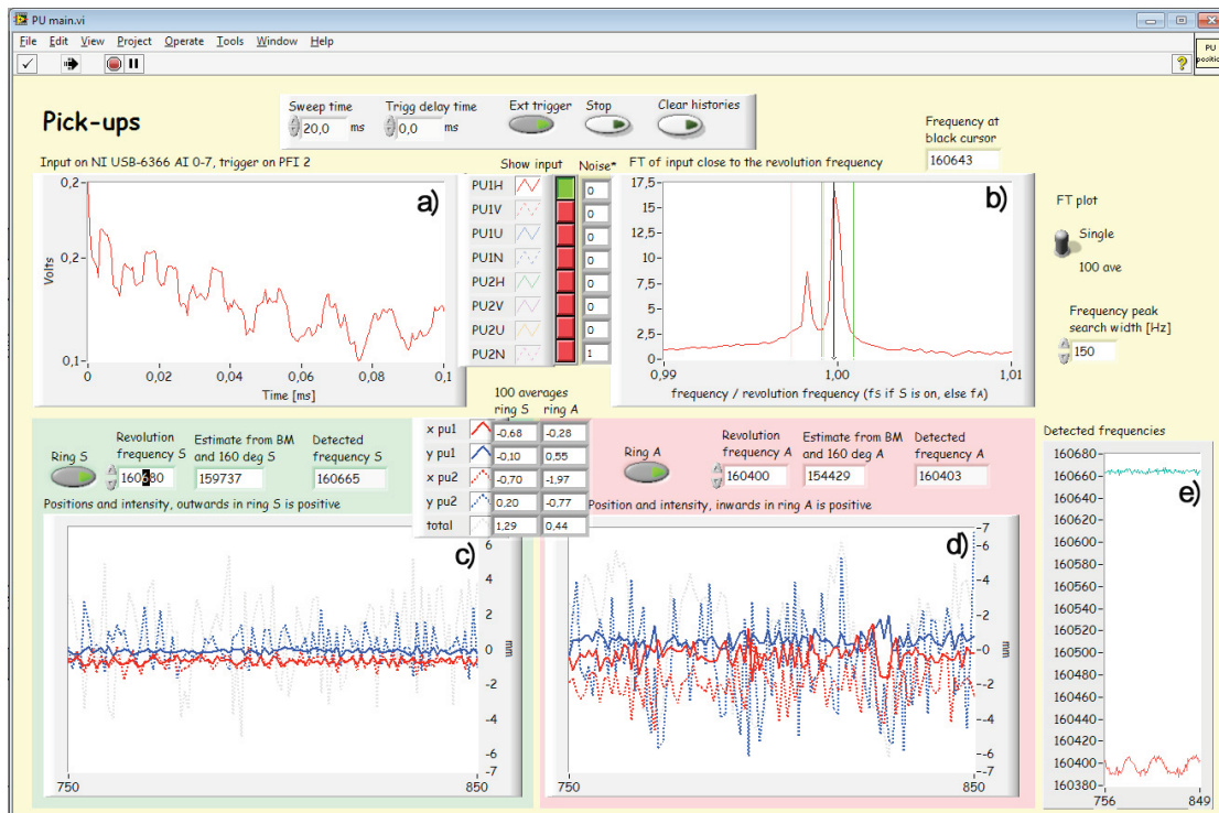
Figure 3: Screen dump from a PU measurement of 10 keV \text{H}^+ in ring A and 10 keV \text{H}^- in ring S. The graphs show:
