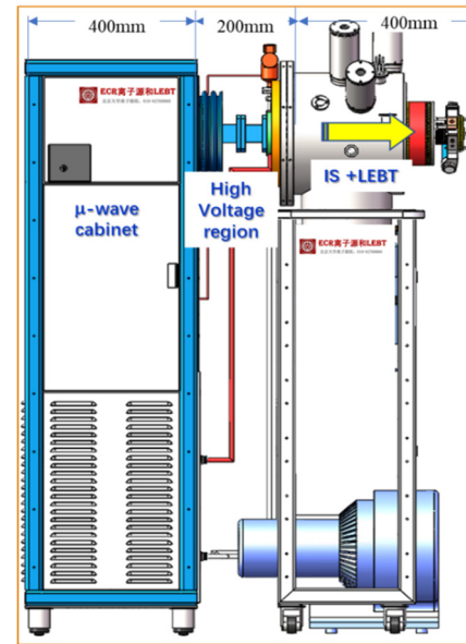
Figure 1: The mechanical view of the proton injector.
