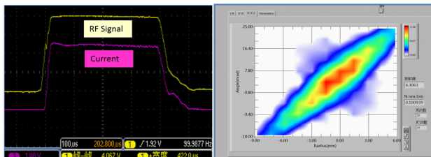
Figure 2: Result of this proton source when RF is 1600W. Beam current (up), Emittance (down).
