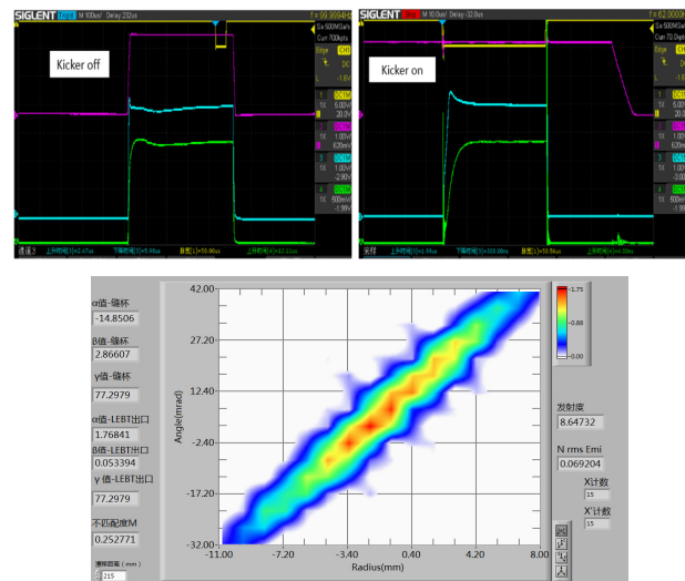
Figure 3: Beam current records with kicker off (up) and kicker on (middle) at ACCT and FC, and its emittance (down). Red: Microwave signal; Yellow: Signal of kicker; Blue: Current at ACCT; Green: Current at Faraday.
