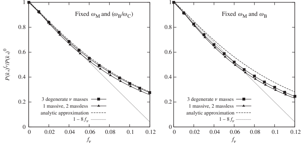
Figure 6.7 Suppression factor P(\eta, k)^{f_v}/P(\eta, k)^0 computed today for k = 10 h/\text{Mpc} , as a function of the total neutrino fraction f_v . The result depends on the mass splitting but is always contained between the two displayed curves corresponding to a single massive neutrino or three degenerate neutrinos, i.e., to the maximal and minimal values of the heaviest mass that can be involved for each value of f_v . We show for comparison the analytic approximation of Eq. (6.86) as well as the well-known linear approximation (1 - 8f_v) . On the left, the comparison was performed with fixed values of \omega_M and (\omega_B/\omega_C) , as explicitly assumed when deriving the analytical formula. On the right, we kept \omega_M and \omega_B fixed (with the increase in \omega_v compensated for by a decrease in \omega_C ), and we compare with the same approximations.
