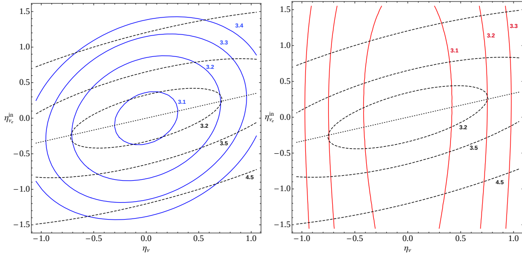
FIG. 1: Final contribution of neutrinos with primordial asymmetries to the radiation energy density. The isocontours of N_{\text{eff}} on the plane \eta_{\nu_e}^{\text{in}} vs. \eta_\nu , including flavor oscillations, are shown for two values of \sin^2 \theta_{13} : 0 (blue solid curves, left panel) and 0.04 (red solid curves, right panel) and compared to the case with zero mixing (dashed curves). The dotted line corresponds to \eta_\nu = \eta_{\nu_x} ( x = \mu, \tau ), where one expects oscillations to have negligible effects.
