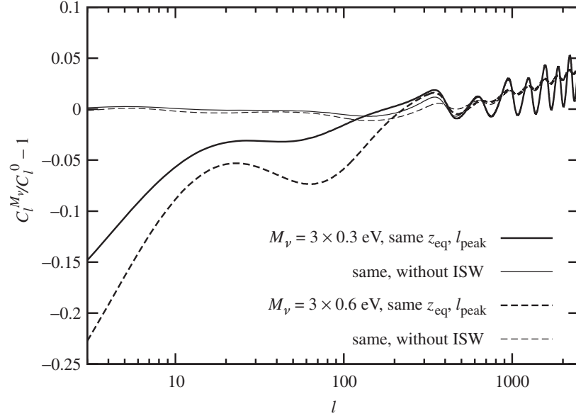
Figure 5.6 CMB temperature spectrum for models with either M_\nu = 3 \times 0.3 eV or M_\nu = 3 \times 0.6 eV divided by the spectrum of a model with three massless neutrinos sharing the same (standard) temperature. From left to right, the differences can be attributed to the LISW effect, EISW effect, gravitationally driven oscillations effect and diffusion damping, as explained in the text. To separate better the impact of the LISW plus EISW effect, the thin lines show the result of the comparison when the full ISW contribution is removed from each spectrum.
