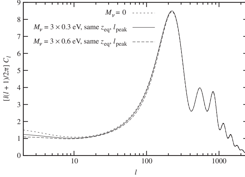
Figure 5.5 Spectrum of CMB temperature anisotropies for a massless neutrino model (highest curve for l \leq 100 ), a model with three degenerate neutrinos of total mass M_\nu = 3 \times 0.3 eV (middle curve for l \leq 100 ), and one with M_\nu = 3 \times 0.6 eV (lowest curve for l \leq 100 ). In all cases the redshift of equality between radiation and matter and the scale of the peaks has been kept constant.
