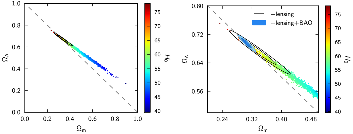
Fig. 25. The Planck +WP+highL data combination (samples; colour-coded by the value of H_0 ) partially breaks the geometric degeneracy between \Omega_m and \Omega_\Lambda due to the effect of lensing in the temperature power spectrum. These limits are significantly improved by the inclusion of the Planck lensing reconstruction (black contours). Combining also with BAO (right; solid blue contours) tightly constrains the geometry to be nearly flat.
