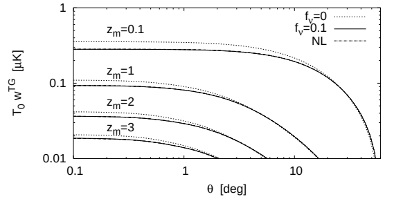
FIG. 4: Angular cross-correlation function, multiplied by the average CMB temperature and displayed in units of micro-Kelvins, for the same cosmological models as in Figs. 2,3. We also plot the same functions including non-linear (NL) corrections to the matter power spectrum: they are indistinguishable from the linear ones.
