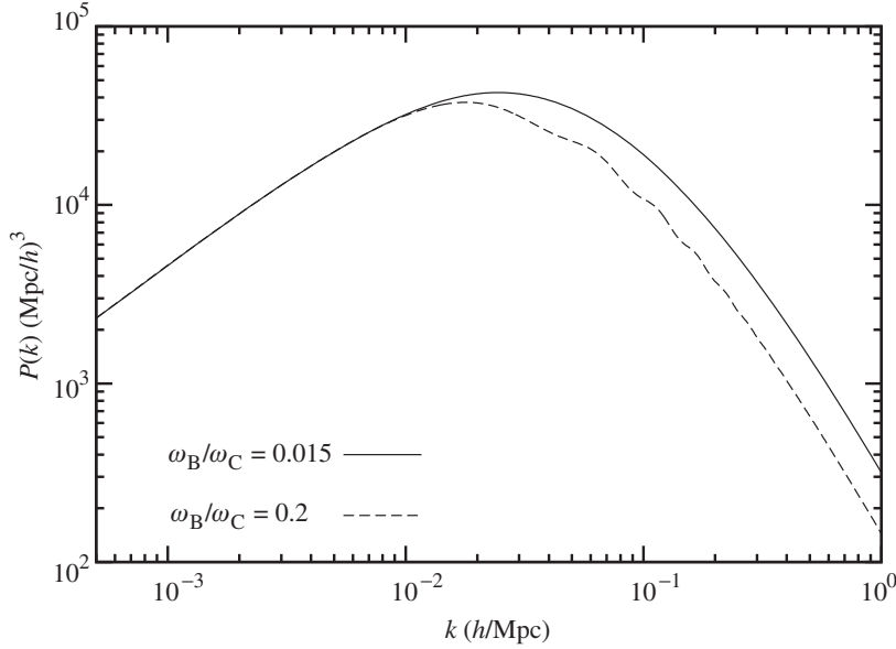
Figure 6.1 Matter power spectrum for two neutrinoless \Lambda CDM models with the same primordial spectrum and \Omega_M , but different baryon-to-CDM ratios \omega_B/\omega_C . The difference between the two curves clearly shows the baryon effects described in the text (suppression of power for k \geq k_{\text{eq}} and imprint of small acoustic oscillations).
