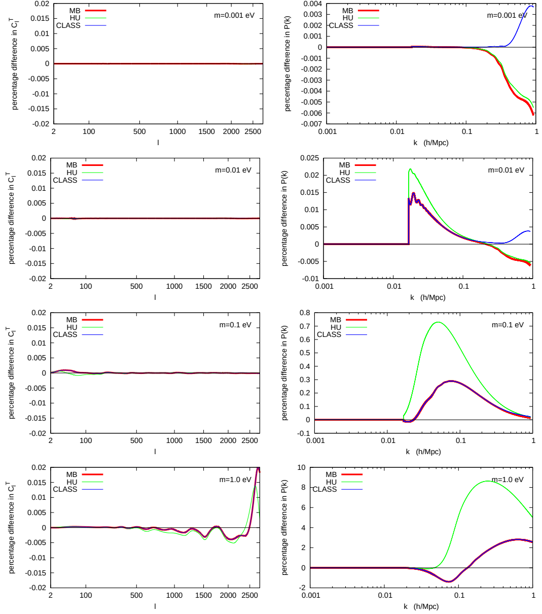
Figure 2: On the left, we have shown the percentage difference in the C_l^T for three degenerate neutrino species with mass m = 0.001\text{eV} , m = 0.01\text{eV} , m = 0.1\text{eV} and m = 1\text{eV} respectively, in runs with/without the fluid approximation. The fluid approximation works very well as long as the neutrinos are relativistic, so this is what we expect. On the right we have shown the matter power spectrum for the same masses. Here the agreement is not so good as the mass becomes higher.
