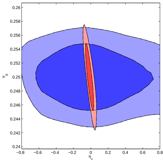
FIG. 3: 68% and 95% confidence regions in total neutrino asymmetry \eta_\nu vs. the primordial abundance of Helium Y_p plane for \theta_{13} = 0 (blue) and \sin^2 \theta_{13} = 0.04 (red), from the analysis of the WMAP+He dataset. Notice the much stronger constraint for the nonzero mixing angle due to the faster equilibration of flavor asymmetries.
