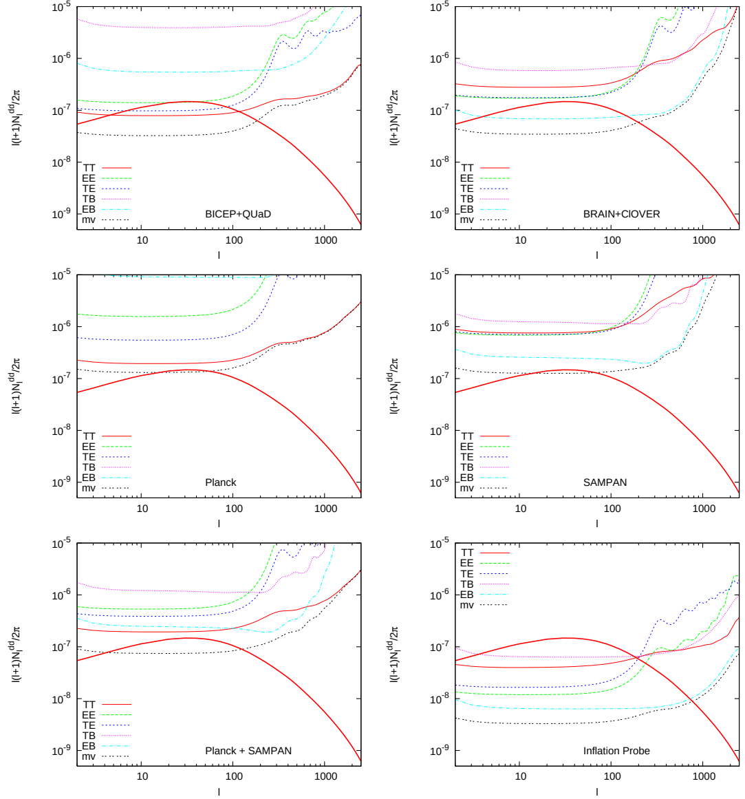
FIG. 1: For six CMB experiments or combinations of experiments, we show the expected noise power spectrum N_l^{dd} for the quadratic estimators d(a, b) built out of pairs ab \in \{TT, EE, TE, TB, EB\} , and for the combined minimum variance estimator (mv). The thick line shows for comparison the signal power spectrum C_l^{dd} = \langle d_l^m d_l^{m*} \rangle . The sum of the two curves N_l^{dd} + C_l^{dd} represents the expected variance of a single multipole d(a, b)_l^m .
