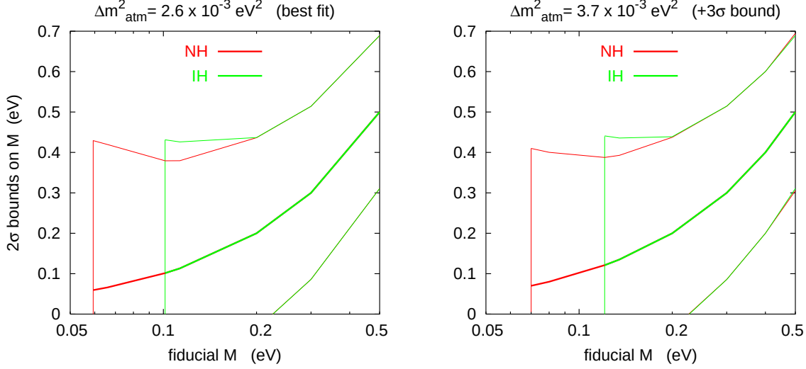
FIG. 5: Predicted 2\sigma error on the total neutrino mass M \equiv \sum m_\nu as a function of M in the fiducial model, using PLANCK and SDSS (limited to k_{\text{max}} = 0.15 h \text{ Mpc}^{-1} ). The left plot was obtained with the preferred experimental value of \Delta m_{\text{atm}}^2 , and the right plot with the current 3\sigma upper bound. In each case, we show the results assuming either NH or IH.
