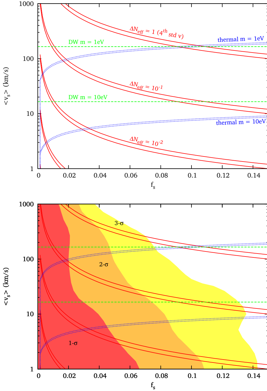
Figure 1: (Top) the parameter space (f_s, \langle v_s \rangle) chosen in our general analysis. The thin bands delimited by red/solid lines show regions of equal \Delta N_{\text{eff}} (assuming \omega_{\text{dm}} = 0.11 \pm 0.01 ); these bands are fully model-independent. We also show the model-dependent regions of equal mass, delimited by blue/dotted lines for the case of early decoupled thermal relics, and consisting in horizontal green/dashed lines for Dodelson-Widrow sterile neutrinos. (Bottom) same with, in addition, the regions allowed at the 68.3% ( 1\sigma ), 95.4% ( 2\sigma ) and 99.7% ( 3\sigma ) C.L. by our cosmological data set, in a Bayesian analysis with flat priors on f_s and \log_{10} \langle v_s \rangle within the displayed range.
