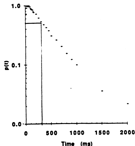
Figure 5 : The release delay curve for ^{19}\text{Ne} from a MgO target at 1000^\circ
