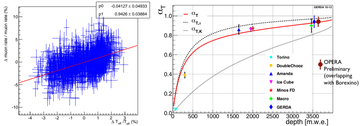
Figure 3. Left: correlation between the muon rate and effective temperature relative variations. Right: Effective temperature coefficient \alpha_T vs depth as measured by different underground experiments. The red line is the value predicted assuming muon production from pions and kaons; the dashed lines correspond to the single production mechanisms.
