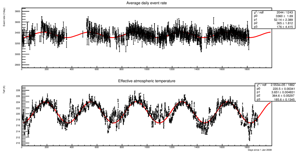
Figure 1. Single muon rate measured by the OPERA detector (top) and effective atmospheric temperature T_{eff} (bottom) from January 2008 to December 2012.
