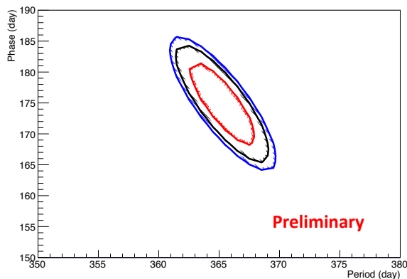
Figure 2. Preliminary 68% (red), 90% (black) and 95% (blue) C.L. allowed regions in the phase versus period parameter space for the atmospheric single muon flux.
