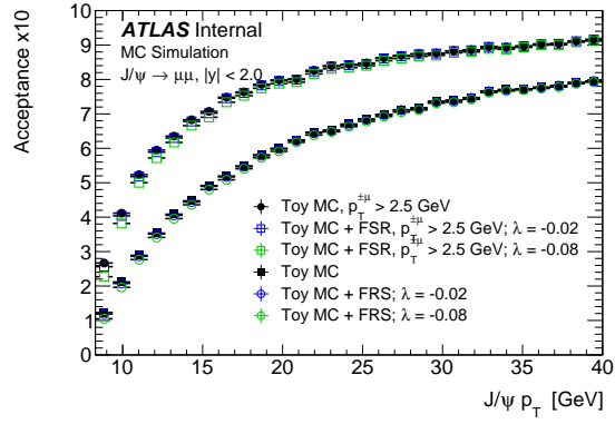
FIGURE F.3: J/\psi kinematic acceptance as a function of p_T . Calculated with and without a cut in the daughters muons and with and without FSR emulation.
