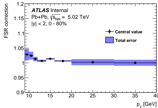
FIGURE 6.13: The derived FSR correction factor for charmium candidates.
