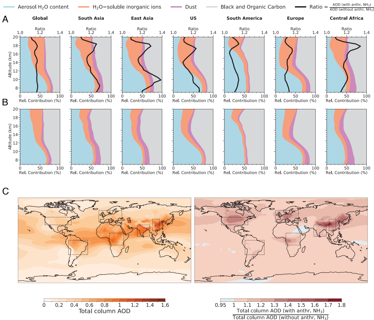
Fig. 3. Vertical distribution of the contribution of different UTLS AOD components to the total AOD over \text{NH}_3 emission hotspots (A) with and (B) without anthropogenic \text{NH}_3 . The relative contributions of aerosol components ( \text{H}_2\text{O} , \text{H}_2\text{O} -soluble inorganic ions, dust, black and organic carbon) to the total AOD (550 nm) are shown as stacked colored regions. The black line represents the ratio of AOD with anthropogenic \text{NH}_3 to AOD without, highlighting the relative enhancement due to \text{NH}_3 emissions at each altitude. The tropopause altitude range for each region is specified in Fig. 1A. (C) Total atmospheric column AOD at 550 nm in the presence of anthropogenic \text{NH}_3 (Left). AOD total column enhancement ratio is defined as the ratio of total column AOD with anthropogenic \text{NH}_3 to without (Right). Values greater than 1 indicate an increase in AOD due to \text{NH}_3 (in red), while values below 1 indicate a decrease (in blue). \text{NH}_3 emission hotspots are marked on the map. The results are calculated at ambient conditions and averaged over the entire period from 2003 to 2019.
