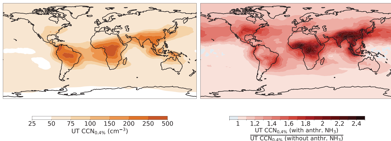
Fig. 4. Global maps of cloud condensation nuclei concentrations at 0.4% supersaturation ( CCN_{0.4\%} ) in the UT, averaged within the 10 to 13 km altitude range. The Left panel illustrates the absolute UT CCN_{0.4\%} values in the presence of anthropogenic NH_3 . The Right panel shows the enhancement ratio, defined as the ratio of UT CCN_{0.4\%} values with anthropogenic NH_3 to those without. Values greater than 1 indicate an increase due to NH_3 (in red), while values below 1 indicate a reduction (in blue). The results are calculated at ambient conditions and averaged over the entire period from 2003 to 2019.
