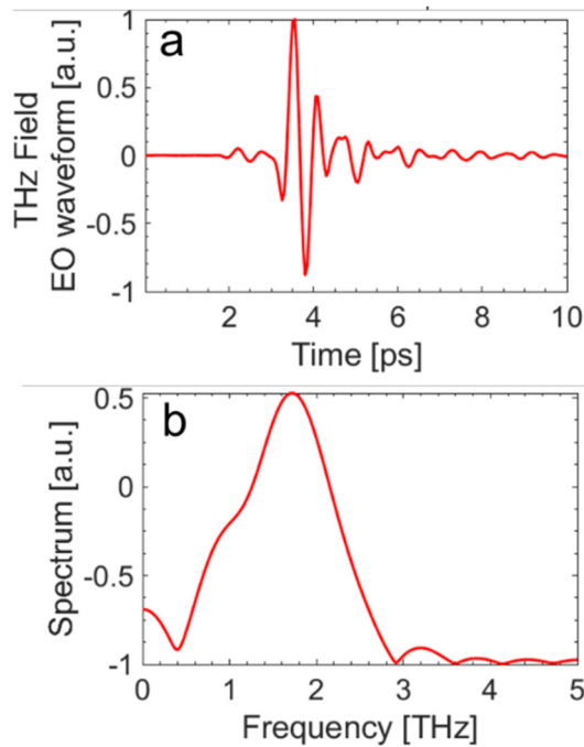
Figure 2: Measured EOS trace of the electric field inside the THz compressor, only from one THz pulse.
