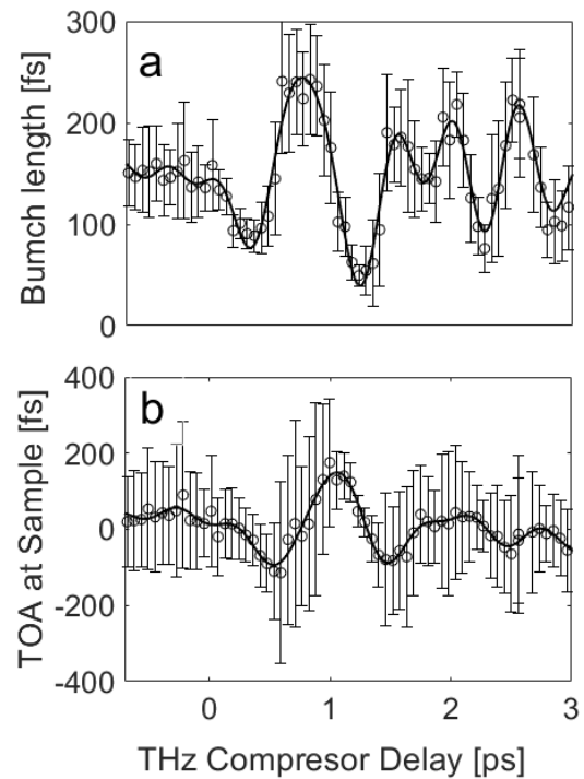
Figure 3: Single shot delay scan of the bunch length and time of arrival at the sample; measured using THz streaking, and showing a minimum bunch length \sim 40 fs and jitter suppression at around 1.3 ps.
