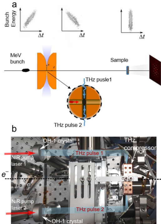
Figure 1: (a) Layout of the dual fed THz compressor and (b) photo of the setup inside the MeV-UED beamline.
