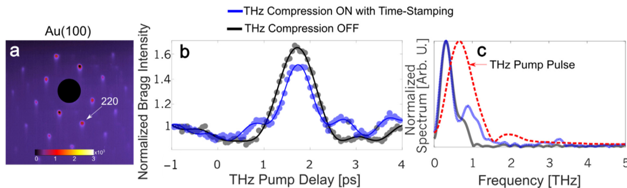
Figure 4: Temporal resolution of the THz time-stamped electron probes using a single crystal Au sample. (a) Diffraction pattern a single crystal Au(100) probed by a time-stamped electron probe taken before the arrival of the THz pump acquired from averaging 20 single shots. (b) Intensity of a Bragg peak (220), for THz compression and time-stamping and without, and (c) the corresponding frequency spectrum of the Bragg peak variations as well as the pump THz pulse in free space.
