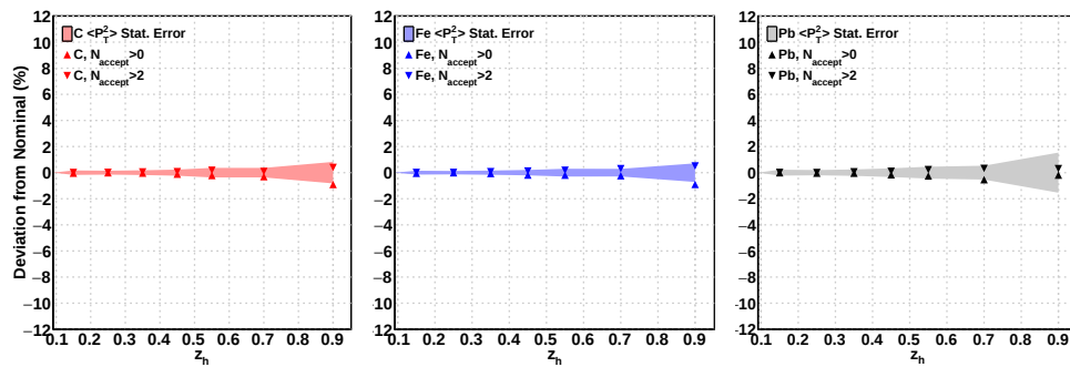
Figure B.22: N_{accept} cut systematic uncertainty's \langle P_T^2 \rangle , with x_f > 0 , deviations from the nominal values for solid targets
