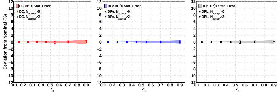
Figure B.19: N_{accept} cut systematic uncertainty's \langle P_T^2 \rangle deviations from the nominal values for liquid targets
