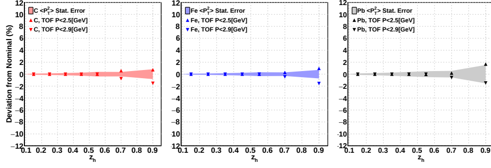
Figure B.3: TOF systematic uncertainty's \langle P_T^2 \rangle deviations from the nominal values for solid targets
