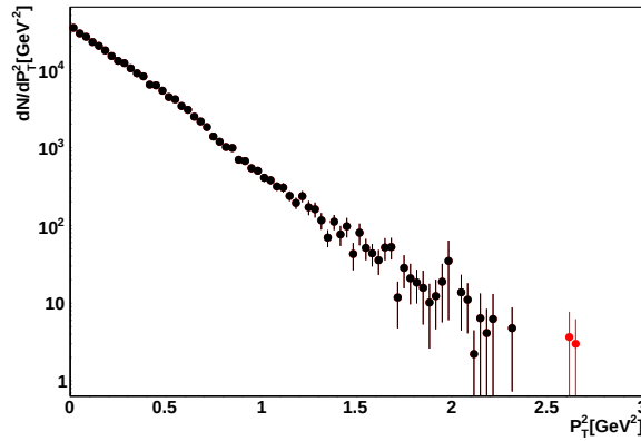
Figure 3.21: P_T^2 distribution for Fe target and within 1.3 < Q^2 [\text{GeV}^2] < 1.8 , 2.2 < \nu [\text{GeV}] < 3.2 , 0.6 < z_h < 0.8 . The red points indicates which bins were considered as scattered points.
