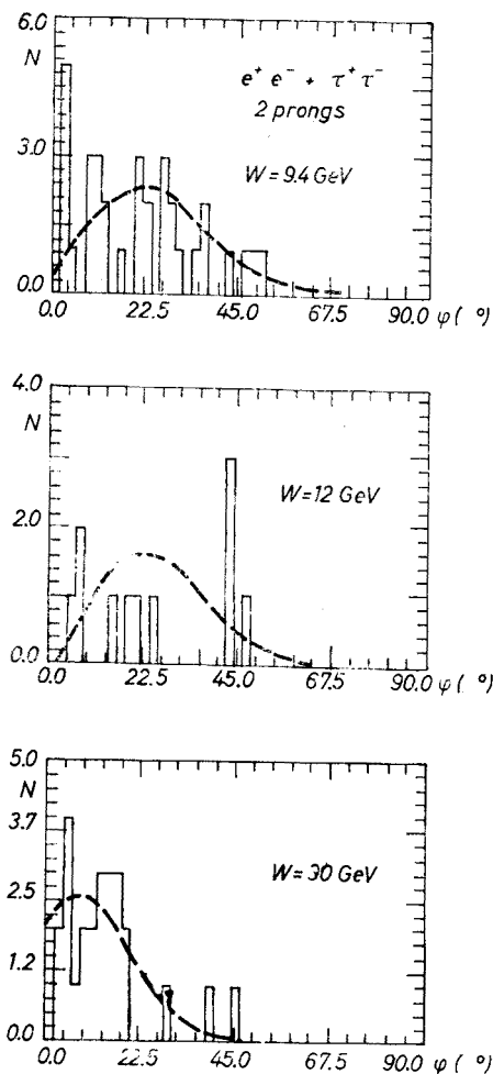
Fig. 13. Acollinearity angle distribution in e^+e^- \rightarrow \tau^+\tau^- 2 prong events, at W = 9.4, 12 , and 30 GeV
