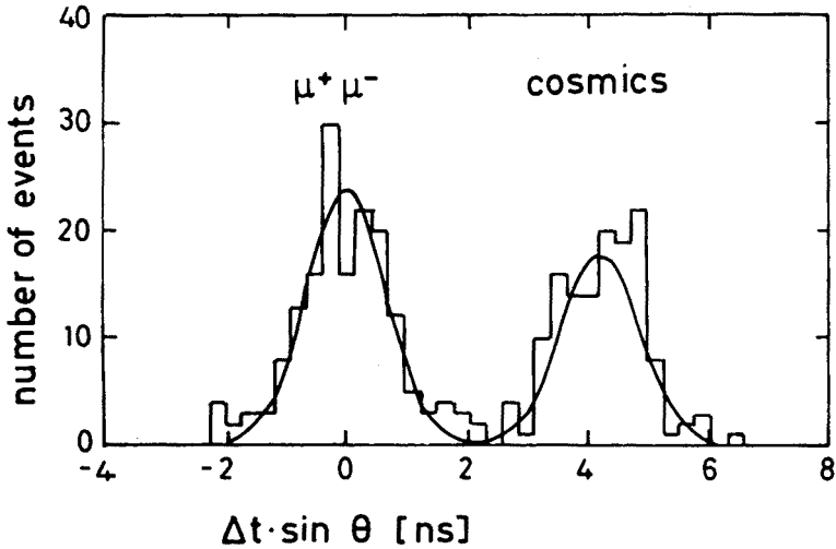
Fig. 12. TOF difference for \mu pairs and cosmics
