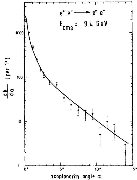
Fig. 5. Distribution of the acoplanarity angle \alpha from the Bhabha event sample, at W = 9.4 \text{ GeV}
