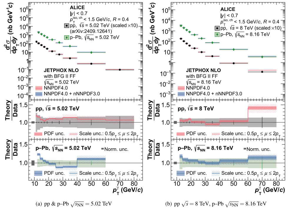
Fig. 4 Isolated prompt photon inclusive production cross section in pp collisions at \sqrt{s} = 5.02 [22] and 8 TeV, and p–Pb collisions at \sqrt{s_{NN}} = 5.02 and 8.16 TeV. Vertical bars and boxes denote statistical and systematic uncertainties, respectively. Coloured lines denote JETPHOX pQCD calculations at NLO using the recent NNPDF4.0 [49] proton PDF and the nNNPDF3.0 [50] nuclear PDF. The BFG II [51] fragmentation function is used to describe parton-to-photon fragmentation. Dashed coloured bands denote the theoretical scale uncertainties, and solid bands denote PDF uncertainties at 90% CL
