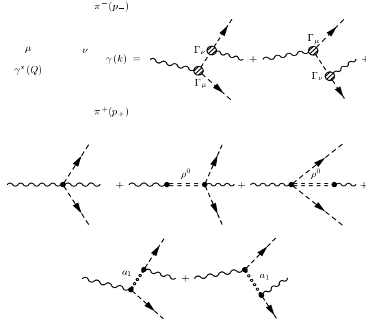
Figure 1: Diagrams for FSR in the framework of ChPT.
