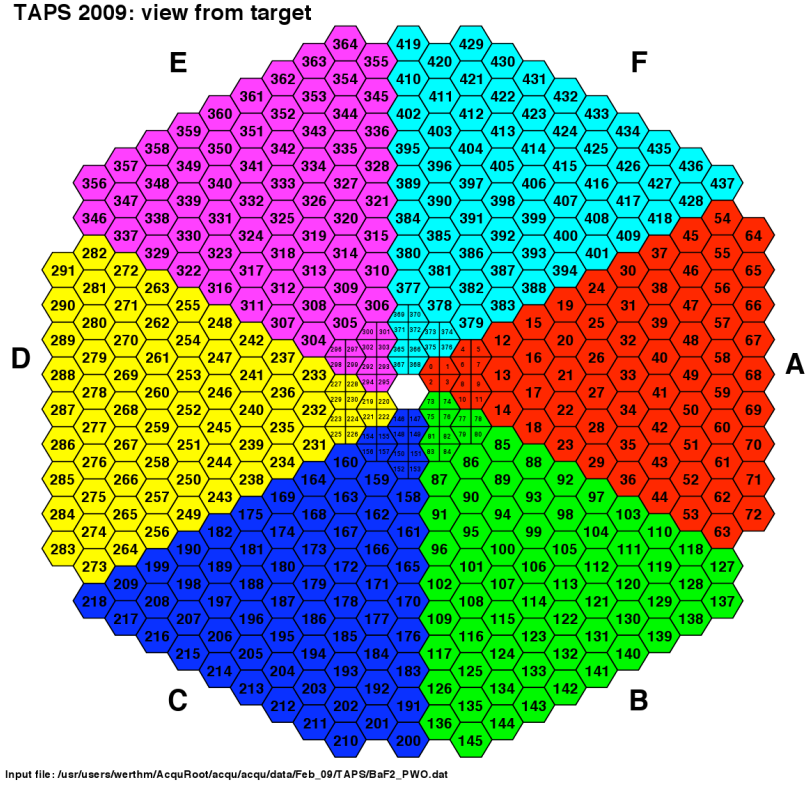
Figure 5.10 Schematic of the TAPS crystal arrangement at MAMI, the smaller inner crystals are the \text{PbWO}_4 crystals [124].
