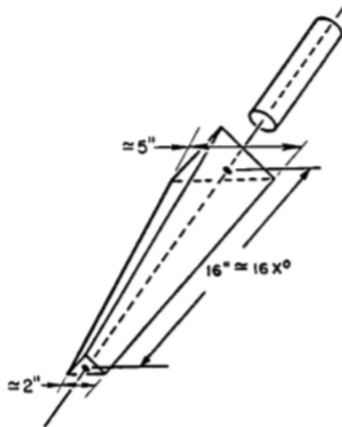
Figure 5.9 Illustration of an individual NaI(Tl) crystal used in the Crystal Ball with dimensions in inches [5].
