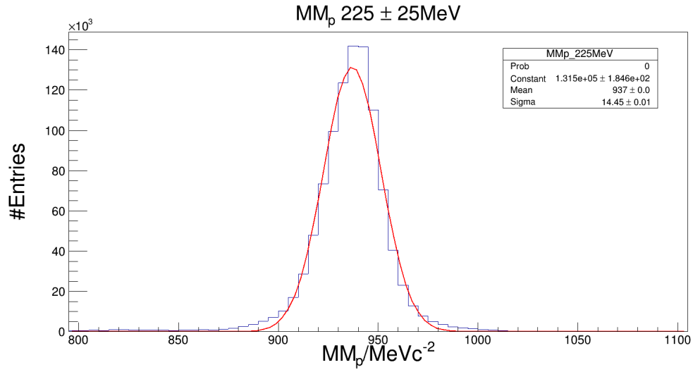
Figure 8.7 The missing mass calculated from the proton track vector, MM_p , for E_\gamma = 225 \pm 25 MeV with a Gaussian fit applied to the peak.
