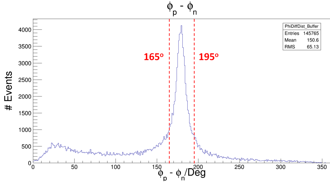
Figure 8.4 Distribution of \Delta\phi between the proton and neutron tracks with the (180 \pm 15)^\circ cut region illustrated. A small peak between 0-50^\circ can be observed in the plot, this is likely due to the contribution of background reactions where more than two particles have been produced.
