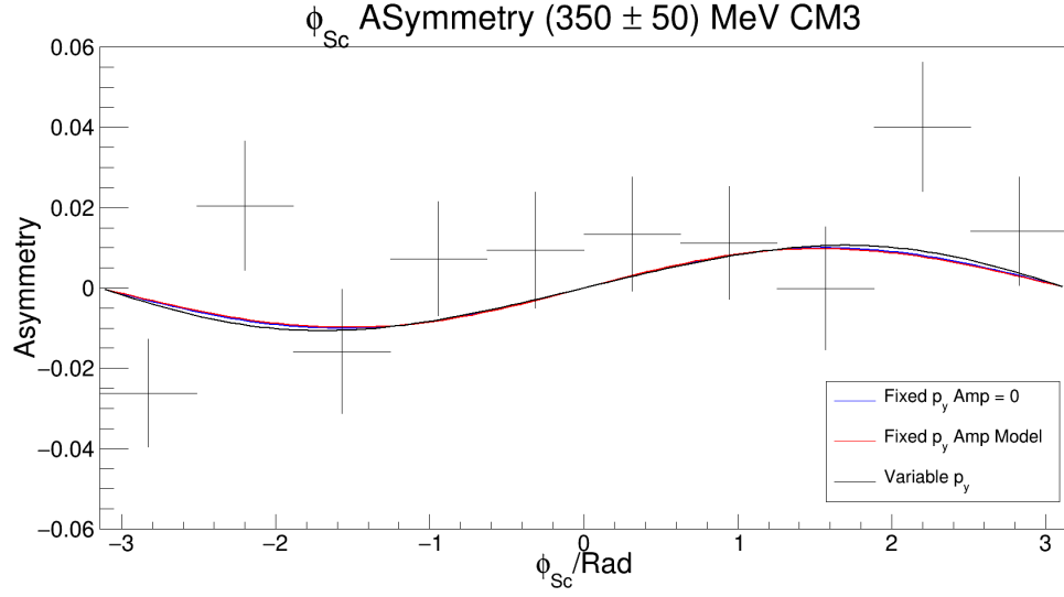
Figure 8.21 Asymmetry in \phi_{\text{Sc}} between the two photon beam helicities for scattered neutrons in one 100 MeV wide E_\gamma bin. Demonstrated on the plot are three fits to the data with differing values for the second parameter (that relates to p_y ) either fixed or limited respectively.
