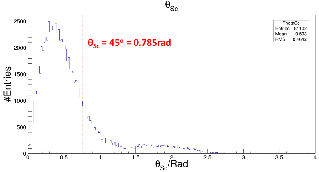
Figure 8.16 \theta_{\text{Sc}} distribution of scattered neutrons with the 45^\circ ( \frac{\pi}{4} rad) cut point marked.
