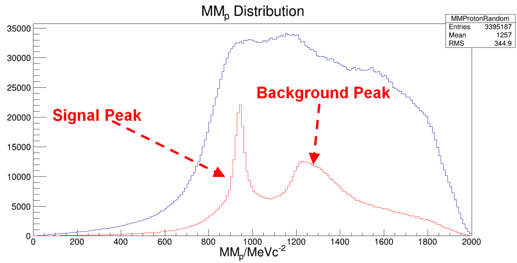
Figure 8.2 An example missing mass distribution for prompt (red) and random (blue) photons. As discussed in Section 8.1.2, events of interest should show a peak at MM_p \approx 940 MeV. This peak and a peak at higher missing mass (background contribution) can clearly be seen in the prompt spectrum. Random events are smeared over a range of missing mass values.
