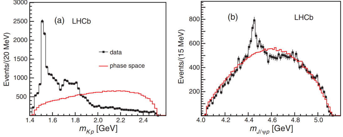
Figure 4.4 Background subtracted invariant mass distributions for K^-p (left, (a)) and J/\psi p (right, (b)) combinations from \Lambda_b^0 \rightarrow J/\psi K^- p decays [58]. The red curve shows expectations from phase space. A clear peak is observed in the distributions for J/\psi p .
