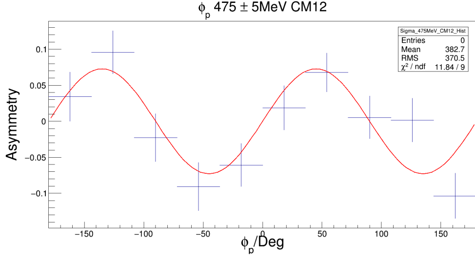
Figure 9.1 Example fit of P_0(\cos(2\phi + \frac{\pi}{2})) to the asymmetry between N^\parallel(\phi_p) and N^\perp(\phi_p) for the extraction of \Sigma . This is one 10 MeV wide bin in E_\gamma for \cos\theta_{\text{CM}} = -0.2 - -0.3 . Fit parameters are included in the top right.
