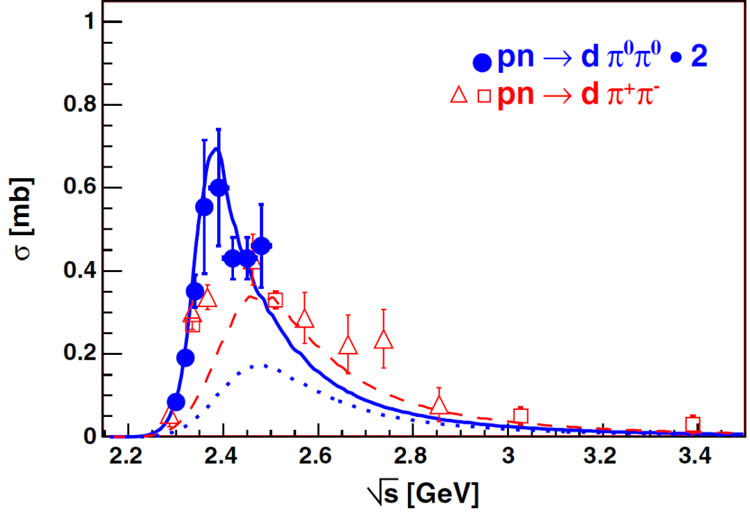
Figure 4.6 A plot of the energy dependence of the cross section for the reactions pn \rightarrow d\pi^+\pi^- and pn \rightarrow d\pi^0\pi^0 showing hints of an enhancement at around \sqrt{s} = 2.4 GeV [51].
