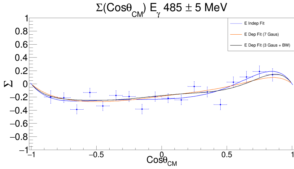
Figure G.2 \Sigma(\cos\theta_{\text{CM}}) in one 10 MeV wide E_{\gamma} bin. Demonstrated on the plot are three fits, the original energy independent and two further fits. The parameters for these fits were set based upon energy dependent fits (using three Gaussians and a Breit-Wigner or seven Gaussians) to the parameters P_{2-7}^2 as a function of E_{\gamma} .
