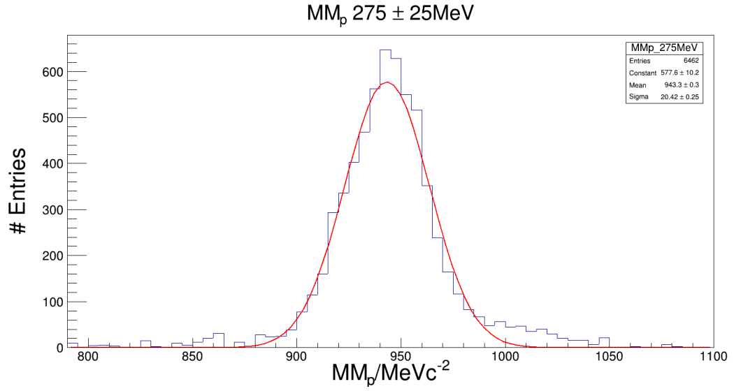
Figure 8.12 The missing mass calculated from the proton track vector, MM_p , for E_\gamma = 275 \pm 25 MeV with a Gaussian fit applied to the peak.
