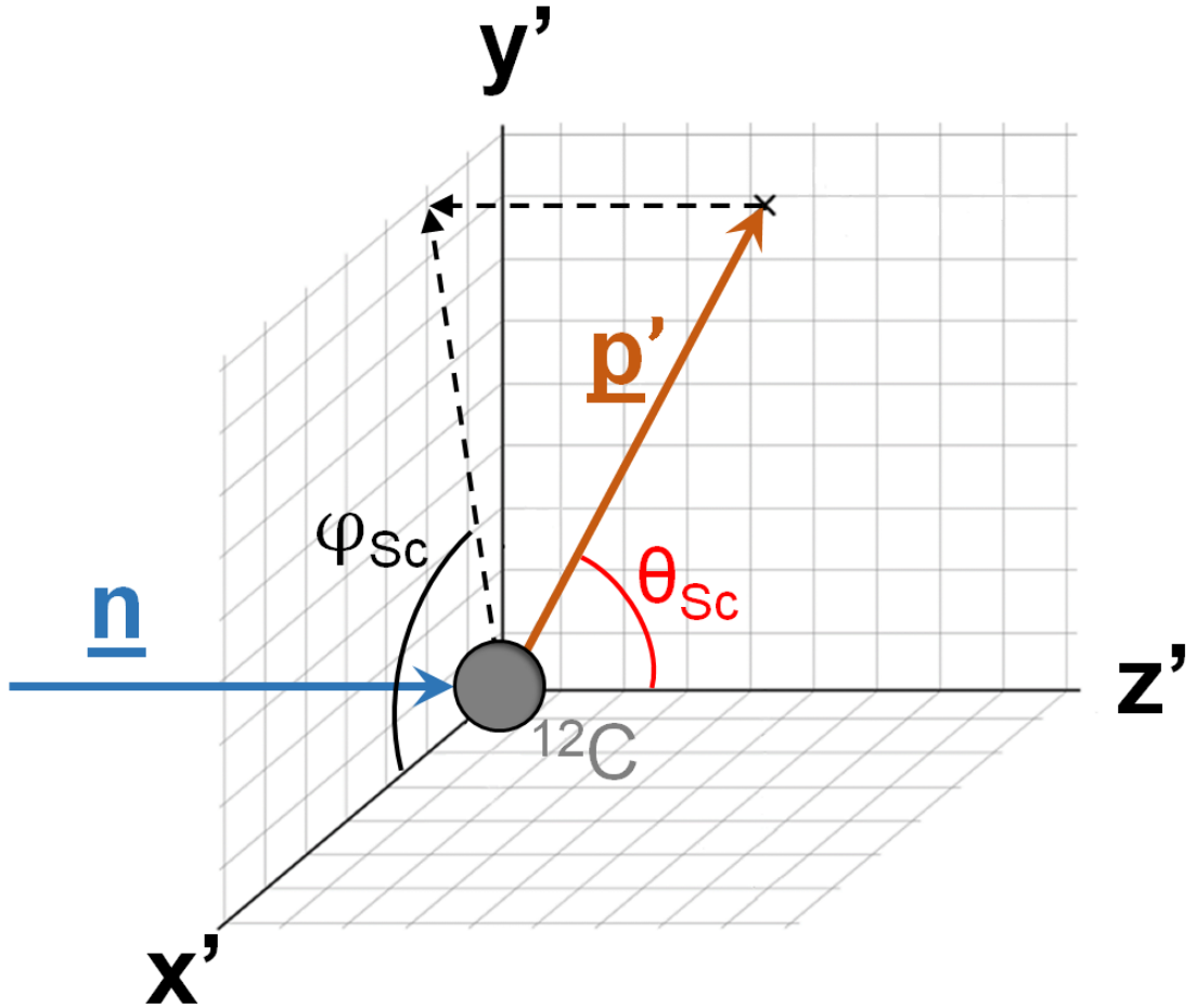
Figure 3.2 Neutron, n , undergoing a charge exchange interaction with a carbon nucleus in the (x', y', z') frame as defined by Equations (3.1–3.3). The angles \theta_{\text{Sc}} and \phi_{\text{Sc}} for the recoiling proton, p' , are shown (modified version of [28]).
