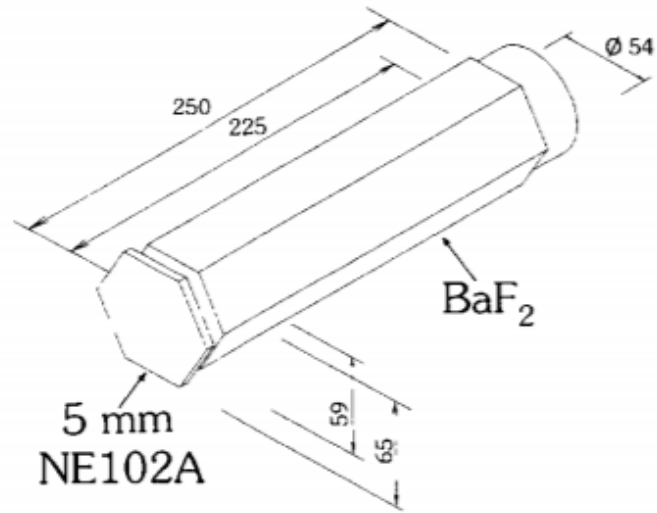
Figure 5.11 Diagram of individual TAPS \text{BaF}_2 crystal with VETO [7].
