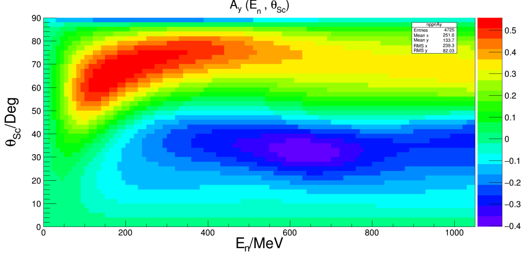
Figure 3.3 A_y for the elastic scattering reaction np \rightarrow pn as a function of \theta_{Sc} and E_n . A colour scale for the value of A_y is included.
