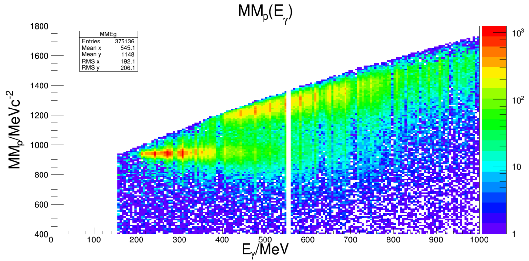
Figure 8.8 The missing mass calculated from the proton track vector as a function of the incident photon energy, E_\gamma . The \sim 940 MeV signal peak broadens as E_\gamma increases. A background peak begins to appear at E_\gamma \sim 350 MeV. Note that the z-axis of this figure is in a logarithmic scale.
