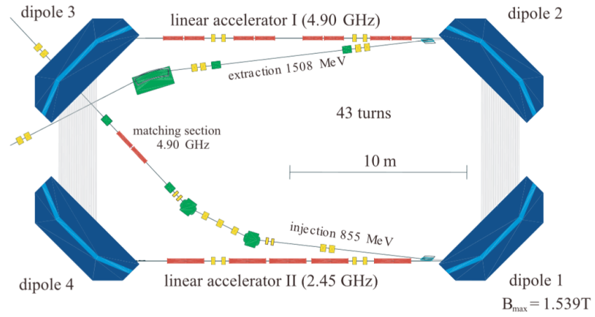
Figure 5.3 Schematic of the MAMI-C harmonic double sided microtron, the four 90^\circ dipole magnets are shown in blue [107].
