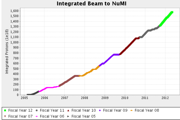
Figure 5: Integral protons to the NuMI target since the beginning of the program.
