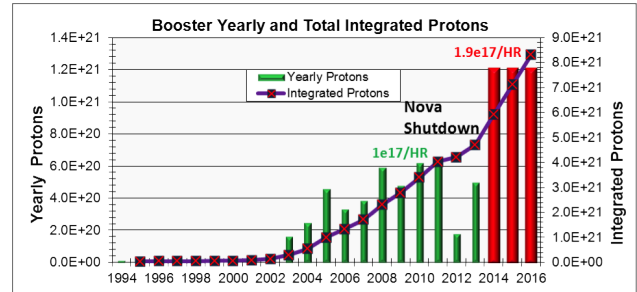
Figure 3: Historical Booster performance in protons/year and total integrated protons.
