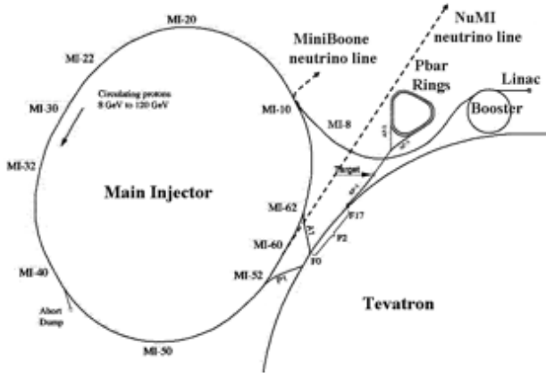
Figure 2: Layout of Fermilab Accelerator Complex.
