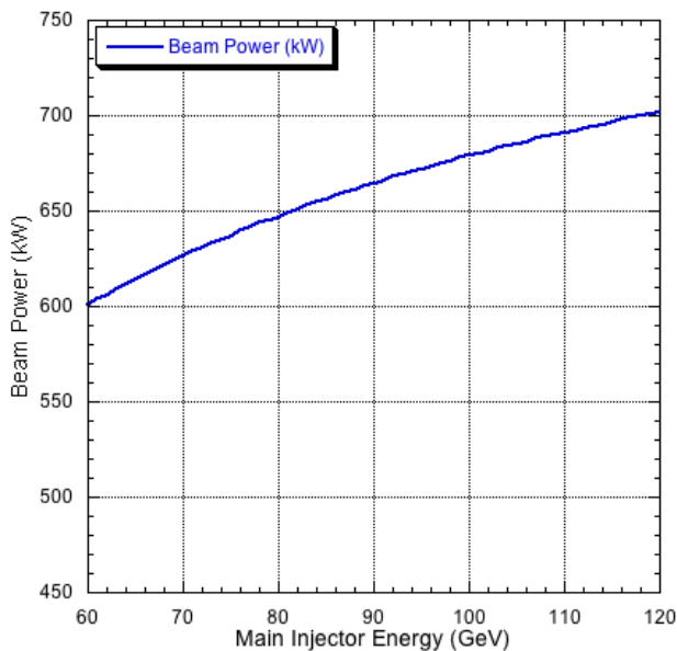
Figure 6: Beam power on target as a function of Main Injector flattop energy. It falls as the energy decreases due to the fixed time elements in the ramp.
