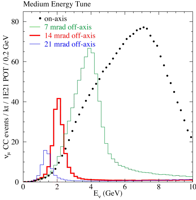
Figure 4: Muon neutrino charged current energy spectrum for the planned target hall configuration.
