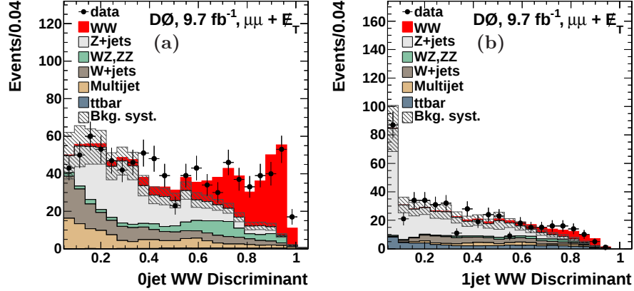
FIG. 21: The WW discriminant distributions in the \mu\mu channel for (a) no jet and (b) one jet.
