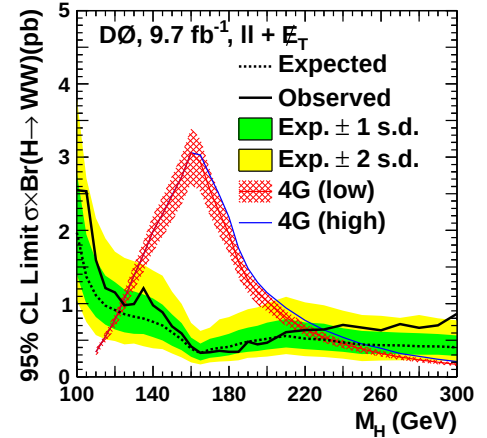
FIG. 4: [color online] Excluded cross section \sigma(gg \rightarrow H) \times \text{Br}(H \rightarrow WW) in pb as a function of M_H using all channels. The red and blue lines correspond to the theoretical prediction for a sequential fourth generation assumption in the “low mass” and “high mass” scenarios, respectively (see main text). The hatched region corresponds to the PDF and scale uncertainties on the fourth generation “low mass” prediction [50]. The green and yellow shaded bands indicate \pm 1 and \pm 2 s.d. uncertainties of the background-only hypothesis, respectively.
