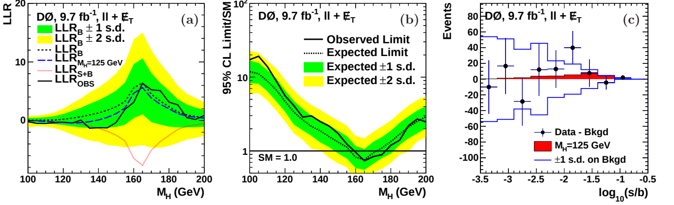
FIG. 3: [color online] (a) The observed LLR as a function of M_H . Also shown are the expected LLRs for the background-only hypothesis, for the signal+background hypothesis, and the expectation in the presence of a signal of M_H = 125 GeV. (b) Excluded cross section, \sigma(p\bar{p} \rightarrow H + X) , at the 95% C.L. in units of the SM cross section as a function of M_H . In (a) and (b), the green and yellow shaded bands indicate \pm 1 and \pm 2 s.d. uncertainties of the expected observation for the background-only hypothesis, respectively. (c) Background-subtracted data distribution for the final discriminants, summed in bins with similar signal to background ratios, for M_H = 125 GeV. The uncertainties shown on the background-subtracted data points are the square roots of the post-fit background predictions of number of events in each bin, representing the expected statistical uncertainty on the data points. Also shown is the \pm 1 s.d. band on the total background after fitting.
