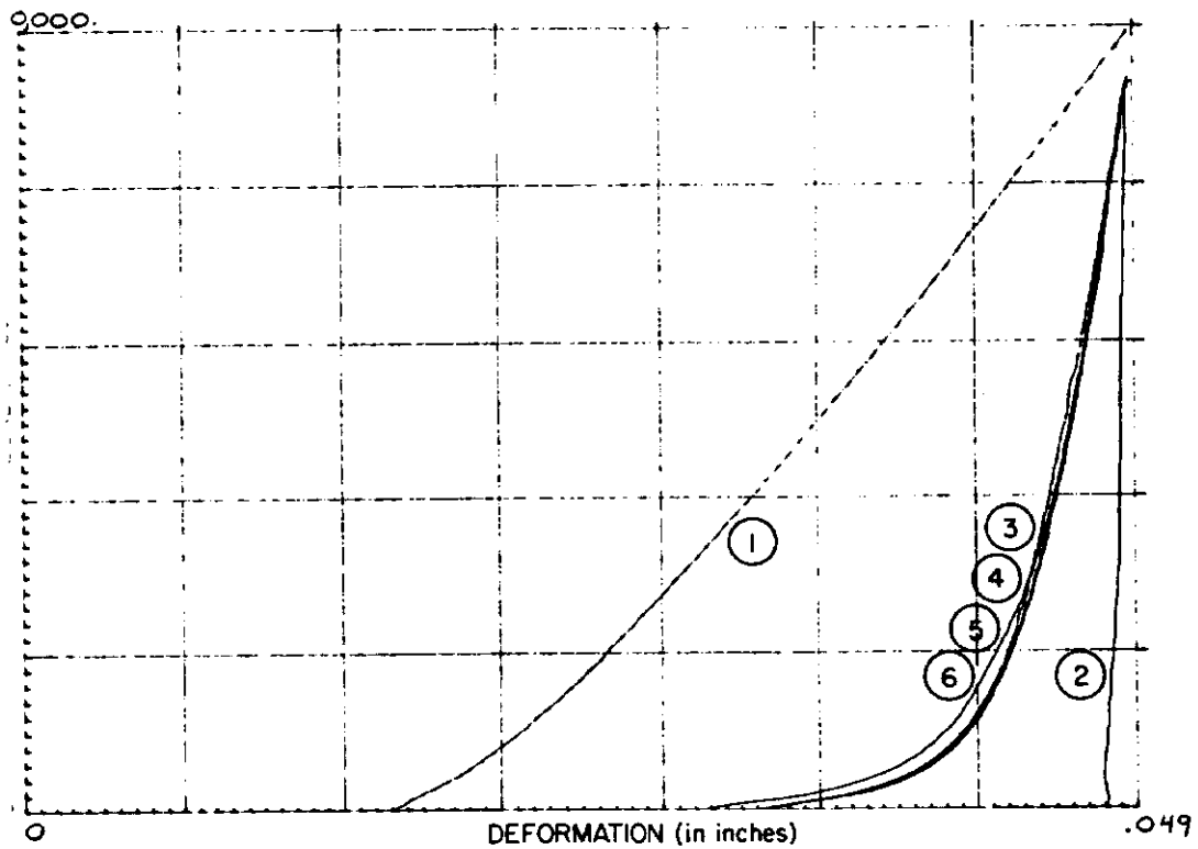
Figure 6. Azimuthal Data Normalized to 10,000 lbs.
