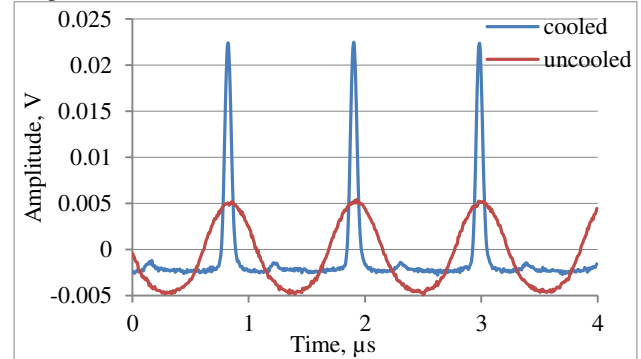
Figure 4: Proton bunch shortening during electron cooling with 200 mA. Shown are the bunch shapes for the cooled and uncooled proton beam as reported by the bunch phase monitor [8].
