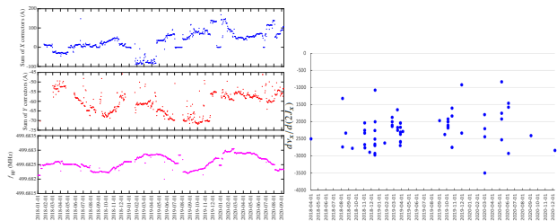
Figure 1: a) (Left) Measured seasonal variations of the RF frequency and of the sum strength of orbit correctors. b) (Right) dv_x/d(2J_x) coefficient measured in 2018-2020.
