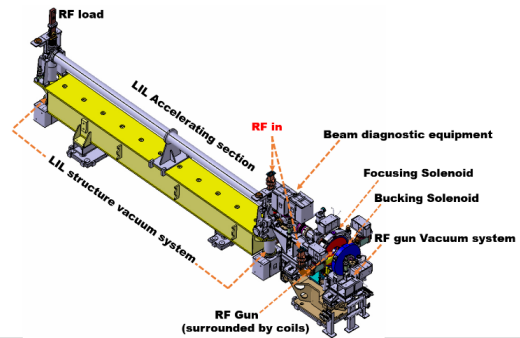
Figure 1: 3D scheme of the ThomX linear accelerator injector.
