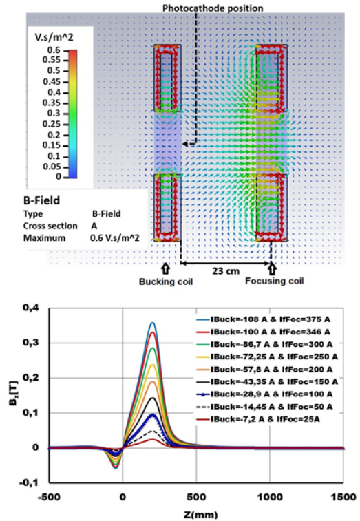
Figure 3: Model of the solenoids surrounding the ThomX gun cavity (cutting plane) with magnetic field distribution (top). Magnetic field strength on the axis for different pairs of currents in the two solenoids (bottom) using CST Studio Suite®.
