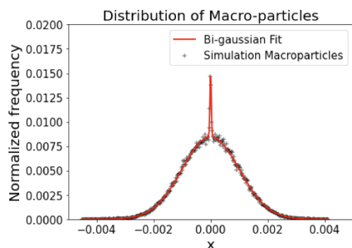
Figure 4: A Bi-Gaussian distribution of macro-particles in JSPEC, together with the fit performed to extract the core and tail amplitudes and standard deviations.
