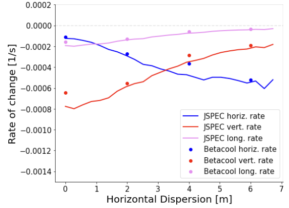
Figure 3: Comparison of JSPEC and Betacool for scans of horizontal dispersion and its effect on cooling rates.
