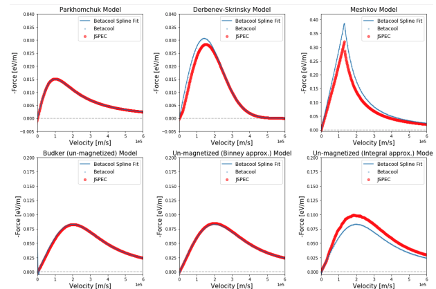
Figure 1: Comparison of friction force calculations in Beta-cool and in JSPEC.
