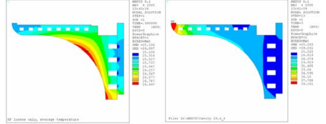
Figure 4: ANSYS thermal model with average RF losses (left) and thermal model with average RF and particle losses (right).
