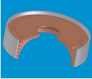
Figure 3: Cutaway view of proposed half cavity.
