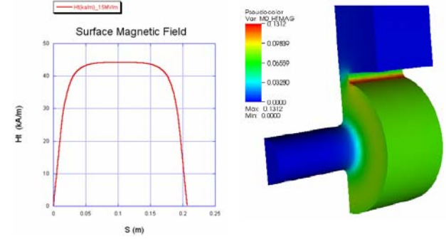
Figure 7: RF pulse heating calculations.
