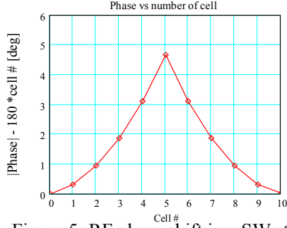
Figure 5: RF phase shift in a SW structure.
