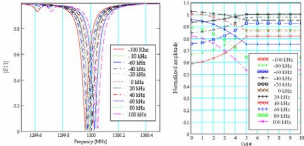
Figure 6: Frequency spectrum (left) and electrical field amplitude (right) for various frequency changes.
