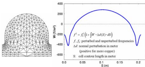
Figure 1: Cell profile of 1.27 m long \pi mode SW structure and the frequency perturbation weighting function along cell surface.
