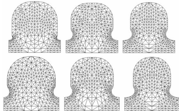
Figure 2: Profiles of the first, middle and last cell for 2.2m 5\pi/6 Mode TW structure (top row) and 4.3m 3\pi/4 Mode TW structure (bottom row).
