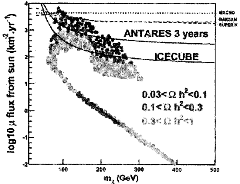
Fig. 4. Sensitivity limits reached by the present indirect detection experiments (from ref. 49). The ANTARES 0.1 km 2 detector will improve the present SuperKamiokande sensitivity by a factor 3, ICECUBE by a factor \approx 10 . Present sensitivities of direct and indirect detection experiments are comparable, with EDELWEISS being a factor 2 more sensitive than the current SuperKamiokande result.
