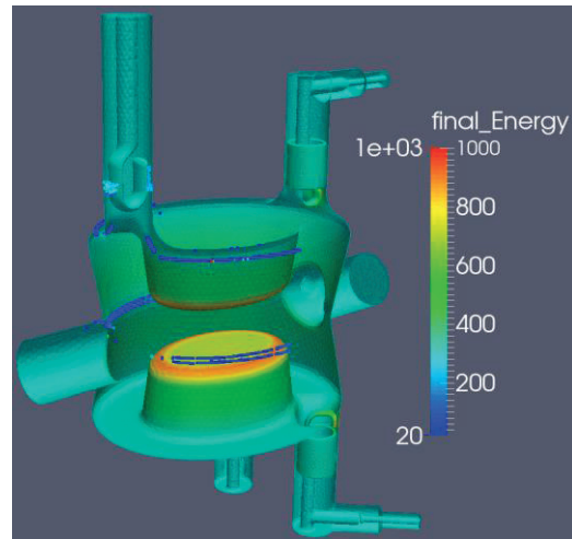
Figure 3: Multipacting sites in SPS DQWCC.
