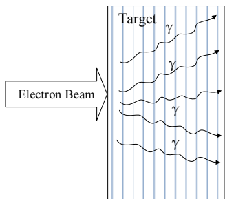
Figure 1: Schematic diagram of response of electron beam to heavy target
