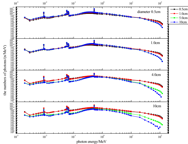
Figure 4: X-ray photon energy spectrum produced by electrons in Ta targets.
