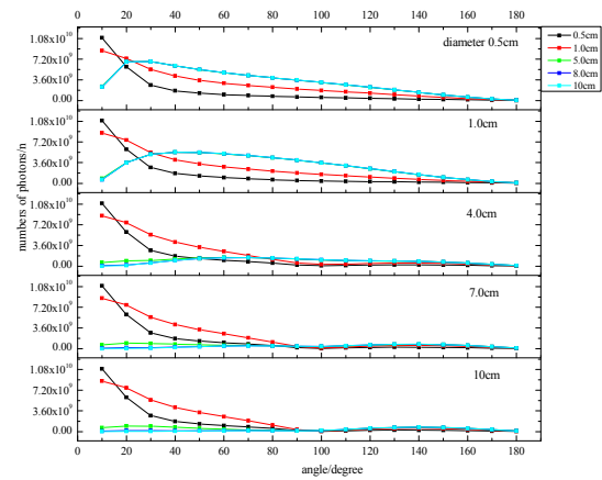
Figure 6: Photon angle spectrum produced in Ta targets with different diameters and thicknesses.
