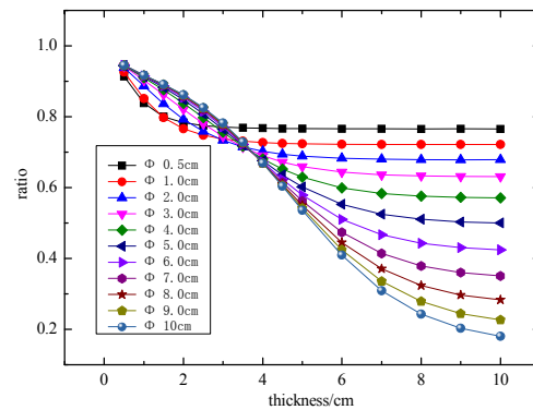
Figure 7: Proportion of photon numbers in the direction of 0-90 degree.
