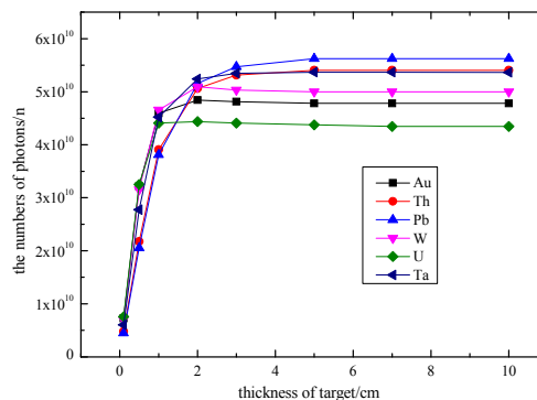
Figure 2: Calculation results of X-ray in heavy targets.
