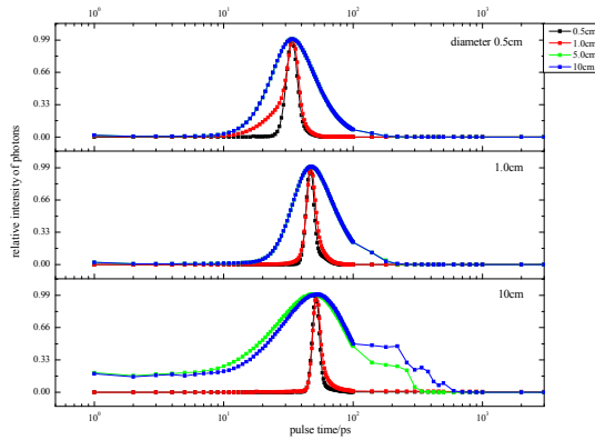
Figure 5: Photon time spectra in Ta targets with different diameters and thicknesses.
