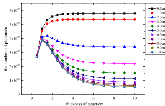
Figure 3: The numbers of X-ray photon produced by electrons in Ta targets.
