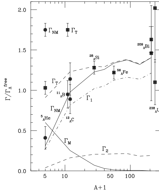
Fig. 1. Decay widths of a \Lambda in finite nuclei as a function of the nuclear mass number A (taken from Refs. [5, 7]).
