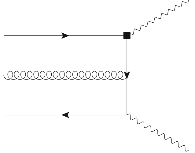
FIGURE 6: Diagrammatical representation of the three-particle higher-twist corrections to the vacuum-to- B -meson correlation function. The square box indicates the insertion of the weak vertex \bar{q} \Gamma_{\mu} b , and the waveline represents the interpolating current \bar{d} n \gamma_5 q for the light-pseudoscalar meson.
