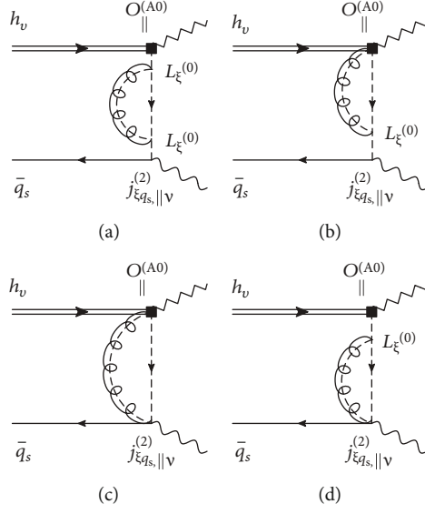
FIGURE 3: Diagrammatic representation of the vacuum-to- B -meson correlation function \Pi_{v,||}^A(p, q) defined with the A0 -type SCET operator O_{||}^{(A0)} = (\bar{\xi} W_c) \gamma_5 h_v and the power suppressed interpolating current j_{\xi q_s, || v}^{(2)} at one loop.
