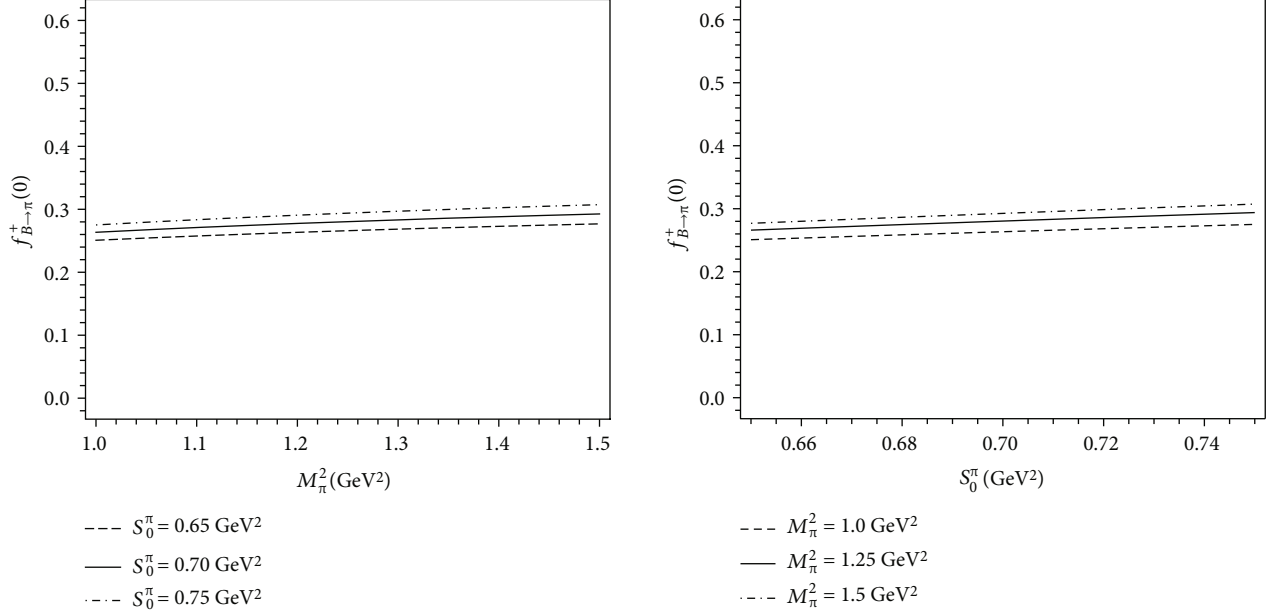
FIGURE 7: The Borel mass and threshold dependence of the form factor f_{B \rightarrow \pi}^+(0) .
