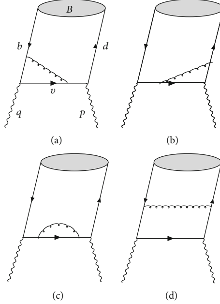
FIGURE 1: Diagrammatic representation of the correlation function \Pi_\mu(n \cdot p, \bar{n} \cdot p) at O(\alpha_s) . Figure 1 is reproduced from [32].
