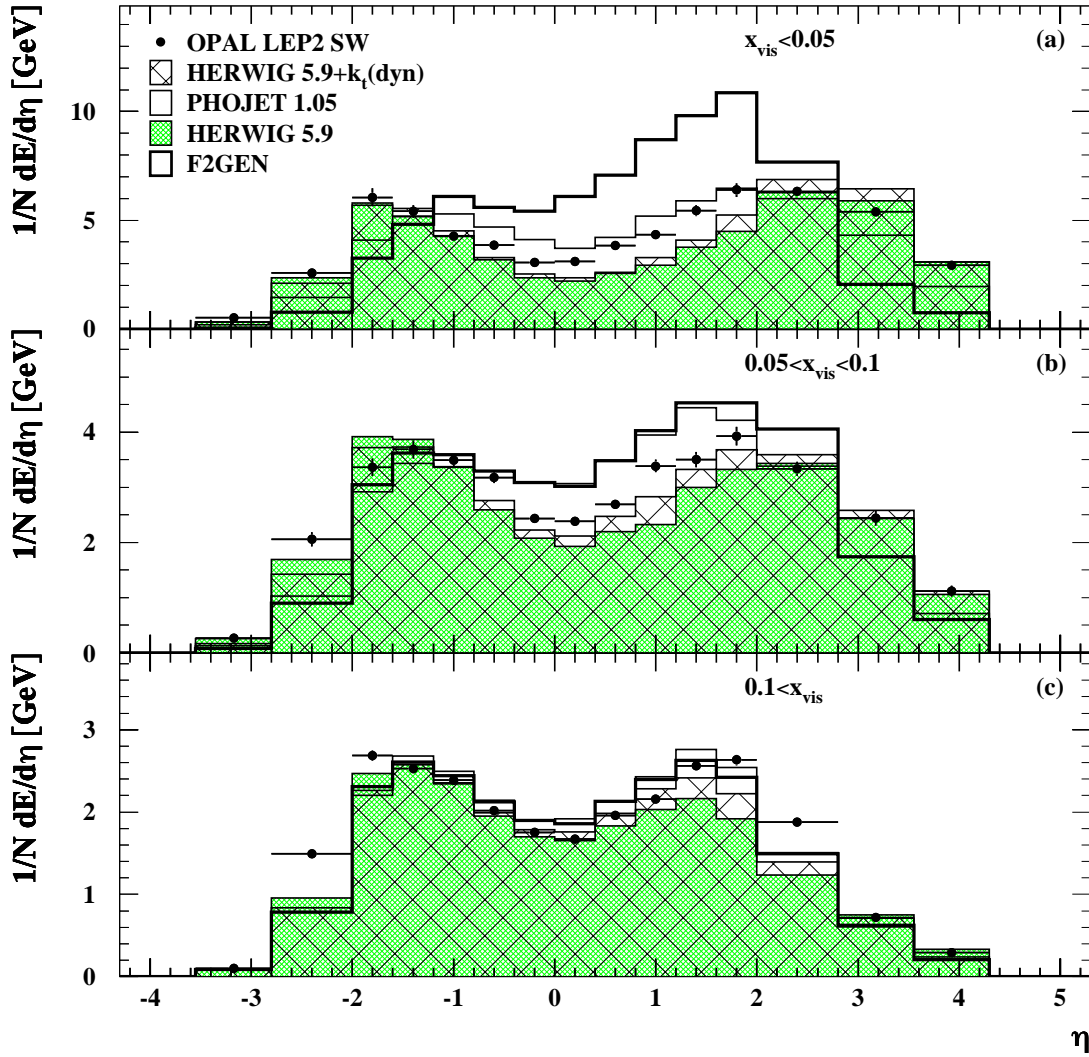
Figure 5.24: Comparison of hadronic energy flow per event as a function of the pseudorapidity, \eta = -\log(\tan(\theta/2)) , where \theta is measured with respect to the beam axis on the tag side, for the LEP2 SW sample. The samples are divided into three bins of x_{vis} . The errors are statistical only.
