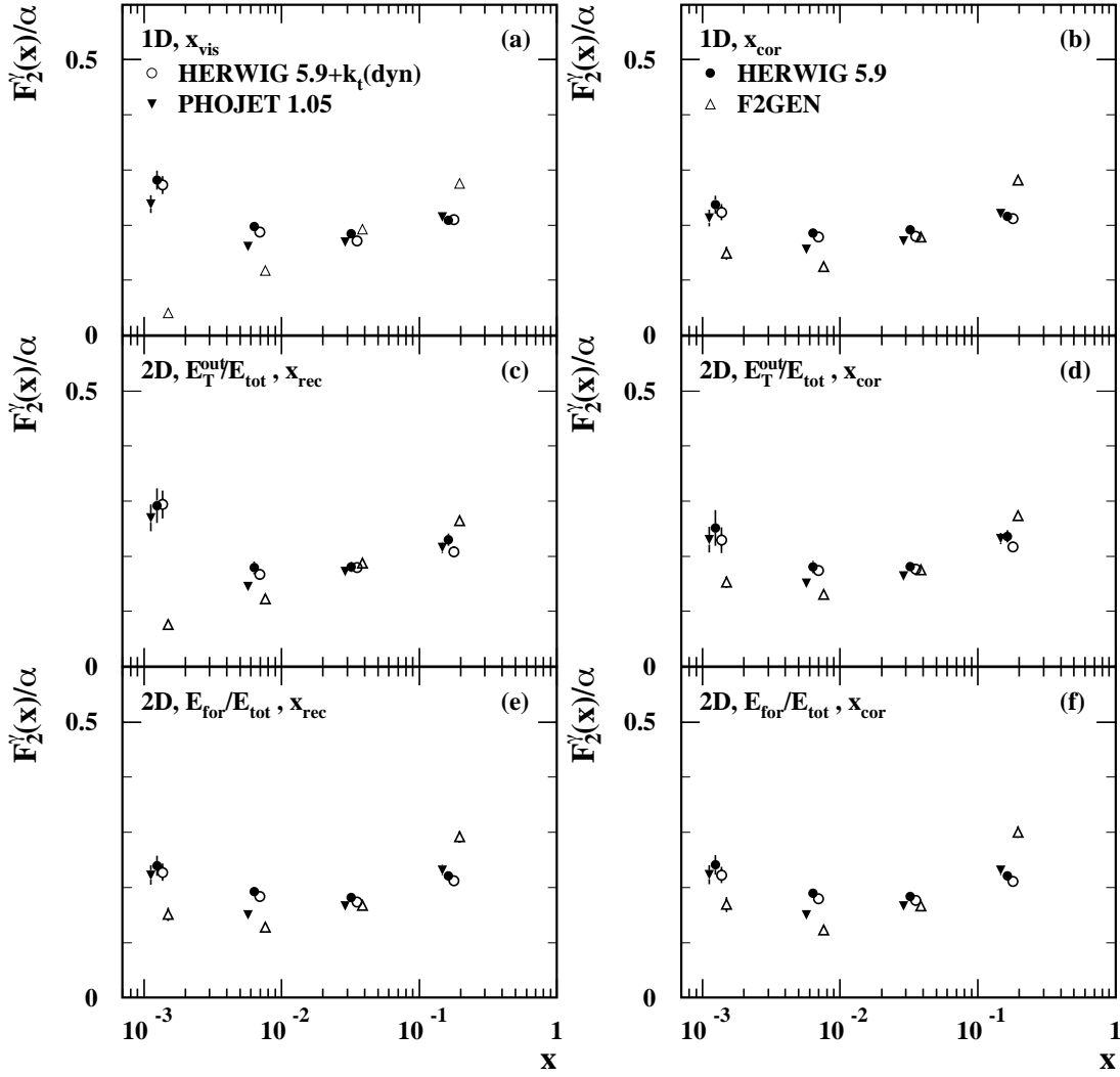
Figure 7.6: Unfolding of the LEP1 SW low Q^2 sample with 4 Monte Carlo models and different unfolding variables. The errors are statistical only. a) x_{\text{vis}} , b) x_{\text{cor}} , c) x_{\text{rec}} and E_{\text{T}}^{\text{out}} , d) x_{\text{cor}} and E_{\text{T}}^{\text{out}} , e) x_{\text{rec}} and E_{\text{for}}/E_{\text{total}} , f) x_{\text{cor}} and E_{\text{for}}/E_{\text{total}} .
