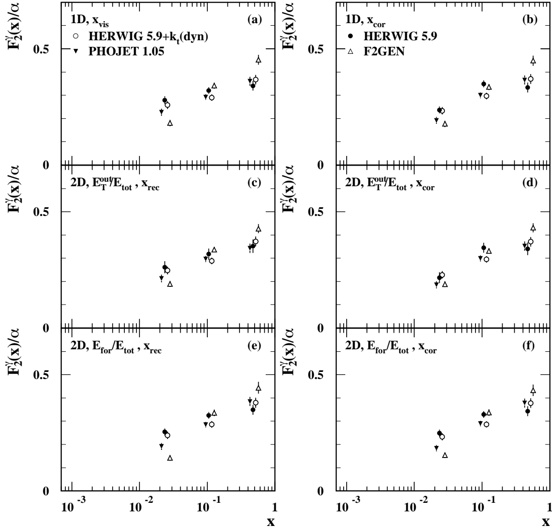
Figure 7.8: Unfolding of the LEP1 FD low Q^2 sample with 4 Monte Carlo models and different unfolding variables. The errors are statistical only. a) x_{\text{vis}} , b) x_{\text{cor}} , c) x_{\text{rec}} and E_{\text{T}}^{\text{out}} , d) x_{\text{cor}} and E_{\text{T}}^{\text{out}} , e) x_{\text{rec}} and E_{\text{for}}/E_{\text{total}} , f) x_{\text{cor}} and E_{\text{for}}/E_{\text{total}} .
