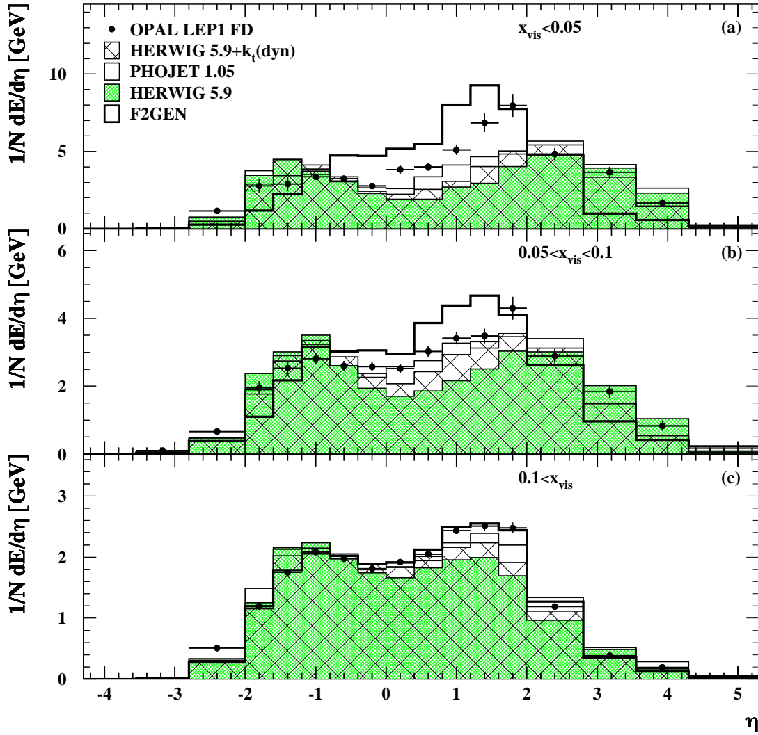
Figure 5.23: Comparison of hadronic energy flow per event as a function of the pseudorapidity, \eta = -\log(\tan(\theta/2)) , where \theta is measured with respect to the beam axis on the tag side, for the LEP1 FD sample. The samples are divided into three bins of x_{\text{vis}} . The errors are statistical only.
