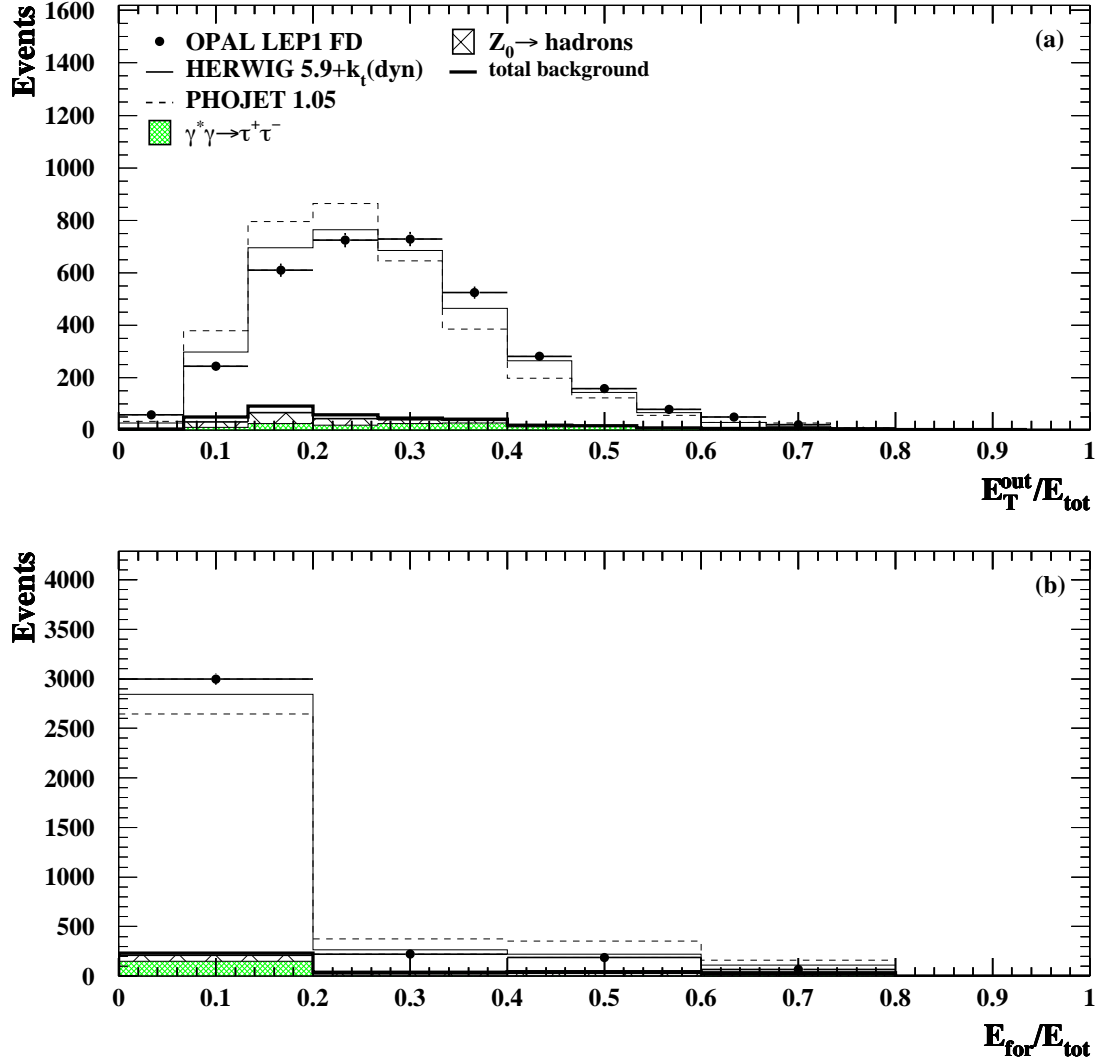
Figure 5.20: Comparison of data distributions with Monte Carlo predictions for the LEP1 FD sample. The dominant background sources, \gamma^*\gamma \rightarrow \tau^+\tau^- and Z^0 \rightarrow \text{hadrons} , the total background and the sum of the signal and the total background for HERWIG 5.9+ k_t (dyn) and PHOJET 1.05 are shown. The Monte Carlo samples have been normalised to the data luminosity. All selection cuts have been applied, except for any cut on the variable in the plot. The cuts are shown as dotted lines. The errors are statistical only. The variables in the plots are as defined in Figure 5.19.
