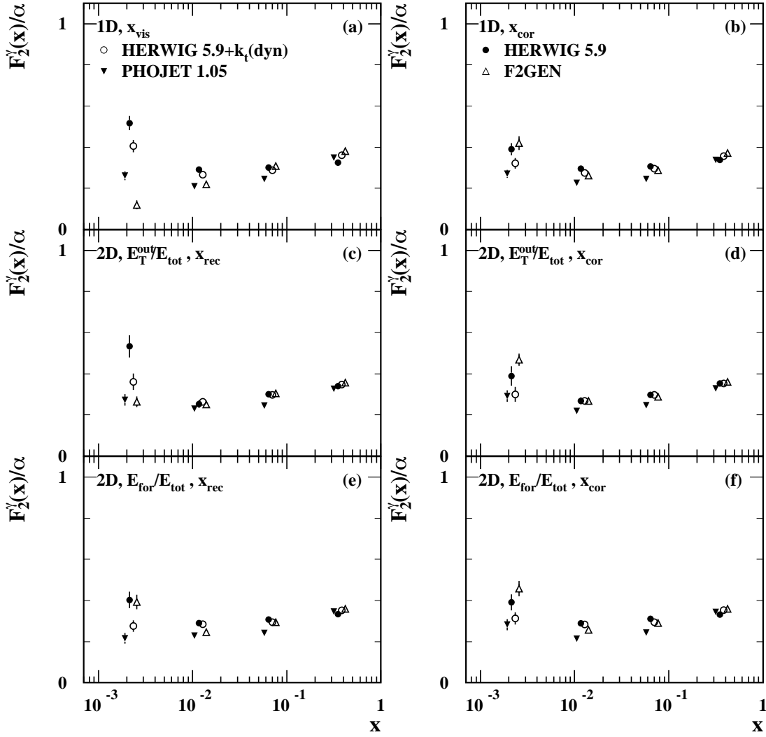
Figure 7.10: Unfolding of the LEP2 SW low Q^2 sample with 4 Monte Carlo models and different unfolding variables. The errors are statistical only. a) x_{\text{vis}} , b) x_{\text{cor}} , c) x_{\text{rec}} and E_T^{\text{out}} , d) x_{\text{cor}} and E_T^{\text{out}} , e) x_{\text{rec}} and E_{\text{for}}/E_{\text{total}} , f) x_{\text{cor}} and E_{\text{for}}/E_{\text{total}} .
