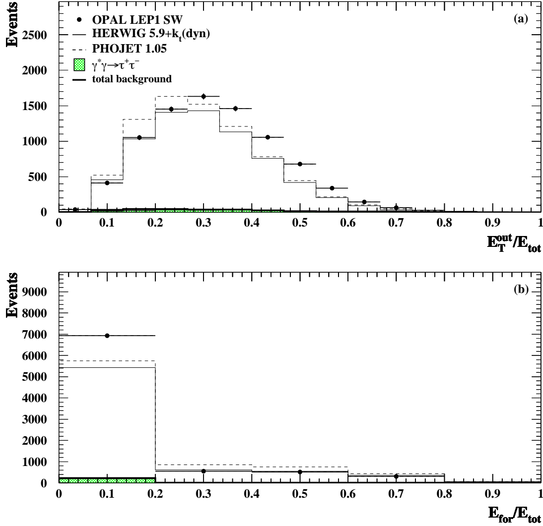
Figure 5.19: Comparison of data distributions with Monte Carlo predictions for the LEP1 SW sample. The dominant background source, \gamma^*\gamma \rightarrow \tau^+\tau^- , the total background and the sum of the signal and the total background for HERWIG 5.9+ k_t (dyn) and PHOJET 1.05 are shown. The Monte Carlo samples have been normalised to the data luminosity. All selection cuts have been applied, except for any cut on the variable in the plot. The cuts are shown as dotted lines. The errors are statistical only. The distributions shown are: (a) E_T^{\text{out}}/E_{\text{tot}} , the transverse hadronic energy out of the plane containing the beam line and the tagged electron, divided by the total observed energy, and (b) E_{\text{for}}/E_{\text{tot}} , the observed energy in the forward regions divided by the total observed energy.
