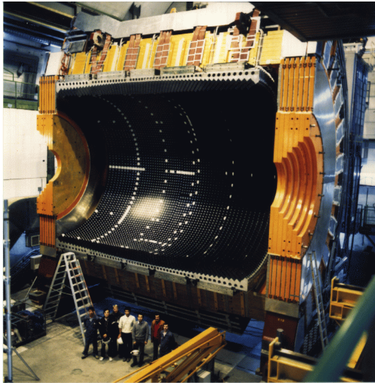
Figure 2.5: A picture taken during the construction of OPAL, showing half of the barrel lead glass calorimeter.
