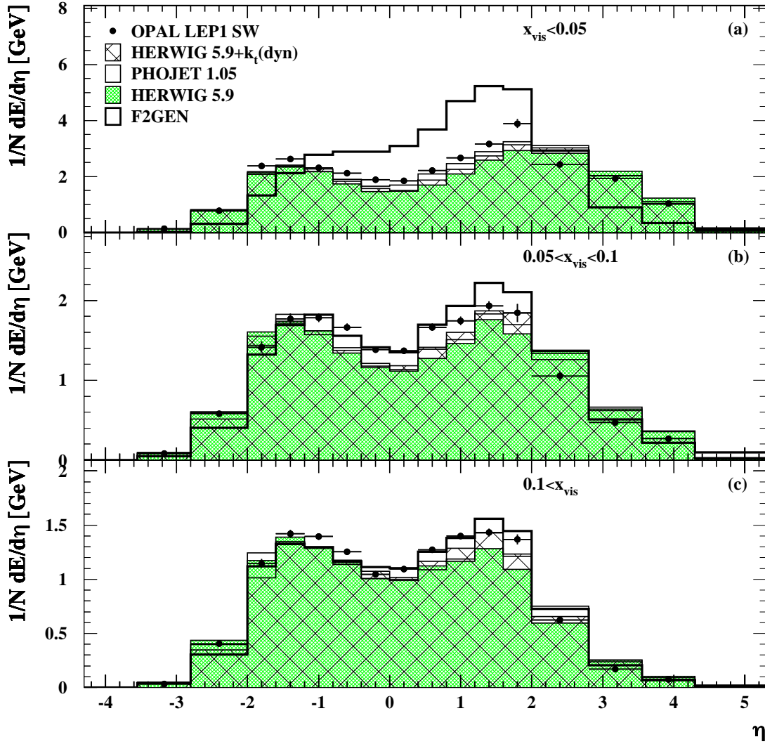
Figure 5.22: Comparison of hadronic energy flow per event as a function of the pseudorapidity, \eta = -\log(\tan(\theta/2)) , where \theta is measured with respect to the beam axis on the tag side, for the LEP1 SW sample. The samples are divided into three bins of x_{\text{vis}} . The errors are statistical only.
