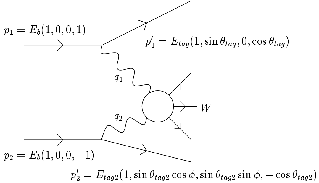
Figure 3.1: Deep inelastic electron-photon scattering.
