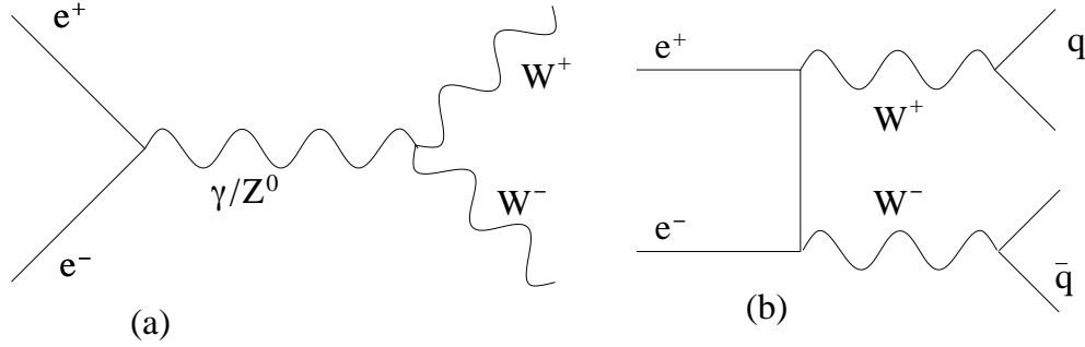
Figure 5.4: W pair production and decay: (a) annihilation, (b) conversion.
