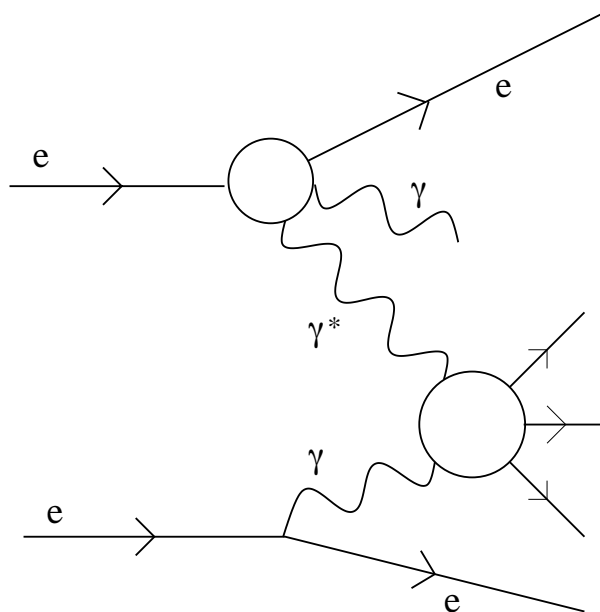
Figure 4.2: Radiative corrections to two-photon DIS.
