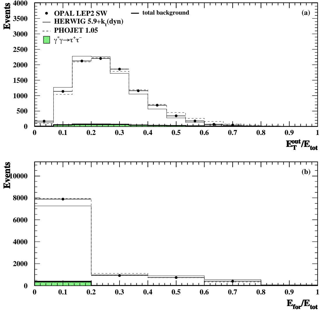
Figure 5.21: Comparison of data distributions with Monte Carlo predictions for the LEP2 SW sample. The dominant background source, \gamma^*\gamma \rightarrow \tau^+\tau^- , the total background and the sum of the signal and the total background for HERWIG 5.9+ k_t (dyn) and PHOJET 1.05 are shown. The Monte Carlo samples have been normalised to the data luminosity. All selection cuts have been applied, except for any cut on the variable in the plot. The cuts are shown as dotted lines. The errors are statistical only. The variables in the plots are as defined in Figure 5.19.
