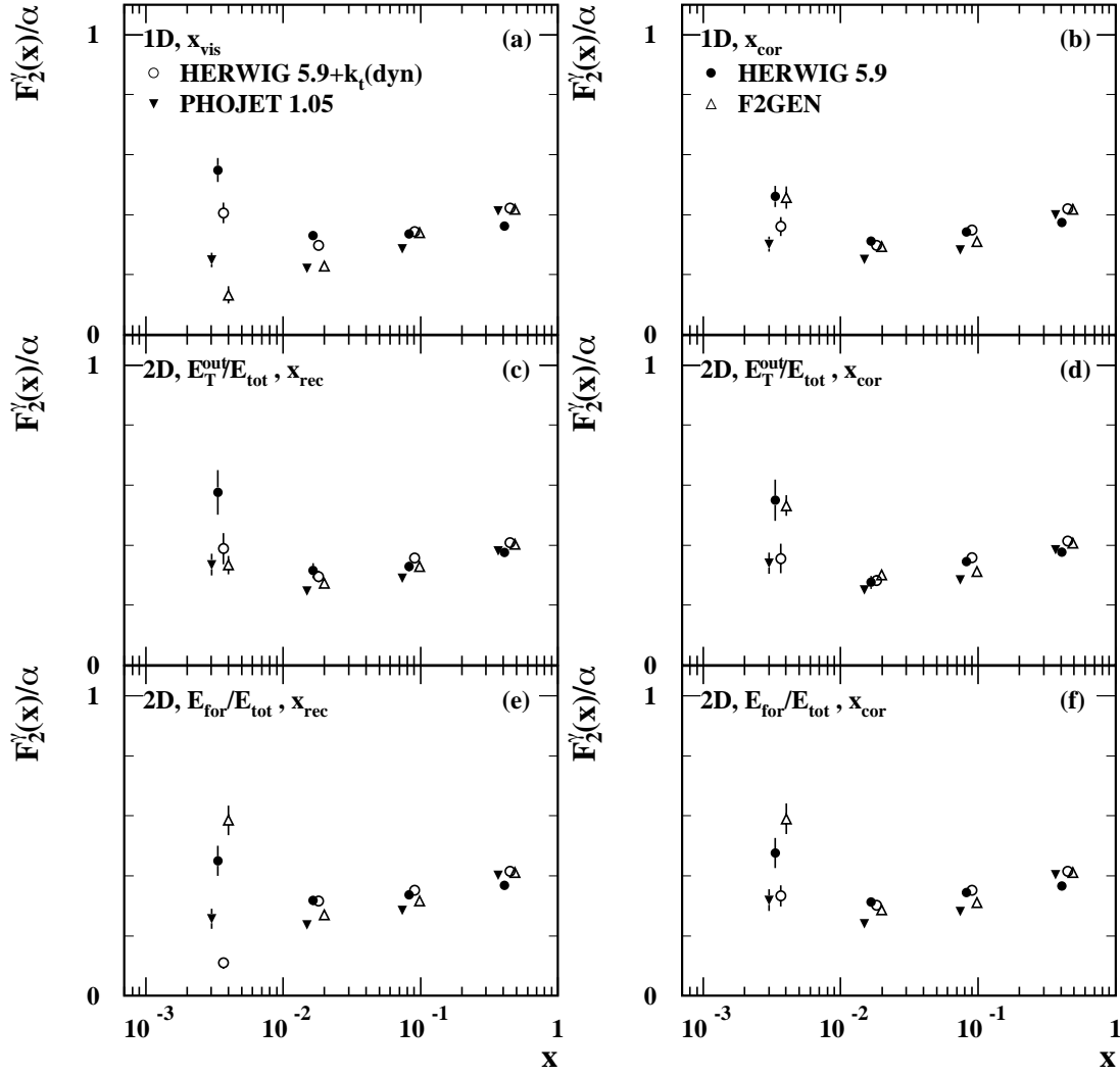
Figure 7.11: Unfolding of the LEP2 SW high Q^2 sample with 4 Monte Carlo models and different unfolding variables. The errors are statistical only. a) x_{\text{vis}} , b) x_{\text{cor}} , c) x_{\text{rec}} and E_{\text{T}}^{\text{out}} , d) x_{\text{cor}} and E_{\text{T}}^{\text{out}} , e) x_{\text{rec}} and E_{\text{for}}/E_{\text{total}} , f) x_{\text{cor}} and E_{\text{for}}/E_{\text{total}} .
