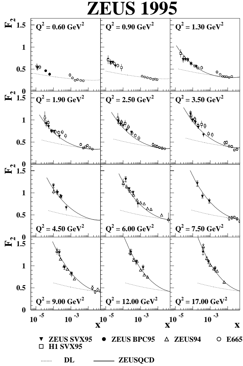
Figure 3.4: Measurements of F_2^p by ZEUS [32].
