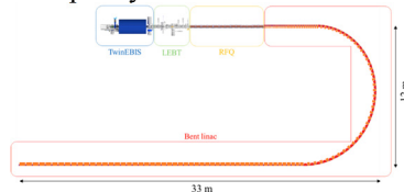
Figure 3: Layout of the bent linac.
