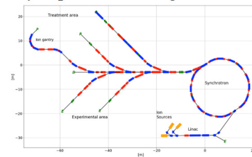
Figure 1: Layout of the synchrotron-based facility.
