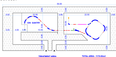
Figure 5: A compact single-room SC ion therapy facility.
