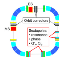
Figure 2: Layout of the superconducting synchrotron.
