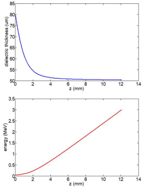
Figure 3: The dielectric thickness and the beam energy along the beam line.
