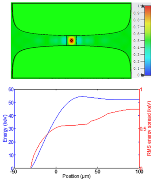
Figure 2: Simulated electric field and the beam energy.
