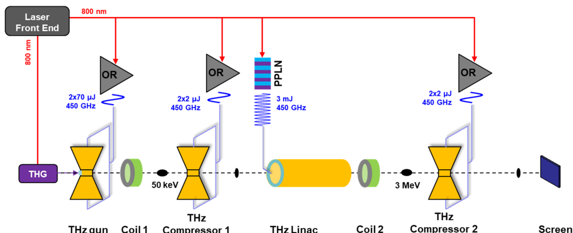
Figure 1: Schematic of the 3 MeV terahertz-driven electron source beamline.
