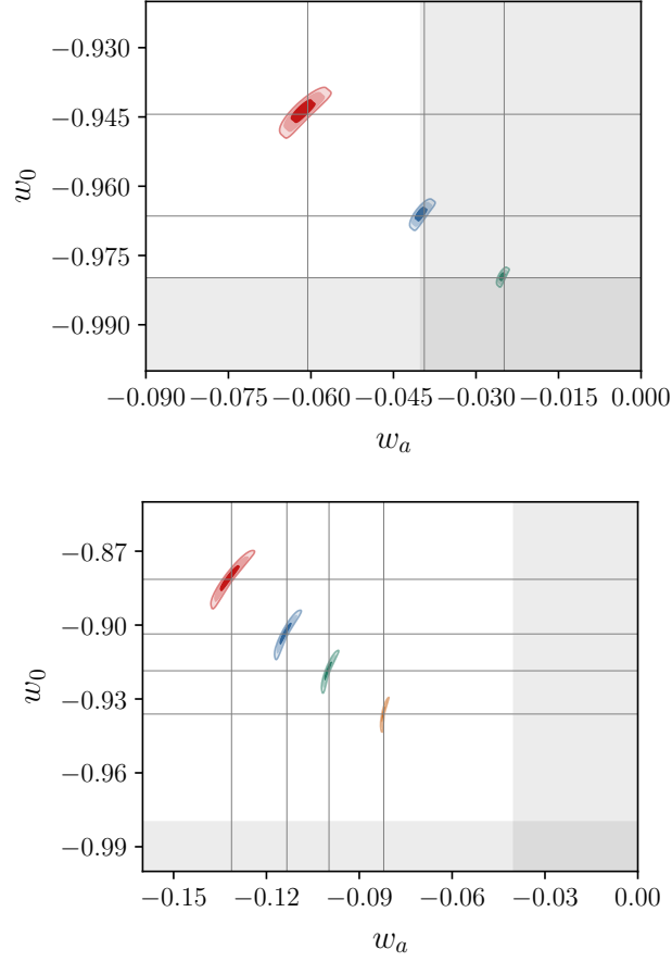
Figure 2.15: Upper panel: Constraints on w_0 and w_a for Exp-model I, and for three cases of \phi_F = -10 (red contours), \phi_F = -10.5 (blue contours), and \phi_F = -11 (green contours). The shaded, grey regions indicate a rough estimate of the target sensitivity for Stage IV large-scale structure surveys in combination with CMB experiments, expected to detect deviations of up to \sim 2\% and \sim 4\% in w_0 and w_a , respectively, from the \Lambda CDM values. Lower panel: The same as in the left panel, but for Exp-model II. Here, red, blue, green, and orange contours correspond to \phi_F = -10 , \phi_F = -10.5 , \phi_F = -11 , and \phi_F = -12 , respectively. Note that all these cases for Exp-model II show detectable deviations from \Lambda CDM.
