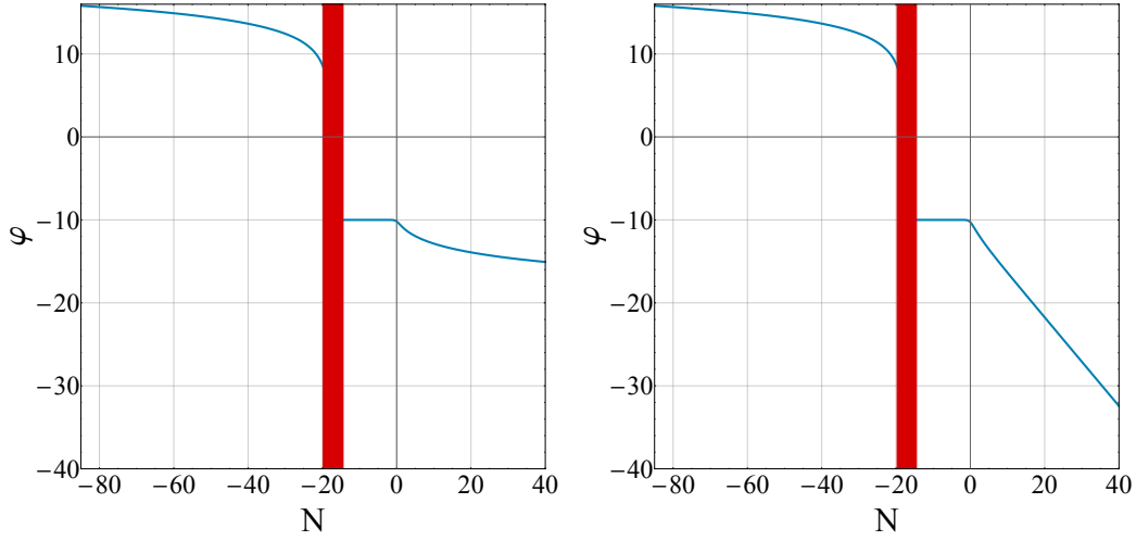
Figure 2.12: Left panel: Evolution of the scalar field \phi as a function of the number of e -folds N over the entire history of the universe for Exp-model I and for the same set of parameters used for computing the inflationary variables shown in Fig. 2.11 with a viable late-time cosmological history. The vertical, red bands depict the period after the end of inflation and before the time at which the scalar field freezes, separating the inflationary and late-time periods. This period includes kination and reheating. Note that the field rolls down during inflation and kination (not shown), and then freezes after reheating (to -10 in this example), for almost the entire history until very recently when it unfreezes again and starts rolling its potential; this is the onset of dark energy domination. N = 0 corresponds to the present time. Right panel: The same as in the left panel, but for Exp-model II. Note the different dynamics for \phi compared to Exp-model I in the future ( N > 0 ).
