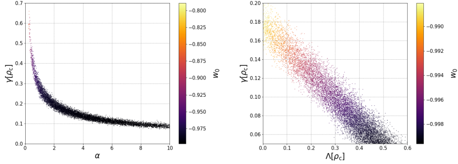
Figure 2.23: Constraints on \gamma , \alpha and \Lambda for the linear, interacting, \alpha -attractor model with the linear potential V(\varphi) = \gamma\sqrt{6\alpha}(\tanh \frac{\varphi}{\sqrt{6\alpha}} + 1) + \Lambda , when \Lambda is fixed to 0 (left) and when \alpha is fixed to 7/3 (right). Note that both \gamma and \Lambda are presented in units of the critical density today. The samples are color-coded with the value of w_0 .
