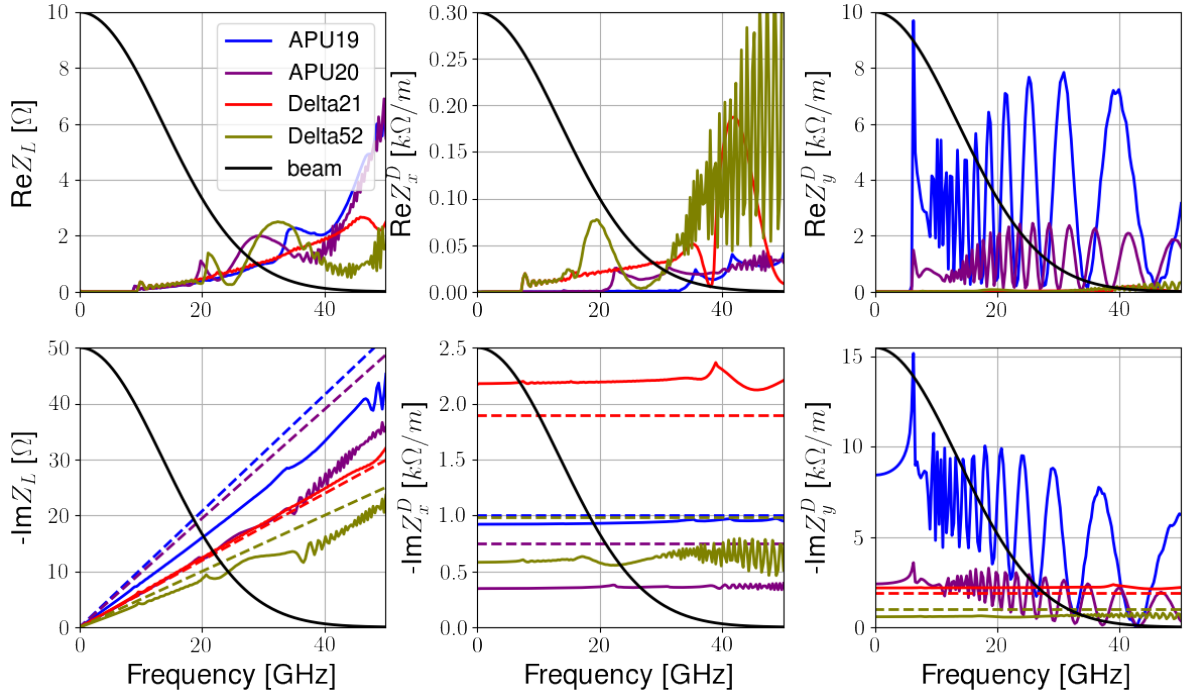
Figure 20 – Geometric impedance from the tapered transitions of the undulators. Solid lines represent numerical calculations performed with ECHOz1 and ECHOz2 for the Delta undulator and with ECHOzR for the APU. Dashed lines are the prediction by the analytic formulas studied in subsection 3.9.1. Full black curves show the spectrum of a 2.5 mm long gaussian bunch.
