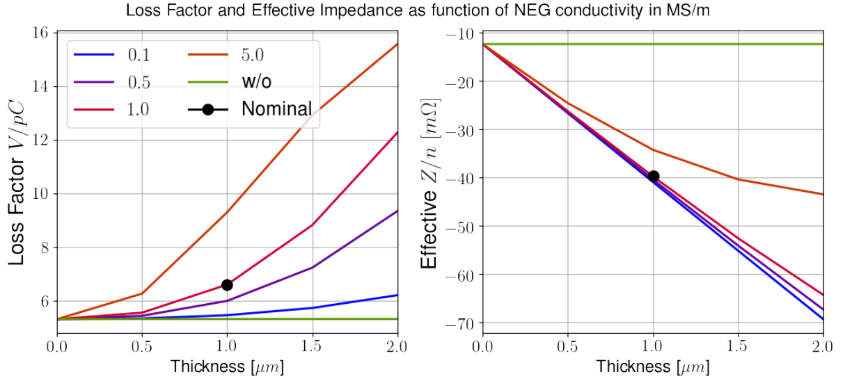
Figure 13 – Loss factor (left) and effective longitudinal impedance (right) for a 2.5 mm bunch as a function of the coating thickness for several different values of NEG conductivity, in MS\,m^{-1} .
