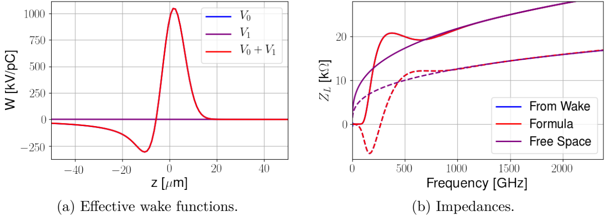
Figure 27 – CSR effective wake functions and impedances calculated using the parameters of the Sirius low-field dipoles. Solid lines represent the real part of the impedance and dashed lines, the imaginary part. In both plots the blue line coincides with the red one and, therefore, it is not visible.
