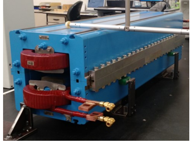
(b) Picture of a real dipole magnet.
