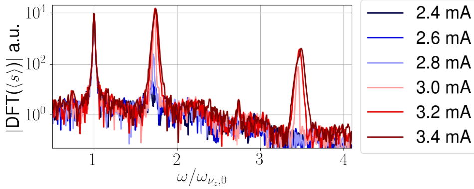
Figure 45 – Discrete Fourier transform of the time-dependent bunch centroid, as a function of frequency in units of the zero-current synchrotron frequency.
