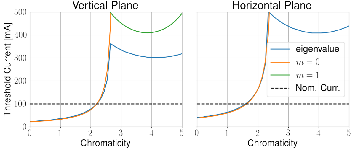
Figure 53 – Effect of chromaticity on the most unstable mode of the transverse coupled-bunch instabilities for the first phase of operation of the Sirius storage ring.
