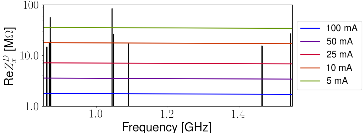
Figure 38 – Transverse PETRA 7–Cell cavity impedance compared with the minimum shunt impedance needed to drive coupled–bunch instabilities for several values of total beam current.
