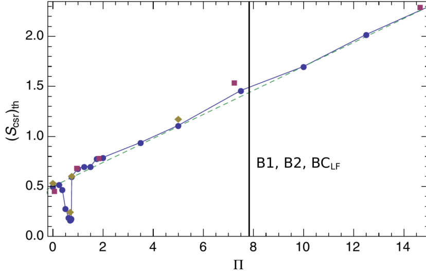
Figure 26 – Plot adapted from Bane et al. (2010): CSR threshold strength, (S_{\text{csr}})_{\text{th}} , as a function of the shielding parameter, \Pi . Blue dots: simulations with the VFP solver. Purple squares: results of the linearized Vlasov equation (does not include damping). Olive diamonds: results with a damping factor two times larger. Dashed line: the scaling (S_{\text{csr}})_{\text{th}} = 0.5 + 0.12\Pi . Black line: shielding parameters for the low field dipoles of Sirius, B1, B2 and the low field part of the BC magnet (BC LF ). The shielding for the high field part of this same magnet (BC HF ) is larger than the maximum value showed.
