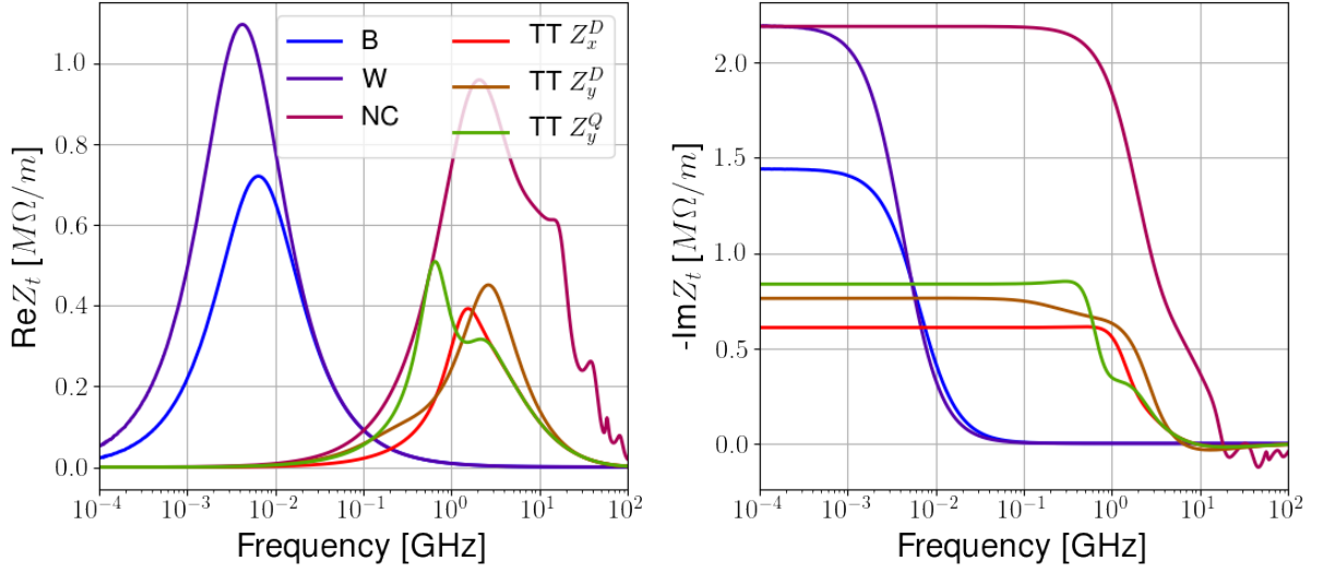
Figure 18 – Transverse impedances of the four models of kicker analysed.
