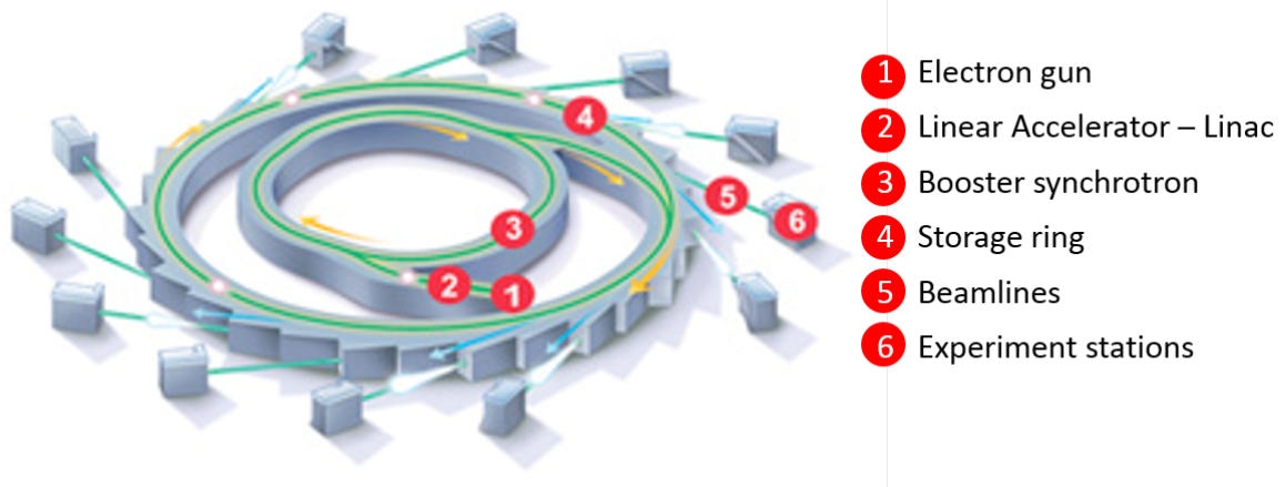
Figure 1 – Schematic of a storage-ring-based light source showing the three main systems: the injection systems, composed of an electron gun, a Linear Accelerator (LINAC) and a booster; the storage ring and the beamlines, with the experiment stations at their ends.
