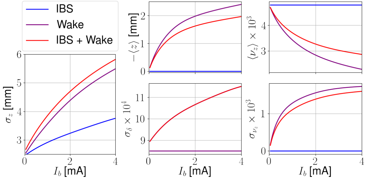
Figure 40 – Stationary parameters of the longitudinal plane, calculated from the solution of the Haissinski equation.
