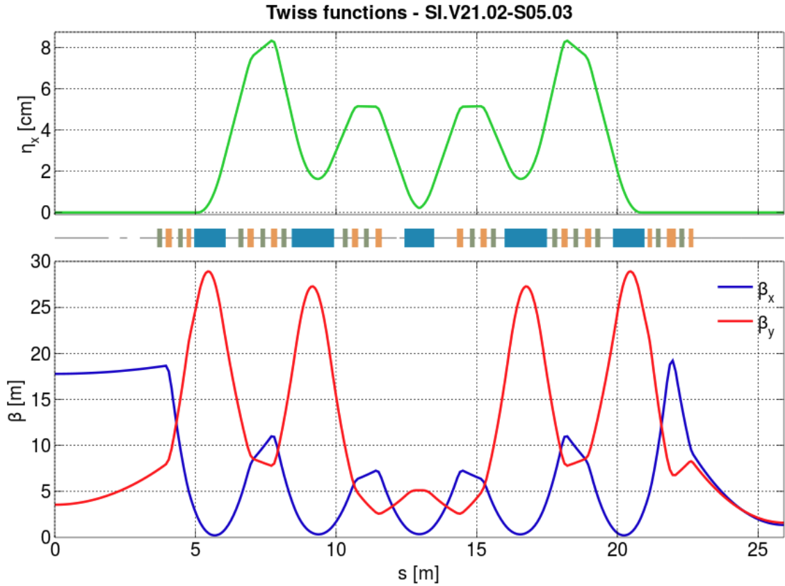
Figure 7 – Optical (twiss) functions for one fourth of a period of the Sirius lattice. In green is shown the dispersion function. In red, the vertical betatron function is shown and in blue, the horizontal betatron function. Notice the strong focusing of the betatron functions at the center of the low-beta (B) sections. (copied from Sirius (2013).)
