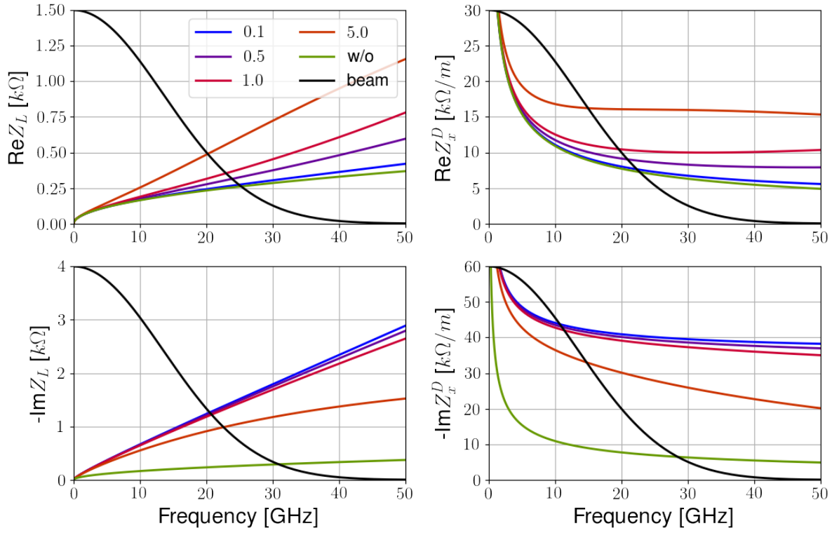
(a) Wall Impedance as a function of NEG conductivity (in \text{MS m}^{-1} ).
