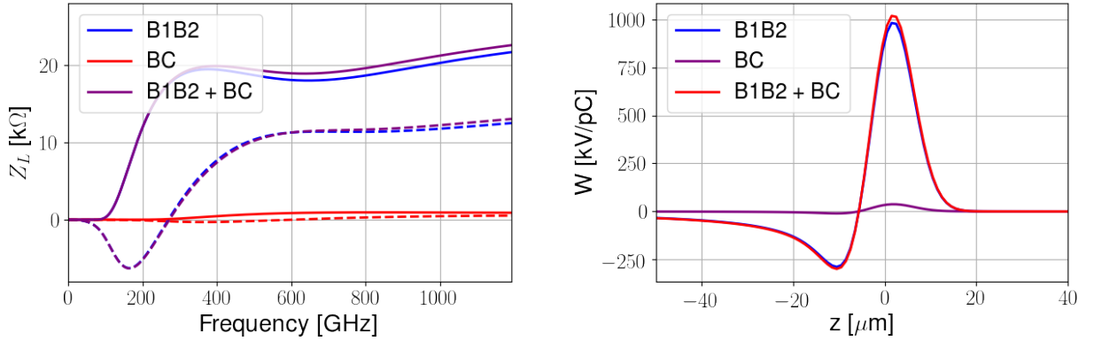
Figure 28 – Total CSR impedance (left) and wake (right) models for Sirius, considering the two types of dipoles. Solid lines represent the real part of the impedance and dashed lines represent the imaginary part.
