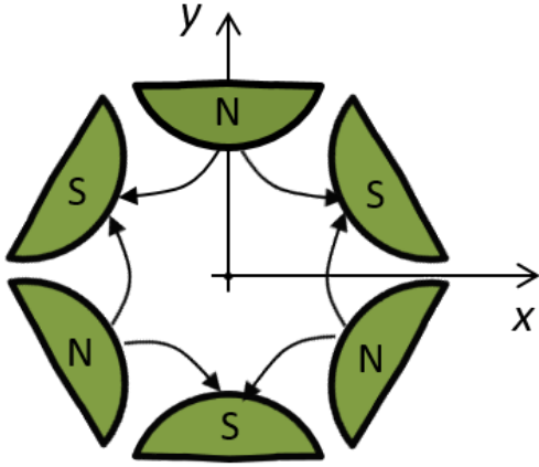
(a) Schematic figure of a sextupole magnet, where N and S indicate the North and South poles of the magnet and the curved arrows indicate the magnetic field lines.
