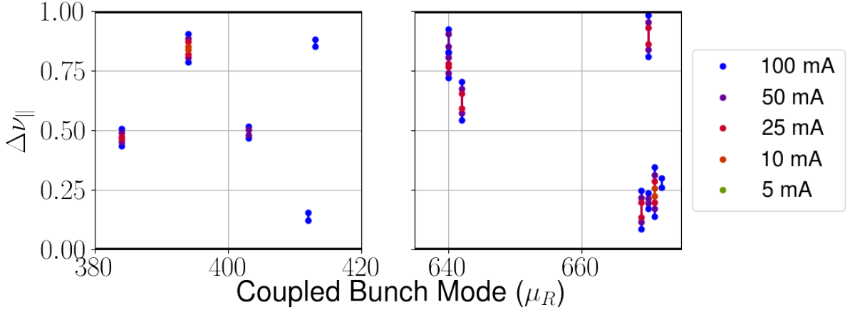
Figure 37 – The horizontal axis indicates the mapping of the RF cavity longitudinal impedance peak frequencies in the coupled-bunch modes. Vertical axis indicates the fractional part of one revolution frequency in the ring. Black horizontal lines are \pm\nu_z and the interval defined by the dots is the interval in which sampling by the synchrotron tune corresponds to instability at the indicated current.
