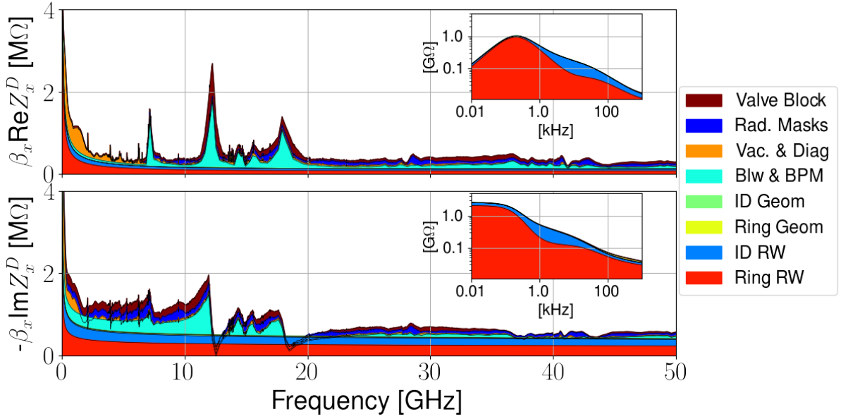
Figure 31 – Horizontal dipolar impedance budget for Sirius.
