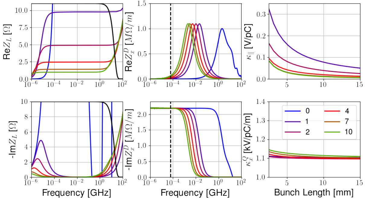
Figure 19 – Longitudinal (left) and dipolar horizontal (middle) impedances as a function of the frequency for several values of coating thickness, in \mu\text{m} . The power spectrum of a 2.5 mm bunch is also shown (solid black) to highlight the important part of the frequency spectrum, and the first horizontal betatron line (black dashed) is shown in the middle. In the right is shown the loss factor (above) and quadrupolar kick factor (below) as a function of the bunch length for several values of coating thickness.
