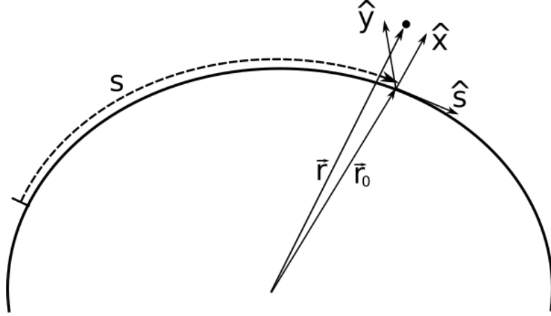
Figure 9 – Frenet-Serret reference frame of a storage ring, with right-handed coordinate system \{\hat{x}, \hat{y}, \hat{s}\} . Adapted from (LEE, 1999, pp. 123).
