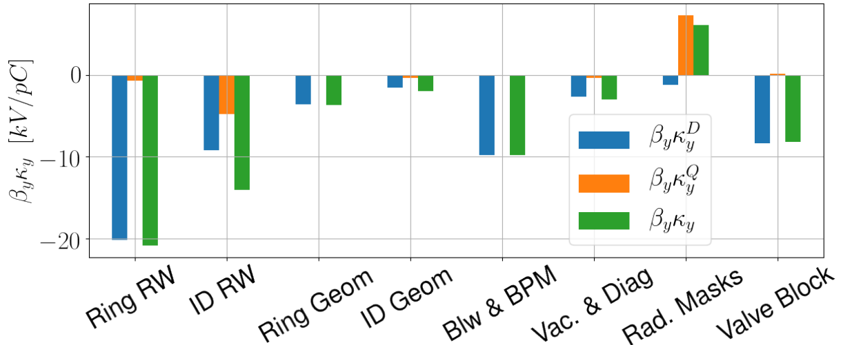
Figure 34 – Vertical kick factors for single-bunch operation mode.
