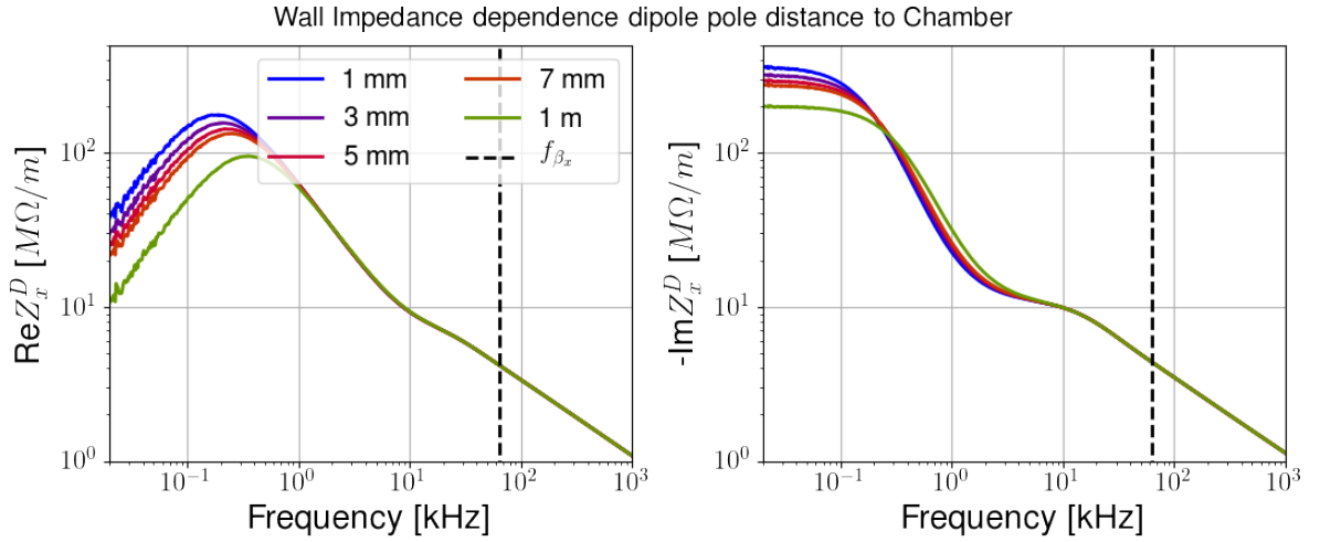
Figure 14 – Low frequency impedance for different distances of the dipole magnetic poles to the vacuum chamber.
