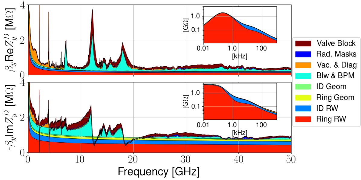
Figure 32 – Vertical dipolar impedance budget for Sirius.
