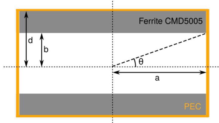
Figure 17 – Tsutsui model for the window-frame kicker magnet.
