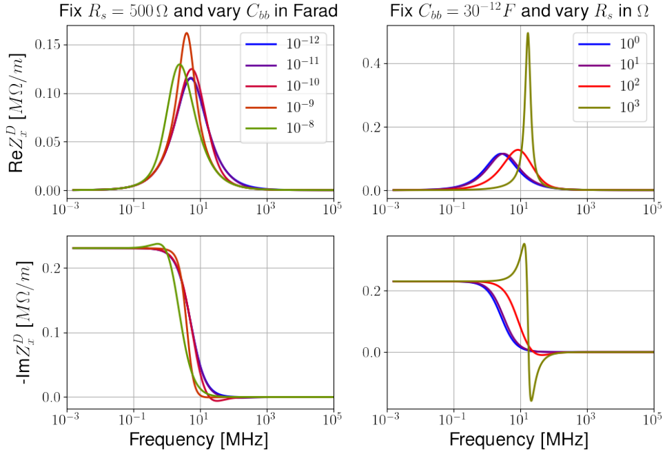
Figure 16 – Coupled flux impedance of the dipole kicker magnet as a function of the frequency for several values of capacitance (left) and resistance (right).
