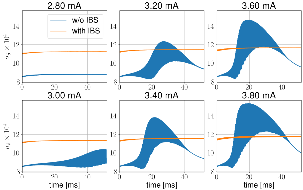
Figure 44 – Time evolution of the energy spread for different bunch currents close to the threshold of the sawtooth-like instability.
