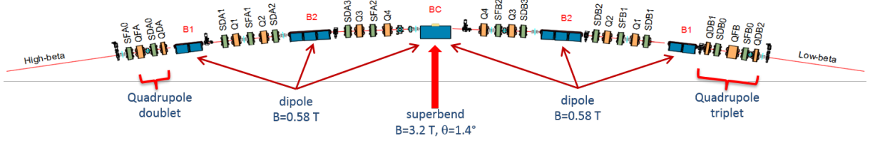
Figure 6 – One fourth of the unit cell of the Sirius storage ring. Dipoles are shown in blue, quadrupoles in orange and sextupoles in green. The vacuum pumps and valves are also shown. Only half of the high-beta (A) and of the low-beta (B) straight sections are shown. The arc and the straight sections are repeated to form the unit cell in the following way: A-B-B-B. The unit cell is then, repeated five times to form the ring.
