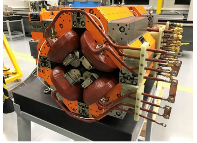
(b) Picture of a real quadrupole magnet, with the coils that generate the magnetic field and the iron core that guide and shape the field lines inside the gap.
