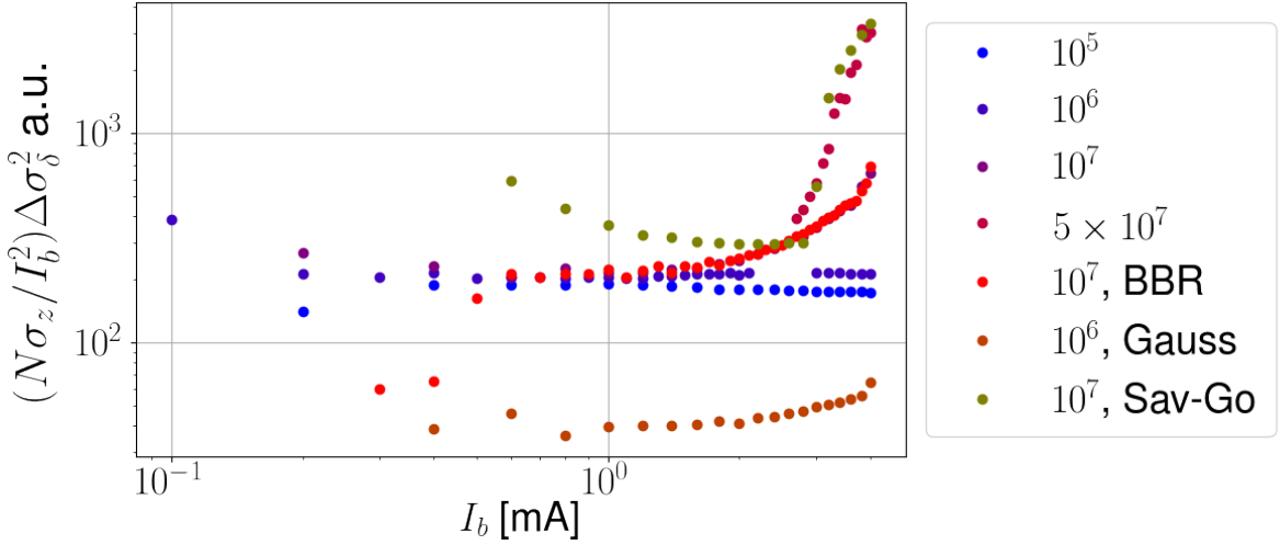
Figure 47 – Energy spread increase in simulations multiplied by N_p\sigma_z/I_b^2 . The curves 10^5 , 10^6 , 10^7 and 5 \times 10^7 were performed with the same wake function using the PIC method, while for curve (10^7, \text{BBR}) the dynamics was simulated using directly the BBRs from the impedance model presented in subsection 7.2.1. For the curve (10^6, \text{Gauss}) a convolution with a 40\text{ }\mu\text{m} gaussian bunch was applied to the wake and a Savitzky–Golay filter was applied in the simulation of the results of (10^7, \text{Sav-Go}) .
