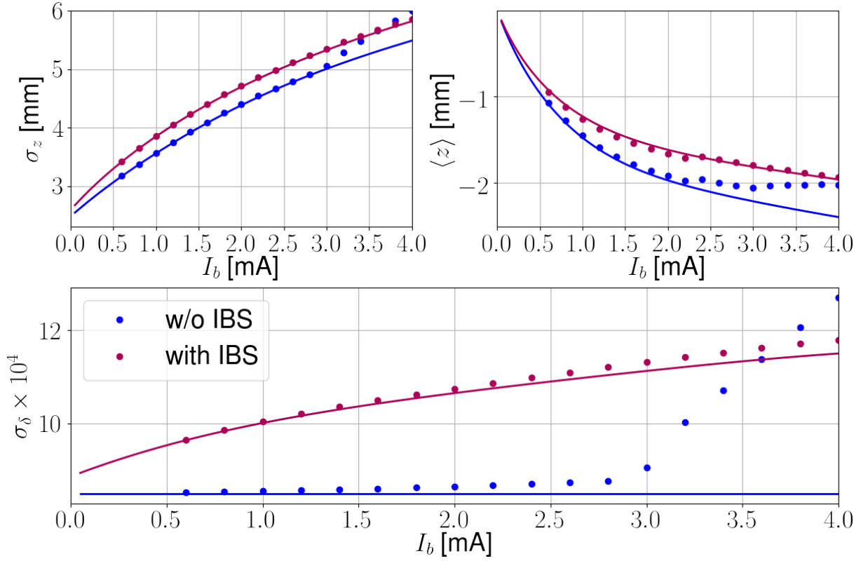
Figure 43 – Main parameters of the beam obtained from tracking (dots) as a function of the current for the simulations with and without the effects of IBS. The values shown here are averages over all the 3 \times 10^4 turns of the simulation. The solid lines are the results obtained from the solution of the Haissinski equation.
