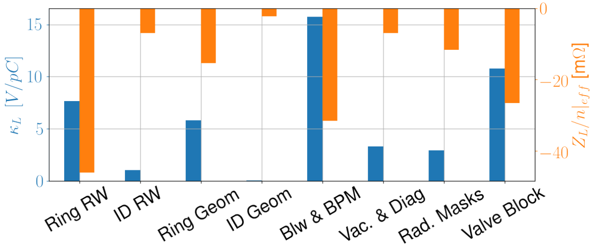
Figure 30 – Single-bunch loss factor (left, blue) and effective impedance (right, orange) calculated for the nominal operation mode of phase1 for Sirius.
