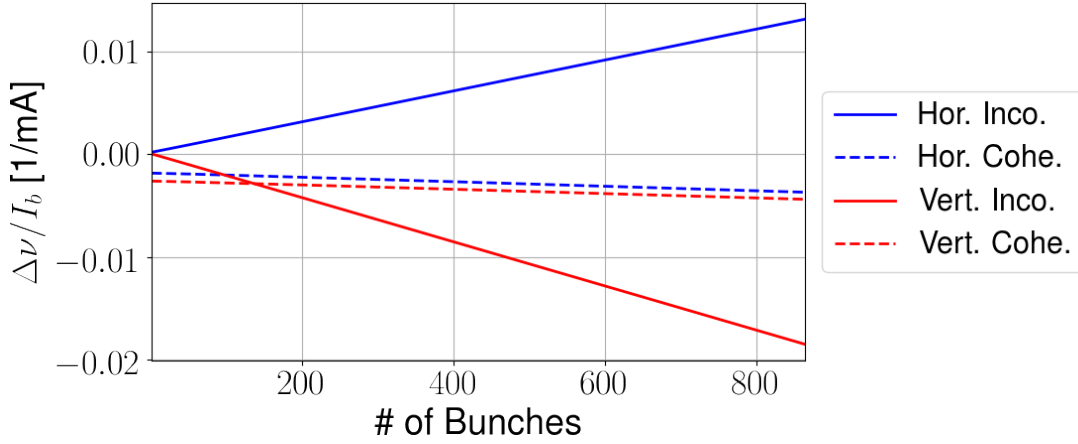
Figure 35 – Tune shift normalized by the bunch current as a function of the number of bunches in uniform filling.
