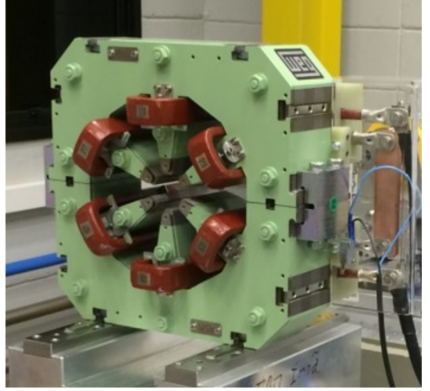
(b) Picture of a real sextupole magnet.
