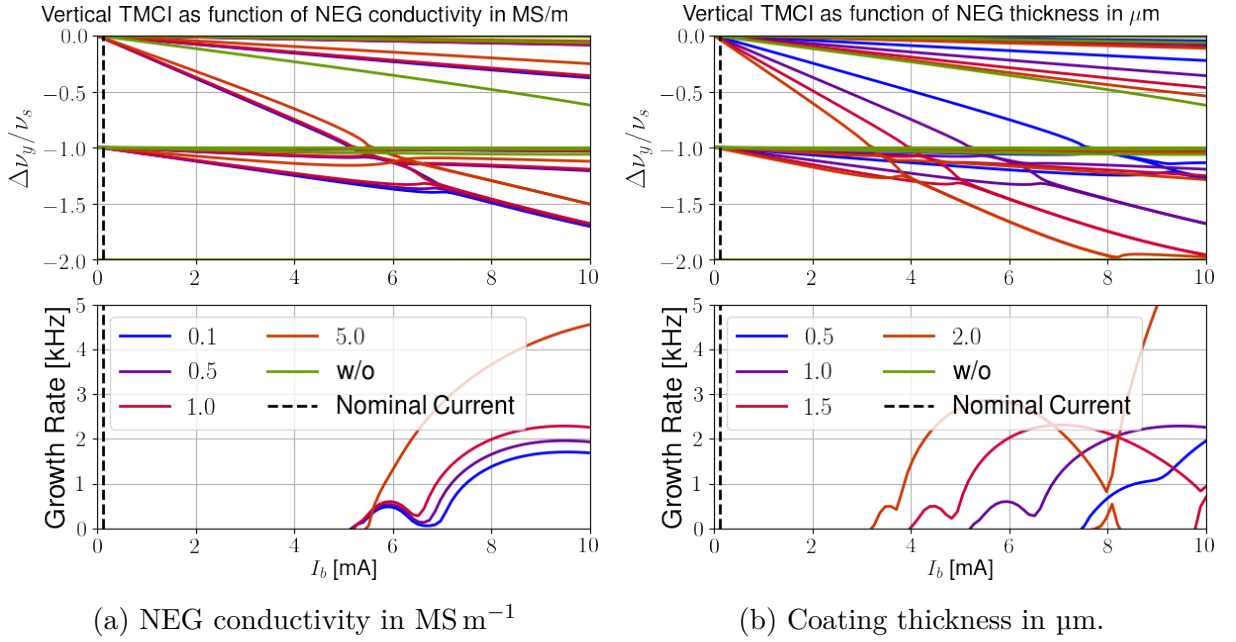
Figure 12 – Simulations of TMCI for single bunch in the machine using the parameters of the first phase of operation of the storage ring, as shown in Table 1, and for several different values of (a) NEG conductivity and (b) coating thickness.
