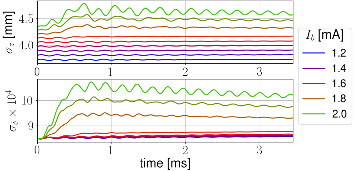
Figure 51 – Time evolution of the energy spread and bunch length for different bunch currents in the simulation with CSR and the machine impedance budget.
