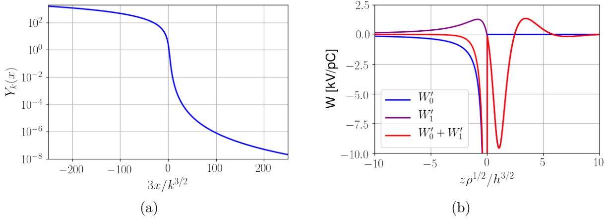
Figure 25 – (a) behavior of Y_k(x) as a function of 3x/k^{3/2} showing its smooth dependency. (b) Sum of the two terms of the CSR impedance: the free-space contribution, W'_0 and the shielding term, W'_1 , where it becomes clear the cancellation of the long tail at positions ahead of the source particle ( z negative).
