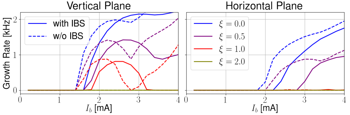
Figure 55 – Transverse single-bunch instabilities for the first phase of operation of the Sirius storage ring, considering effects of IBS and potential well distortion.
