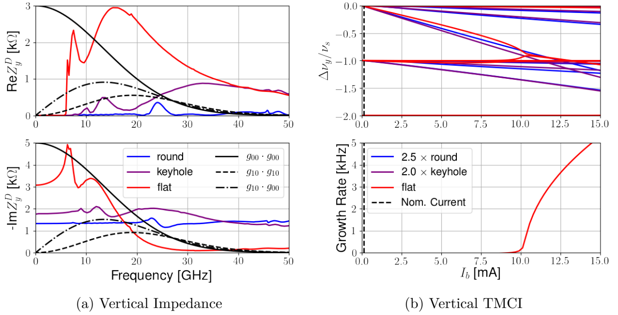
Figure 23 – Comparison of the impedance and its effect on the beam through simulations of mode-coupling instability for different models of impedance. For the TMCI a gaussian single bunch with 2.5 mm root-mean-square (rms) length was considered. The impedance used was that of the 20 components along the ring, multiplied by the average betatron function at the magnet’s position.
