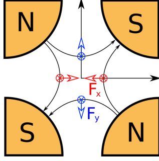
(a) Schematic figure of a quadrupole magnet, where the curved arrows indicate the magnetic field lines and the red/blue arrows indicate the direction of the horizontal/vertical forces felt by an electron entering the sheet. Notice this quadrupole focuses in the horizontal, so it is a focusing quadrupole.
