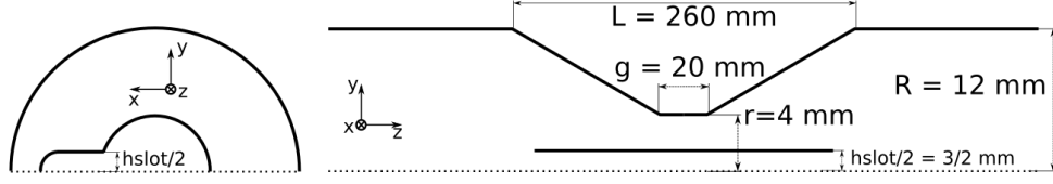
Figure 22 – Scheme of the keyhole-shaped chamber for the BC magnet.
