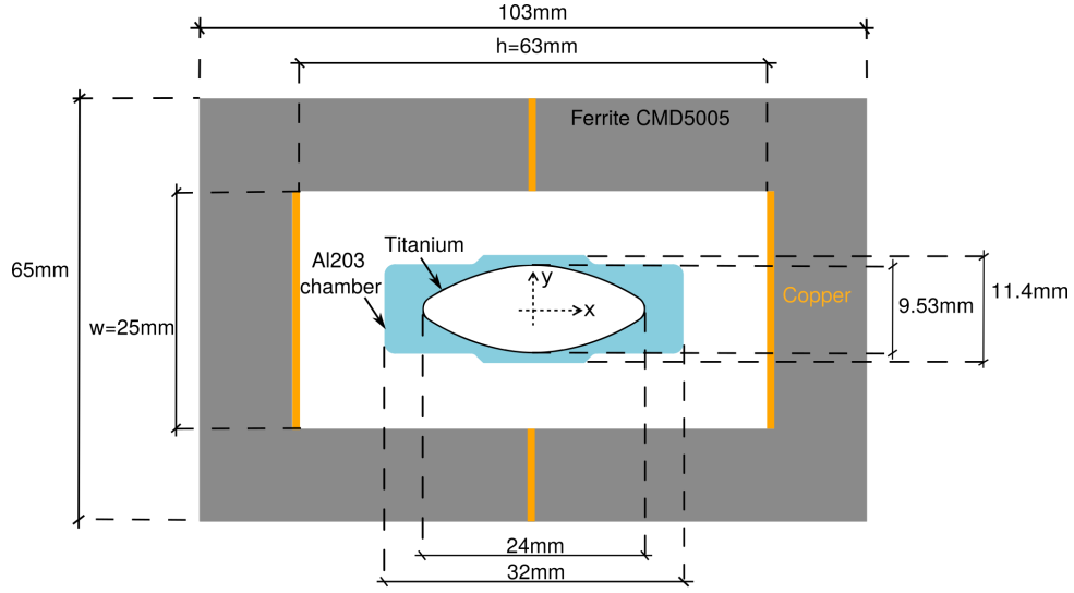
Figure 15 – Cross section of the Sirius storage ring kicker window-frame magnet.
