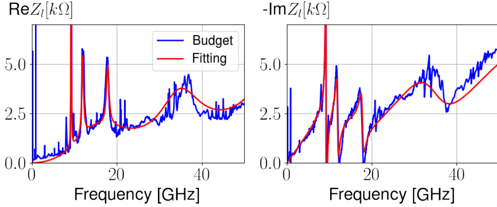
Figure 41 – Comparison of the complete longitudinal impedance calculated for the Sirius storage ring (blue) with the BBRs fitting presented in Table 8 (red).
