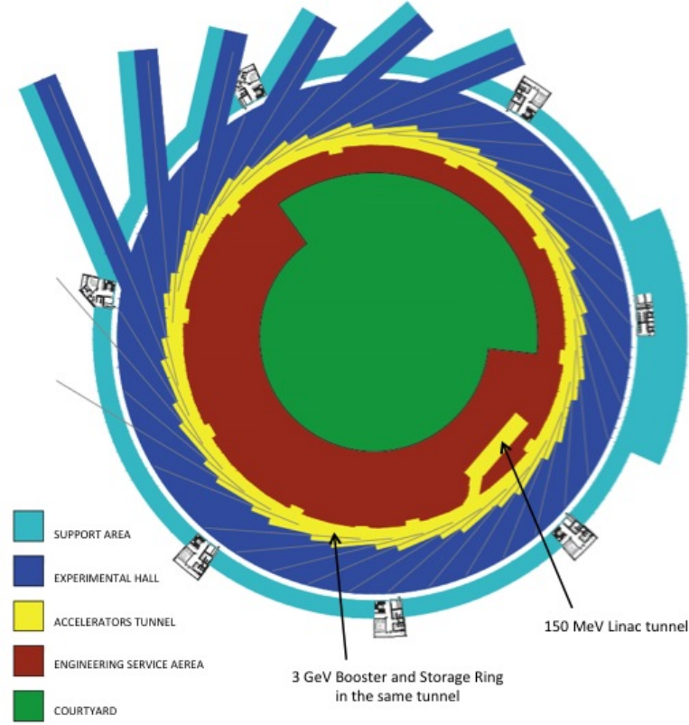
Figure 8 – Sirius building layout, showing all the important areas of the light source, with emphasis on the booster sharing the same tunnel as the storage ring and the 150 MeV LINAC tunnel. The experimental hall will be able to accommodate beamlines up to 100 m long and the requirement for longer beamlines, with possible length up to 450 m, is anticipated. (copied from Sirius (2013).)
