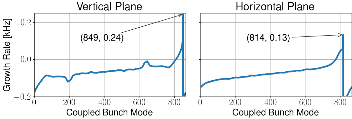
Figure 52 – Transverse coupled-bunch instabilities for the first phase of operation of the Sirius storage ring.
