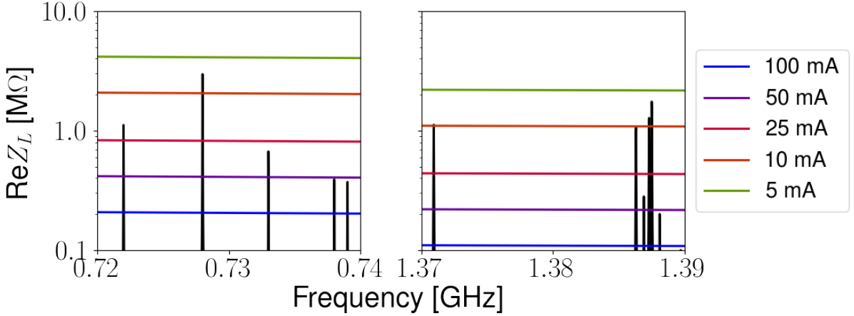
Figure 36 – Longitudinal PETRA 7-Cell cavity impedance compared with the minimum shunt impedance needed to drive coupled-bunch instabilities for several values of total beam current.
