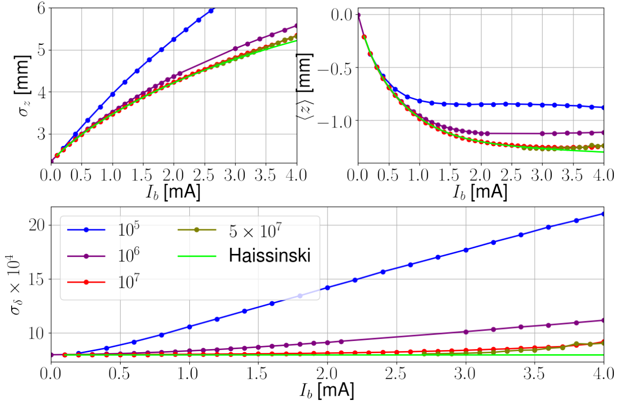
Figure 46 – Tracking results, showing the effect of noise as a function of current for different numbers of macroparticles in the simulation.
