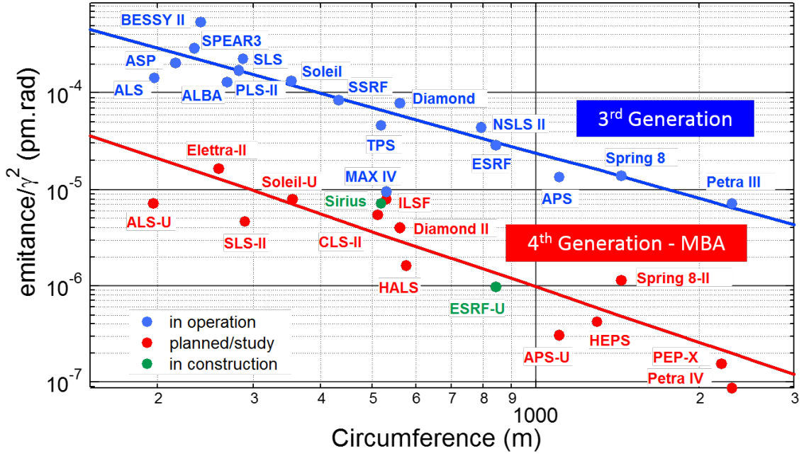
Figure 5 – Natural emittance normalized by relativistic energy squared as a function of ring circumference for several existing Third Generation Light Sources (3 rd GLS) and future 4 th GLS. The blue solid line is a fitting among the 3 rd GLS and the red solid line is a fitting among the 4 th GLS. Note the only 4 th GLS in operation today is MAX-IV. Updated from (LIU; WESTFAHL, 2017).
