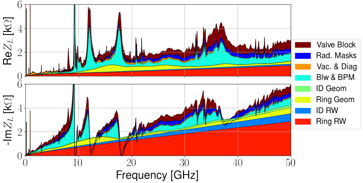
Figure 29 – Longitudinal impedance budget for Sirius.
