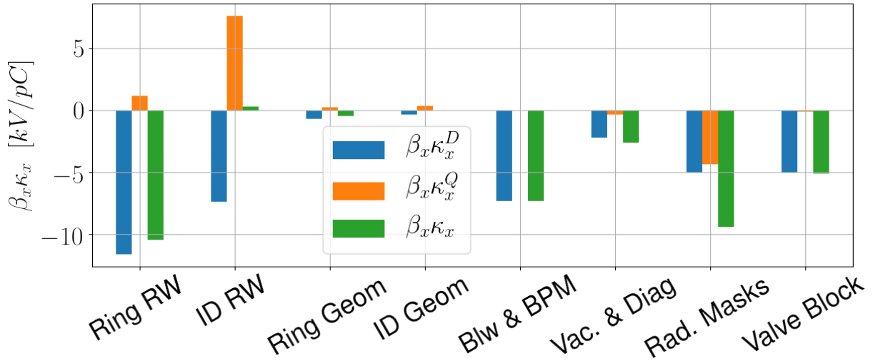
Figure 33 – Horizontal kick factors for single-bunch operation mode.
