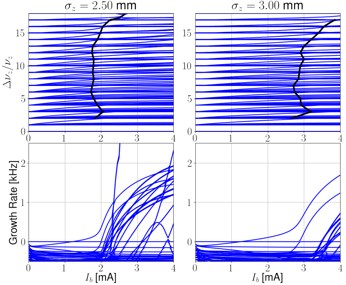
Figure 42 – Mode-coupling instability for two different bunch lengths for phase one of operation. The black lines indicate where different azimuthal modes couple.
