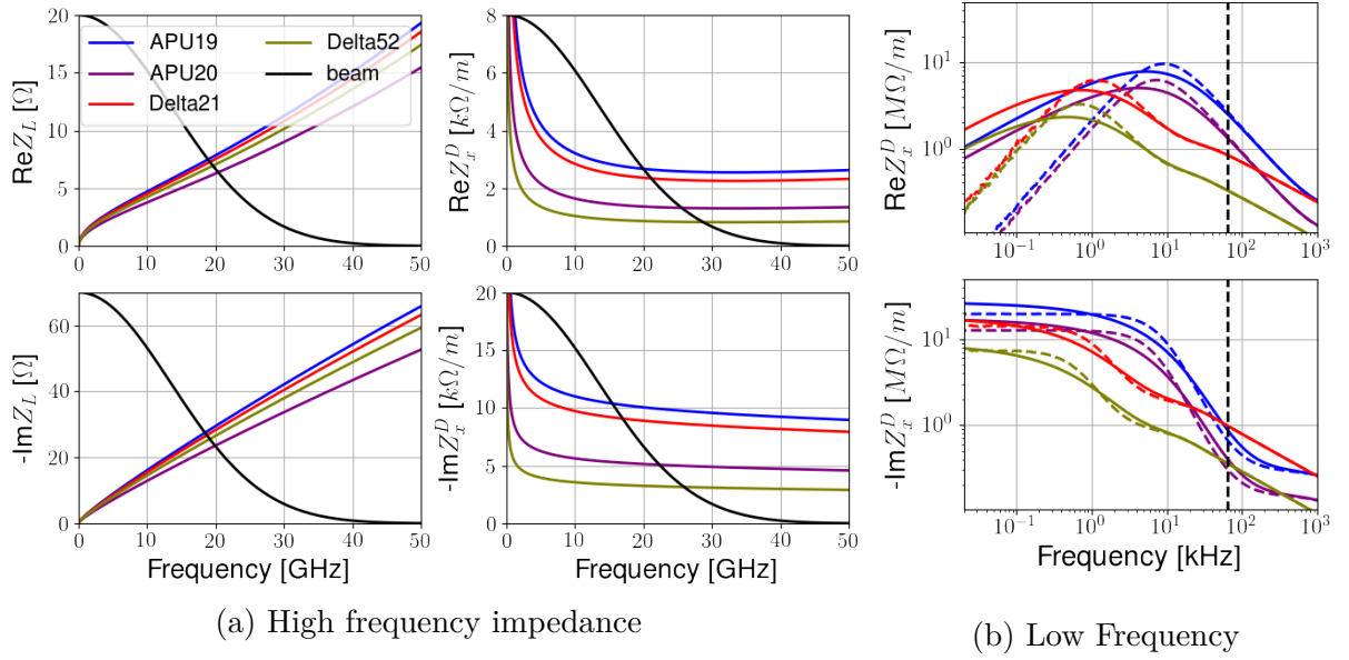
Figure 21 – Wall impedance of the four types of undulators planned for Sirius. Also shown in black in (a) is the power spectrum of a 2.5 mm gaussian bunch in arbitrary units.
