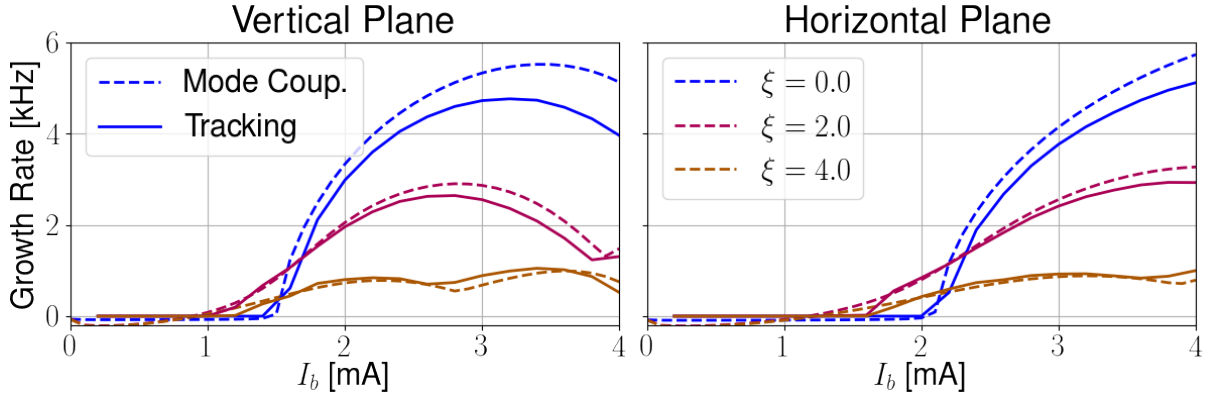
Figure 54 – Transverse single-bunch instabilities for the first phase of operation of the Sirius storage ring, considering the unperturbed longitudinal distribution, without the effects of IBS and potential well distortion.
