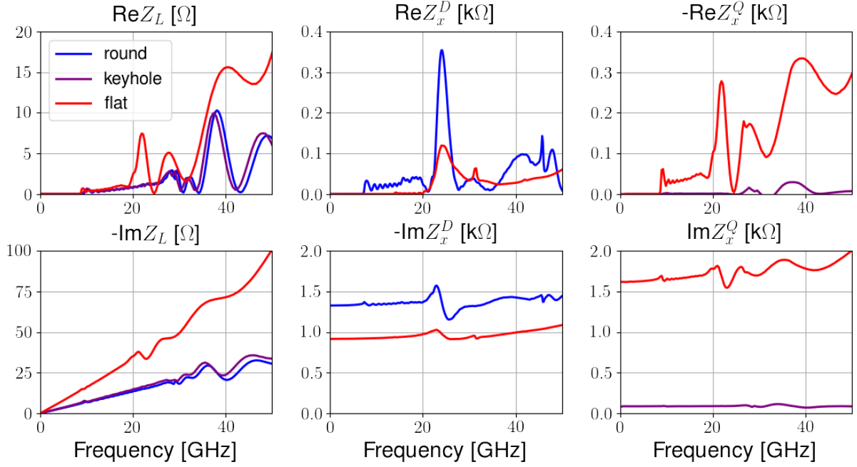
Figure 24 – Longitudinal (left), dipolar horizontal (center) and quadrupolar horizontal (right) impedances for the three models of BC chamber considered. The dipolar horizontal impedance of the keyhole chamber was not calculated yet and the round chamber does not have a quadrupolar impedance.
