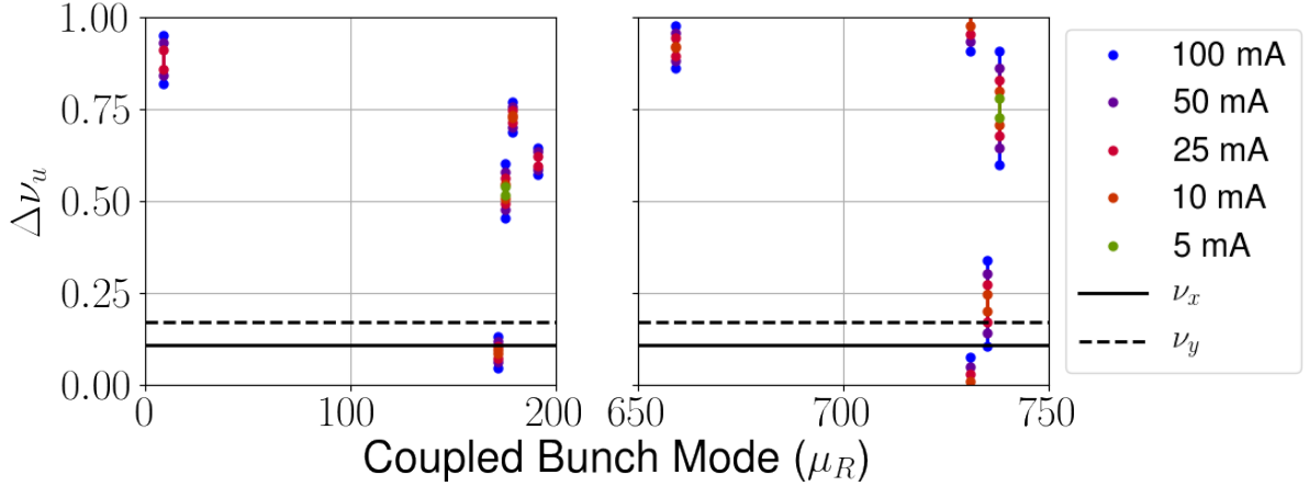
Figure 39 – The horizontal axis indicates the mapping of the RF cavity transverse impedance peak frequencies in the coupled-bunch modes. Vertical axis indicates the fractional part of one revolution frequency in the ring. Black solid horizontal line is the fractional part of \nu_x and black dashed line is the fractional part of \nu_y . The interval defined by the dots is the range in which sampling by the betatron tune corresponds to instability at the indicated current.
