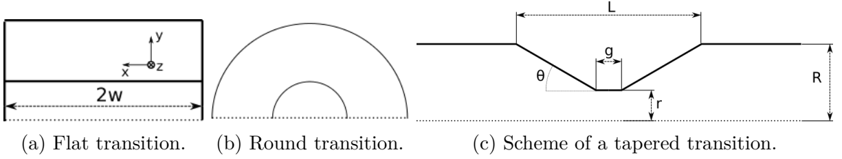
Figure 10 – When r > R the element is called cavity and when r < R it is called collimator. The tapers are the smooth transition regions of the chamber, region where the radius varies. When the transition has no tapers it are called step-in or step-out, depending on the relation between the initial and final radius.
