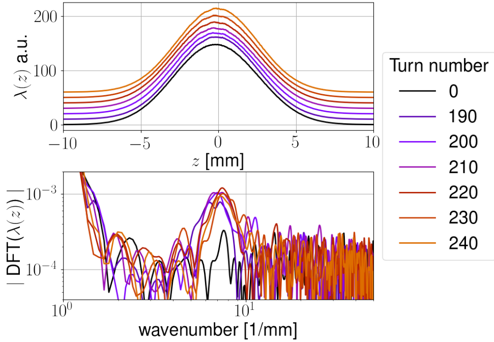
Figure 49 – Longitudinal beam distribution and its discrete Fourier transform for a CSR simulation with beam current of 1.2 mA.
