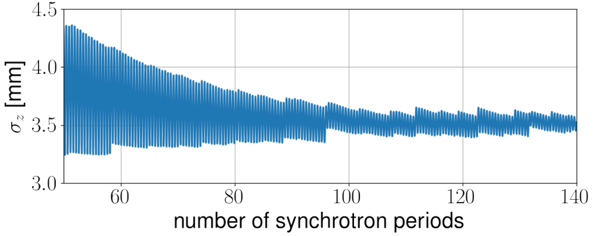
Figure 50 – Time evolution of the bunch size for a beam current of 4.0 mA under the effect of the microbunching instability driven by CSR.
