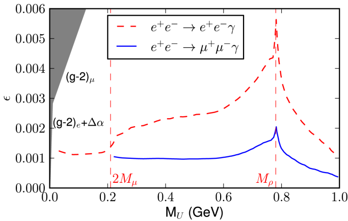
Fig. 1. Discovery potential, defined as the value \epsilon at which N_S/\sqrt{N_B} = 5 , as a function of the dark photon mass M_U , at KLOE/KLOE-2 for an integrated luminosity L = 5 \text{ fb}^{-1} and large angle selection cuts.
