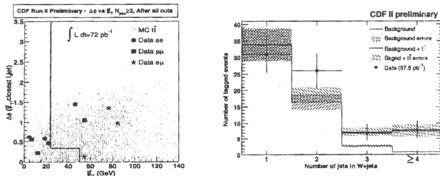
Fig. 13. Left : The five t\bar{t} dilepton candidates in the plane \Delta\phi(\ell_T, \text{nearest } l \text{ or } j) vs. E_T in comparison with the Herwig t\bar{t} Monte Carlo simulation. Right : Number of events in the W + \text{jets} sample with at least one b tag; the 3 and \geq 4 bins are used to extract \sigma_{t\bar{t}} .
