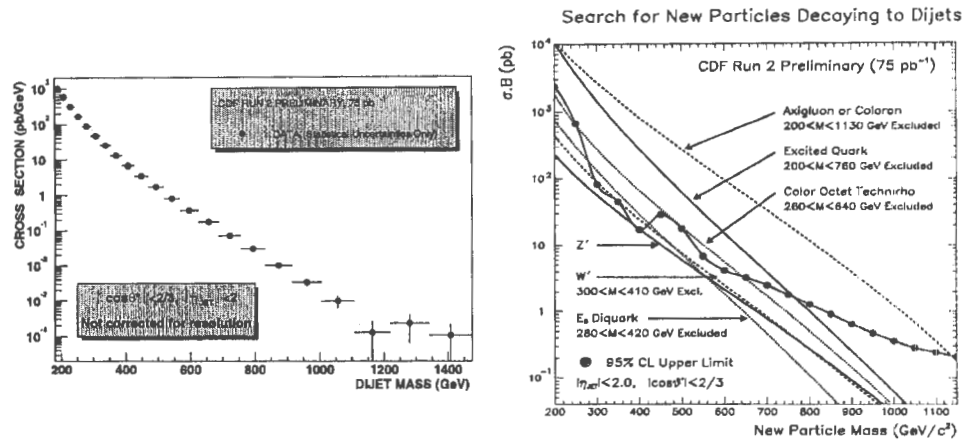
Fig. 15. Left: Dijet mass spectrum. Right: 95% CL upper limits on the cross section times branching ratio for narrow dijet resonances, and predictions for axigluons, flavor universal colorons, excited quarks, Color Octet Technirhos, E6 diquarks, W' and Z' .
