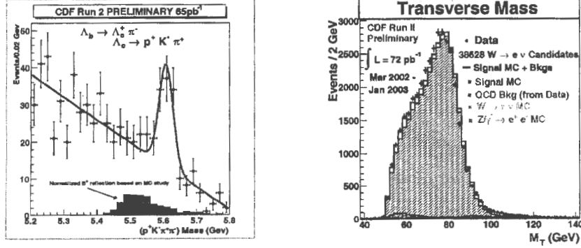
Fig. 10. Left : Observation of \Lambda_b \rightarrow \Lambda_c^+ \pi^- signal. Right : Transverse mass distribution for W \rightarrow e\nu candidate events, overlaid with the expected shape for background and signal.
