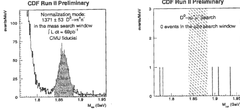
Fig. 8. Search for D^0 \rightarrow \mu^+ \mu^- . Left : Mass spectrum for the normalization mode D^0 \rightarrow \pi^+ \pi^- ; the search window is indicated by the shaded area. Right : Dimuon candidate events; the search window is indicated by the hatched area.
