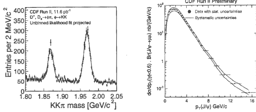
Fig. 6. Left : The reconstructed D^+ \rightarrow \phi\pi^+ and D_s^+ \rightarrow \phi\pi^+ mass distribution. Right : The inclusive J/\psi cross section differential in p_T for |y(J/\psi)| < 0.6 .
