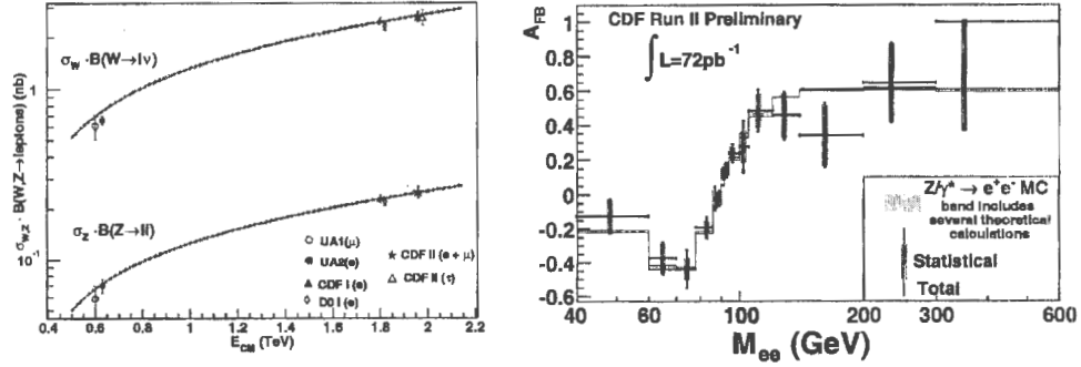
Fig. 11. Left : Cross section measurements for the W and Z boson together with the NNLO prediction. Right : Measurement of the forward-backward asymmetry A_{FB} of electron positron pairs. Predictions by the PYTHIA Monte Carlo simulation are shown as a band.
