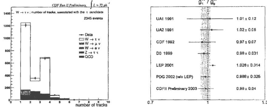
Fig. 12. Left: Signal for W \rightarrow \tau\nu seen in the track multiplicity distribution for the \tau candidates. Right: The ratio of the couplings of the W to the \tau and e as measured by CDF compared to earlier measurements.
