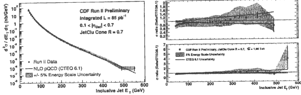
Fig. 14. Left: Measurement of the inclusive jet cross section, compared to the NLO QCD expectation using the CTEQ 6.1 parton density functions. The variation in the cross section due to the 5% energy scale uncertainty is shown as a band. The two lines indicate the uncertainty in the cross section prediction due to the PDF. Right: The ratio of data and theory.
