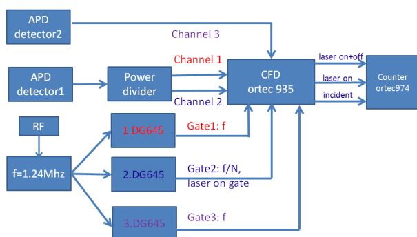
Figure 3: Schematic of channel consistency measurement.
