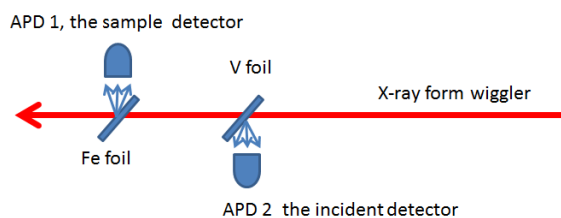
Figure 4: Schematic of XAS experiments.
