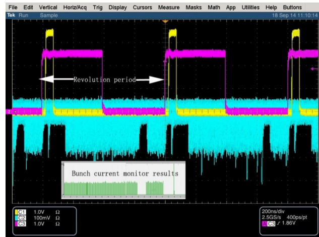
Figure 2: Gate signals used for synchronization with the camshaft pulse. The oscilloscope is working in the infinite remainder seen mode.
