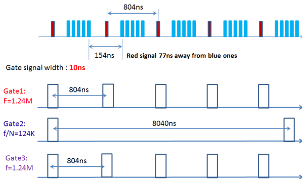
Figure 1: Laser on and laser off gate signals used for selecting the camshaft pulse.
