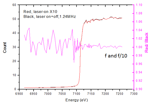
Figure 5: XAS results with different gate signal, presenting laser on (124 kHz) and laser on +off (1.24 Mhz), respectively.
