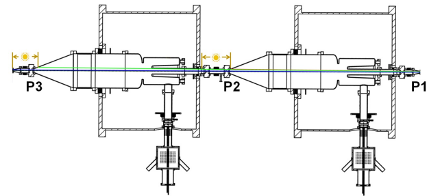
Figure 3: The layout of cavity string. Beam passes right to left through the cavity string.
