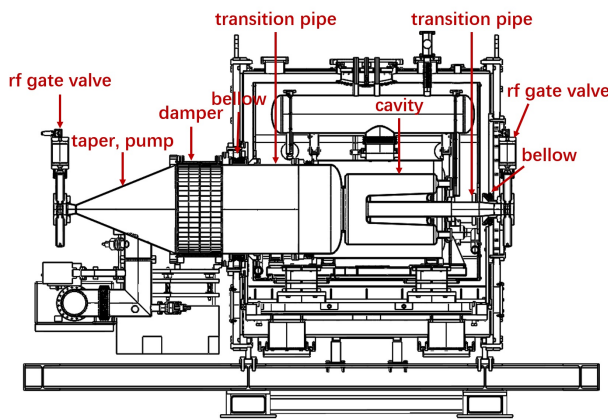
Figure 2: A set of the compact 166.6 MHz cavity equipment.
