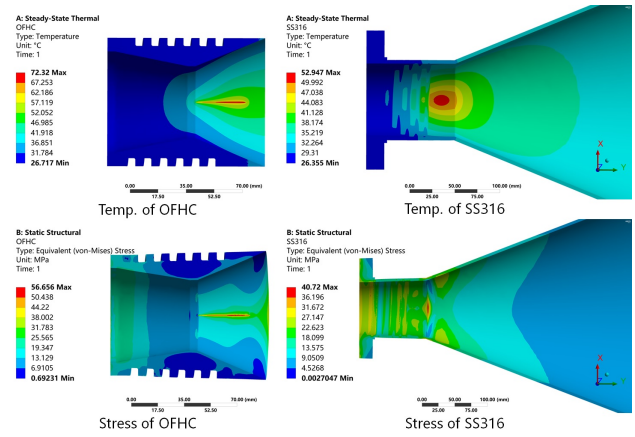
Figure 5: Coupled-simulation results of the collimator with cooling water channel.
