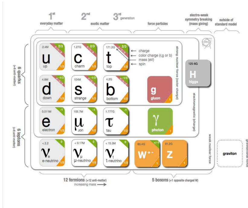
FIGURE 1.1: The Standard Model of particle physics, consisting of the twelve fundamental fermions, four fundamental gauge bosons and the Higgs Boson [6].
