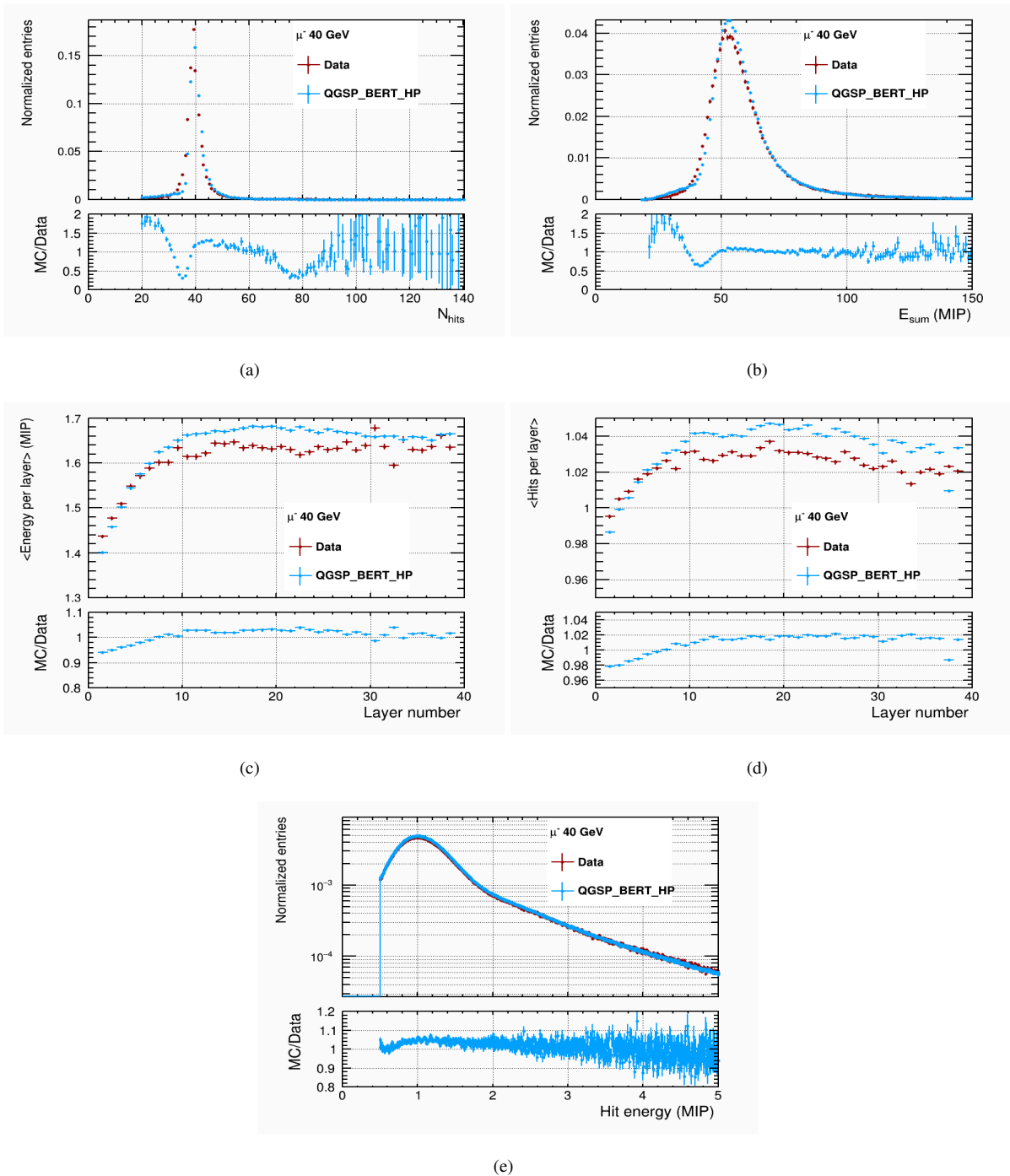
FIGURE 6.1: Comparison of standard reconstructed quantities for 40 GeV muon using testbeam data (red) and simulated data (blue). Lower window shows the ratio of simulated data to testbeam data. (a) The number of hits distributions per event ( N_{\text{hits}} ). (b) Distribution of the visible energy deposit in MIP equivalents. (c) Mean energy per layer in MIPs. (d) Mean number of hits per layer. (e) Hit energy distribution in MIP equivalents
