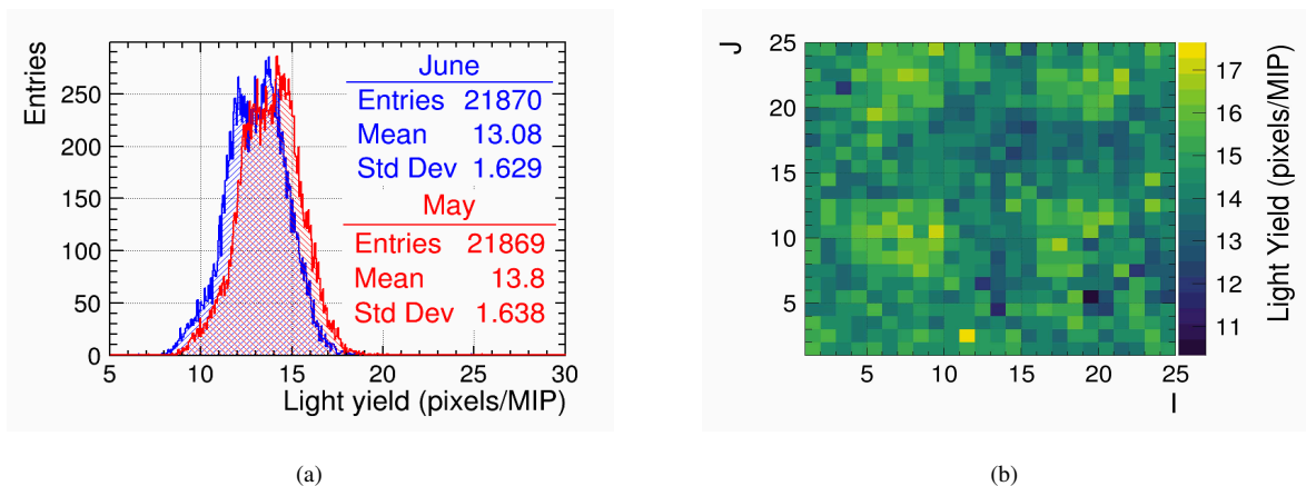
FIGURE 4.16: (a) Light yield measured for AHCAL channels for the two testbeam periods. The mean light yield is \approx 13.08 pixels/MIP for the June testbeam period and \approx 13.8 pixels/MIP for the May testbeam period and a spread of \approx 1.6 pixels/MIP. (b) Light yield distribution of the AHCAL layer number 12 in I and J coordinates.
