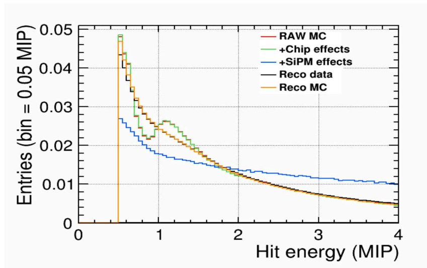
FIGURE 2.9: The simulation of different detector effects. The orange curve shows the final digitized hit amplitude.
