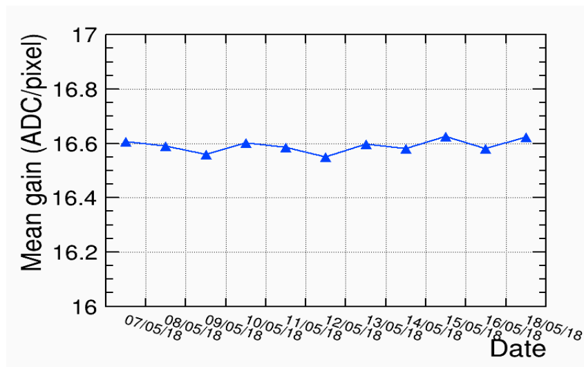
FIGURE 4.11: Mean gains obtained for the May 2018 testbeam period
