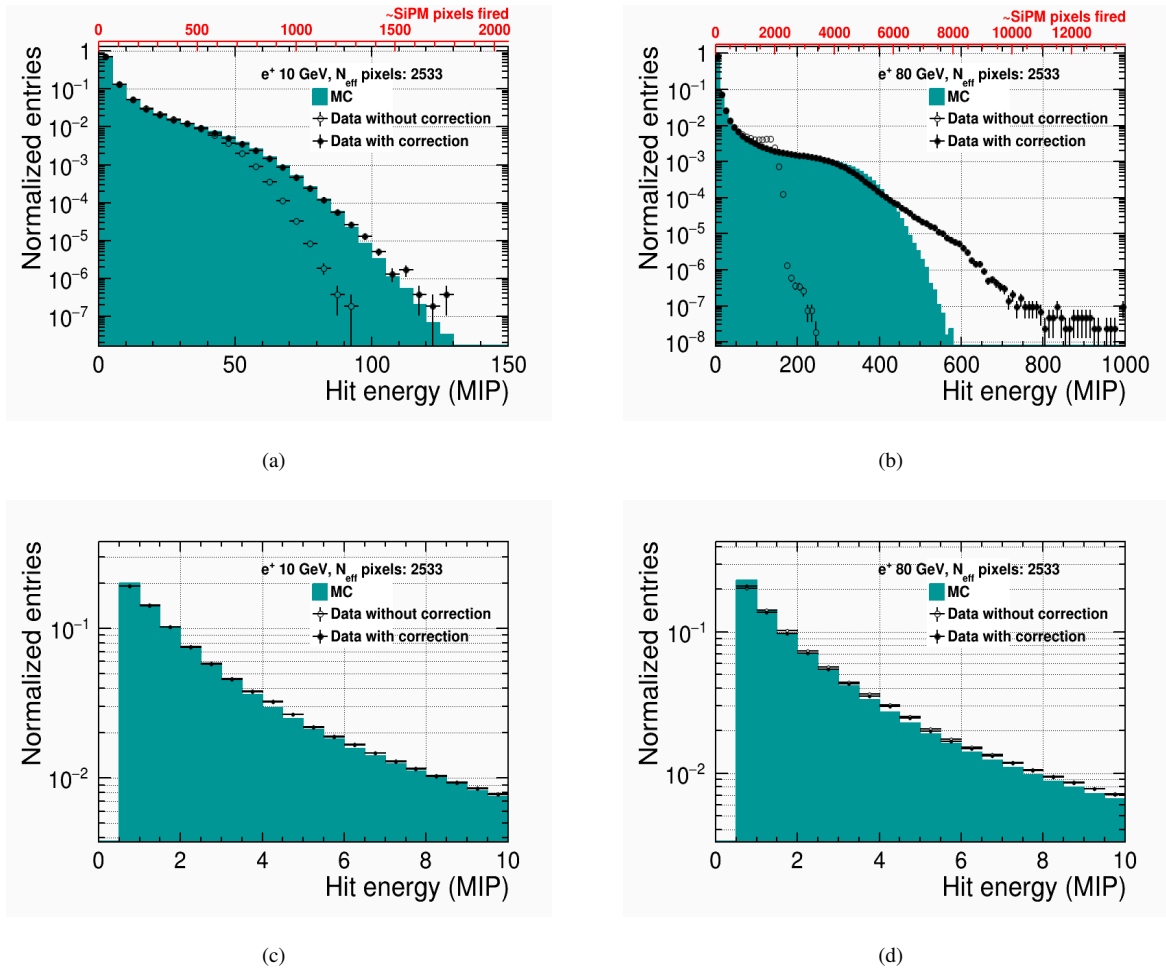
FIGURE 6.2: Comparison of the hit energy distribution for electron showers from simulated data (green) and testbeam data (black) after applying a saturation correction using 2533 as the number of effective pixels. (a) Hit energy distribution for 10 GeV and (b) Hit energy distribution for 80 GeV. Hit energy distribution in the low energy deposits in range between 0-10 MIPs for beam energy at (c) 10 GeV and (d) 80 GeV.
