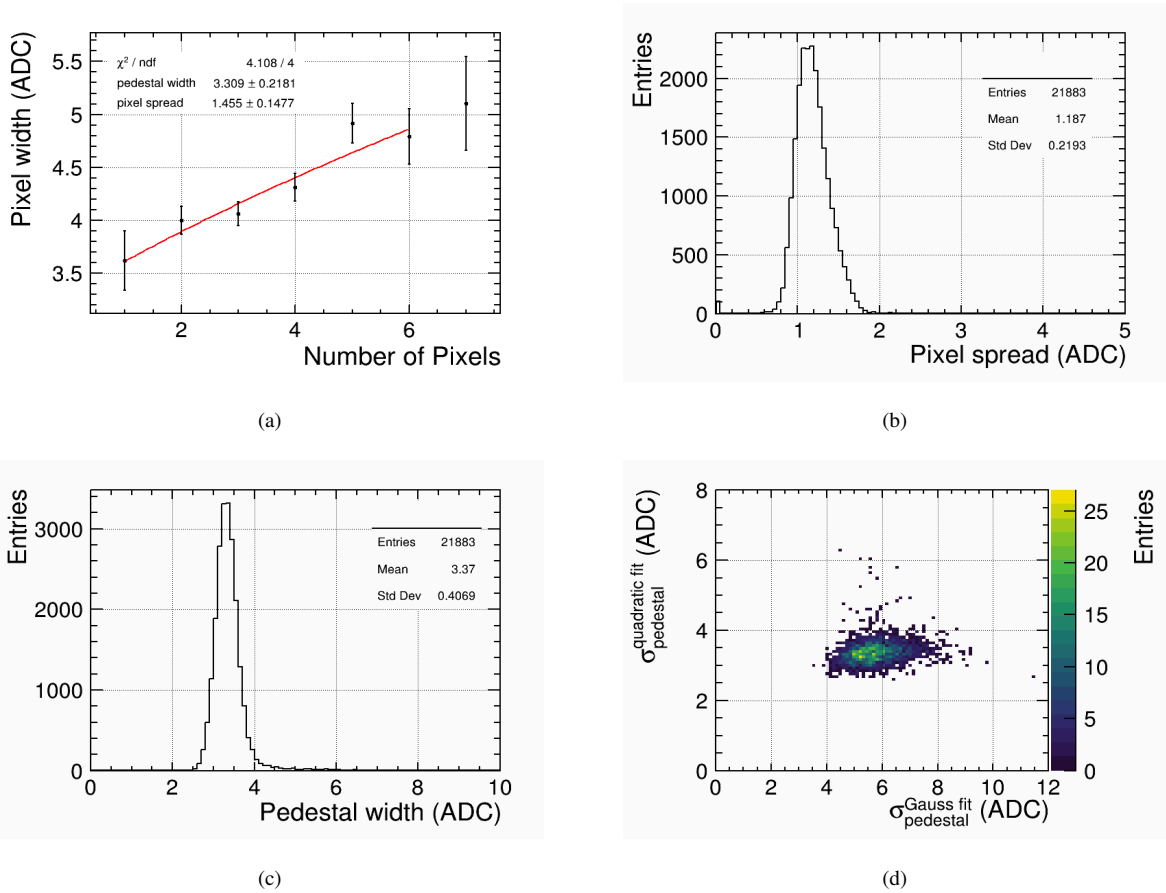
FIGURE 4.5: (a) SiPM pixel width in ADC plotted against the number of pixels for a single SiPM. The width of each peak \sigma_0 to \sigma_6 increases from \approx 3.6 ADC to \approx 5.1 ADC due to inter and intra pixel gain variation. (b) Pixel spread extracted from the quadratic fit. (c) Pedestal width extracted from the quadratic fit. (d) Correlation for the channels between pedestal width extracted from quadratic fit and pedestal width extracted from a pedestal run.
