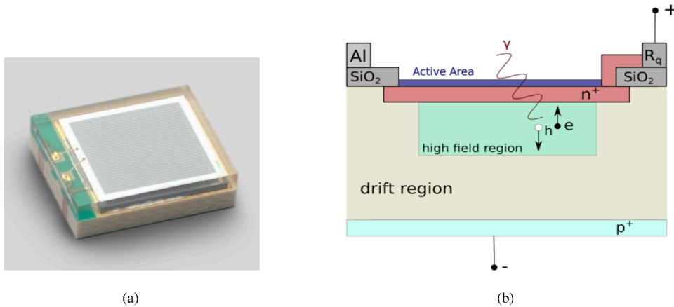
FIGURE 2.1: (a) Picture of a SiPM [83]. (b) Schematic of a single pixel in a SiPM.
