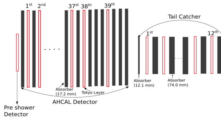
FIGURE 3.3: Schematic of the AHCAL prototype and Tail-Catcher layer configuration of the June 2018 testbeam campaign at the SPS-CERN.
