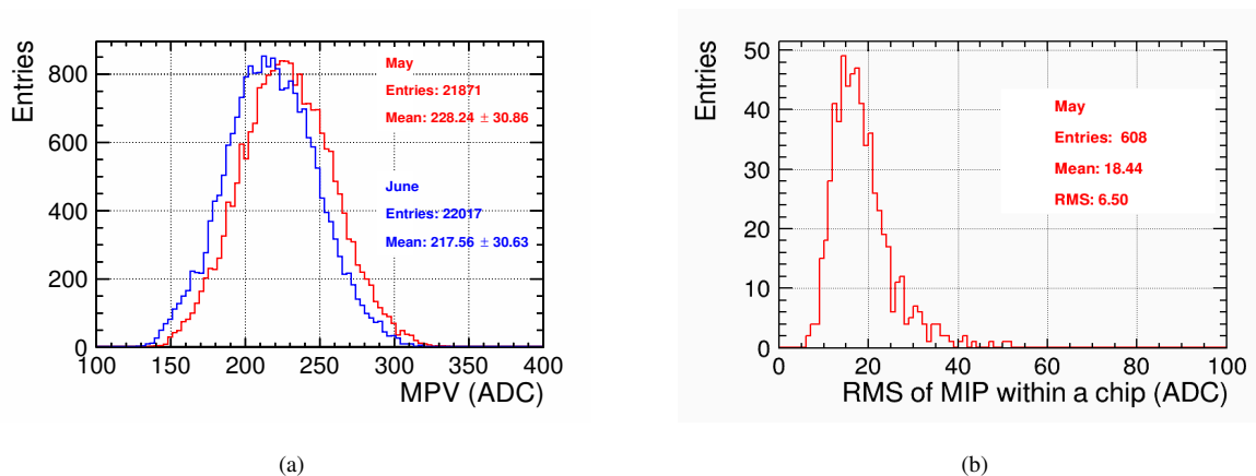
FIGURE 4.14: (a) MIP constants extracted for the AHCAL channels using muons runs from May and June 2018 testbeam data. A mean value of roughly 220 ADC is obtained. (b) The spread within a chip is \approx 18.4 ADC using muon testbeam data from May 2018 [97]
