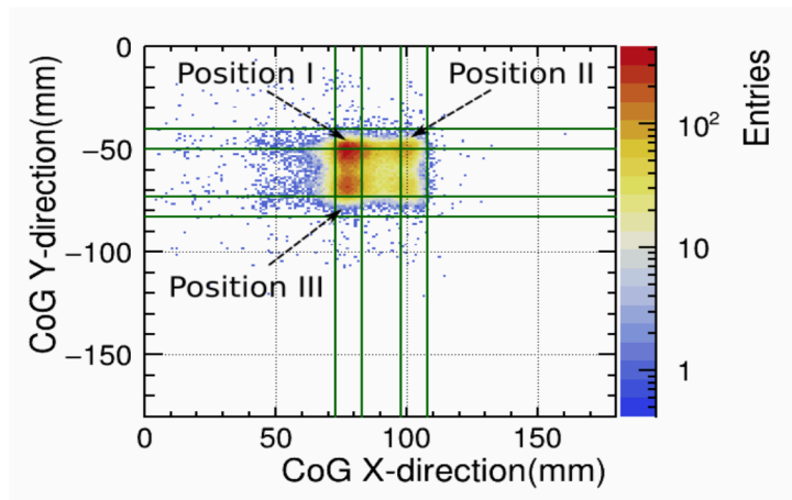
FIGURE 6.3: Centre of gravity plot, depicting position I, II and III tested for saturation correction studies. The green marking shows the region of AHCAL tile acceptance.
