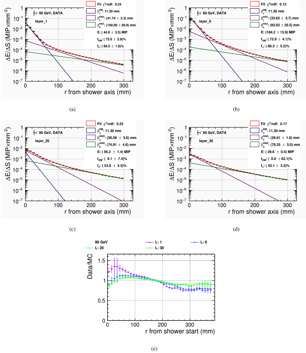
FIGURE 7.42: Fits performed using Eq. 7.21 with fixed \beta_c^{\text{EM}} for radial shower shapes at various depths with beam energy at 80 GeV using testbeam data (a) at the beginning of the shower, (b) at the maximum of the shower, (c) at an intermediate layer (d) and layer at the end of the shower. (e) Shows the ratio between data and QGSP BERT HP for 80 GeV pion shower.
