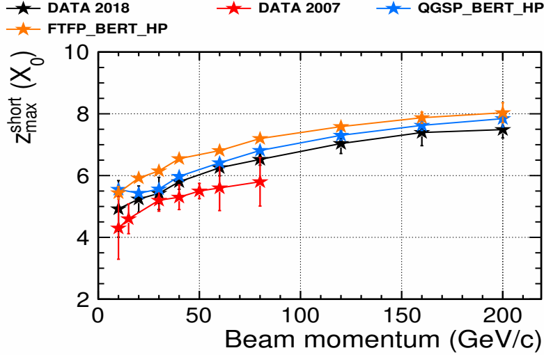
FIGURE 7.23: Maximum of the “short” component in units of radiation length X_0 as a function of pion beam energies. The shower maximum is obtained for 2018 testbeam data (black) and simulations with QGSP_BERT_HP (blue) and FTFP_BERT_HP (orange) physics list, along with the comparison to the 2007 testbeam data (red) from the physics prototype [110].
