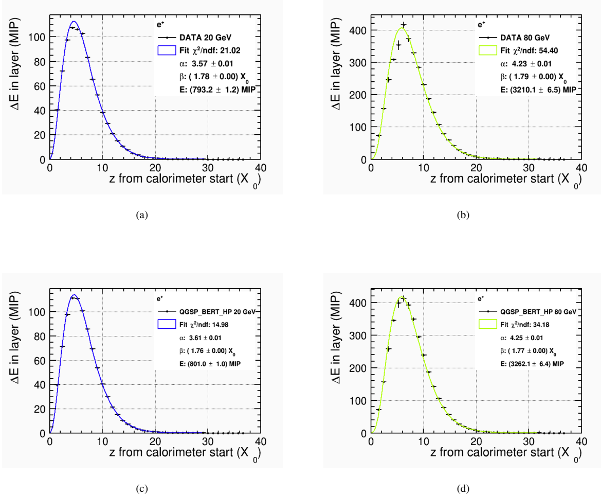
FIGURE D.1: Fits performed to electron longitudinal shower profile using Eq. 7.1 shown by solid line. (a) 20 GeV and (b) 80 GeV electron shower from testbeam data. (c) 20 GeV and (d) 80 GeV electron shower from simulated data using QGSP BERT HP physics lists.
