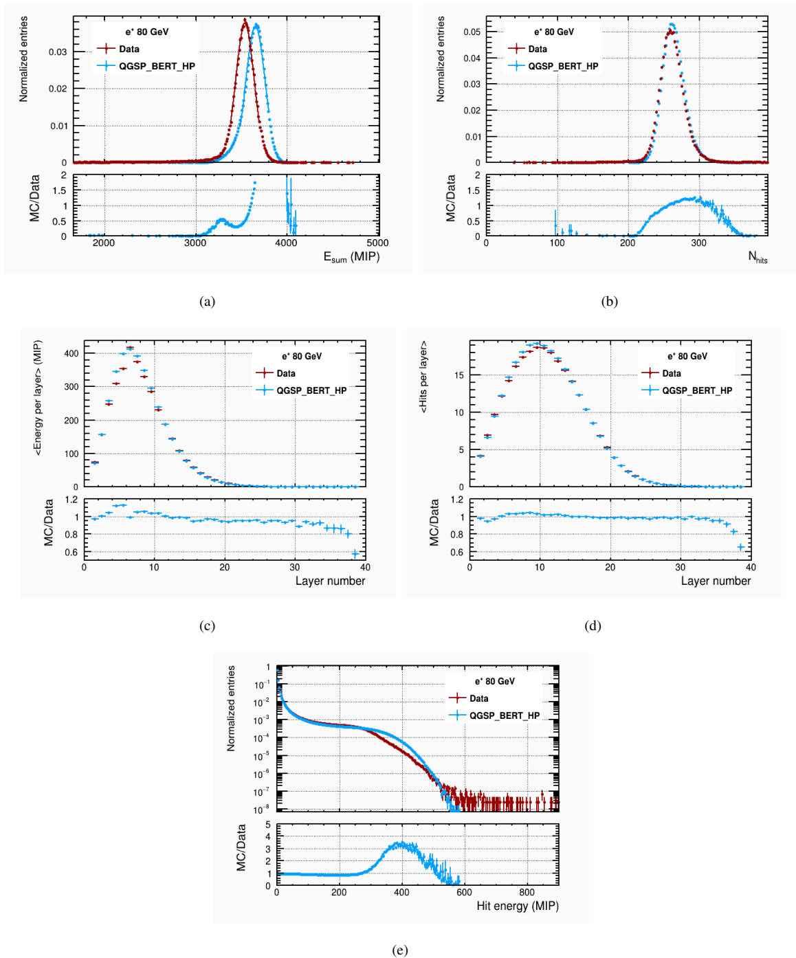
FIGURE 6.10: Comparison of standard reconstructed quantities for 80 GeV electron showers using testbeam data (red) and simulated data (blue). Lower window shows the ratio of simulated data to testbeam data. (a) The visible energy deposition, (b) the number of hits n_{\text{Hits}} , (c) Mean energy per layer, (d) Mean number of hits per layer and (e) Hit energy distribution for 80 GeV electron showers using testbeam data and simulation.
