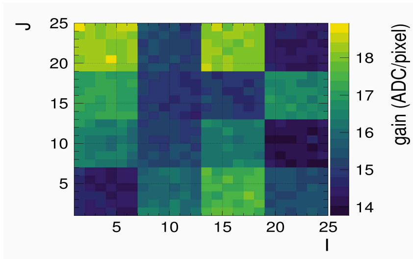
FIGURE 4.9: Gain map in I and J coordinates for layer 12 of AHCAL.
