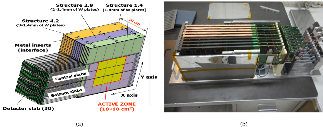
FIGURE 1.13: (a) Schematic 3D view of the SiW-ECAL physics prototype [72]. (b) Picture of SiW-ECAL technological prototype with 7 layers inside the aluminum stack [73].
