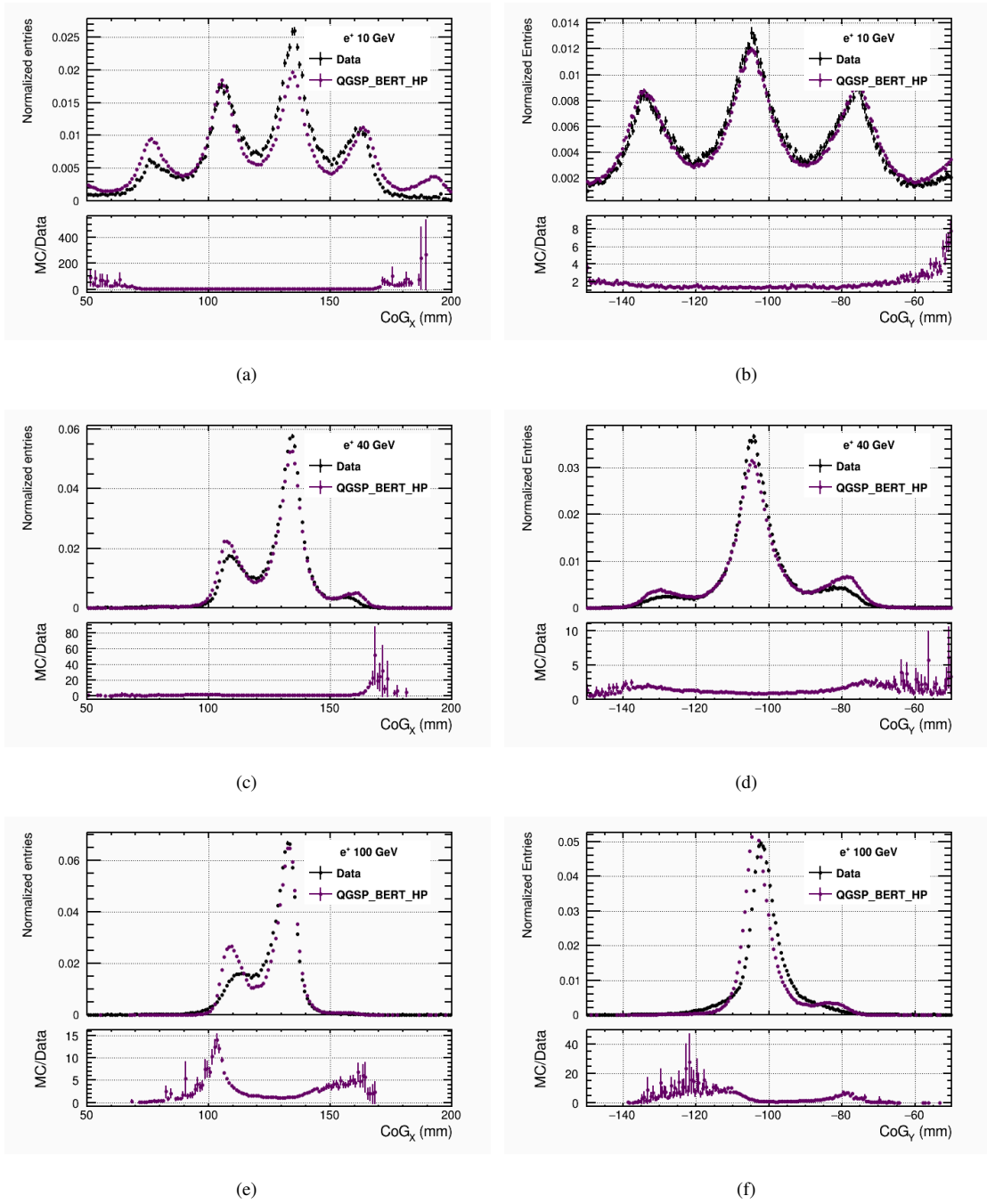
FIGURE B.2: Center of gravity distributions in x and y-directions using electron showers from testbeam data and simulated data with QGSP_BERT_HP physics list.
