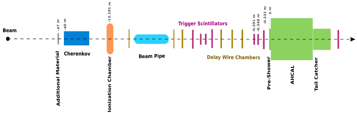
FIGURE 3.4: A schematic illustration of the beamline setup at the CERN SPS H2 beamline in June 2018. The black dashed trajectory indicates the hypothetical path of a particle ( \mu^\pm , e^\pm , \pi^\pm ), which first traverses an additional material, then beam instruments (Čerenkov detector, ionization chamber, delay wire chambers, beam pipe and trigger scintillators) and then lastly enters the pre-shower and analog hadron calorimeter. The pre-shower is the origin where the z-axis is defined along the beamline.
