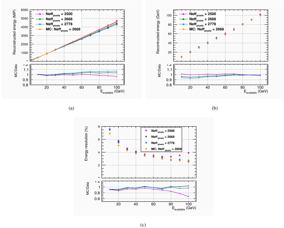
FIGURE 6.9: (a) The upper window is the energy reconstructed as a function of the beam energy from MC and testbeam data with a saturation correction using different numbers of effective pixels. The lower window is the ratio of MC to testbeam data for different numbers of effective pixels. (b) Energy linearity after performing linear fit. (c) The upper window shows the comparison of the shower energy resolution between MC and data with the saturation correction applied using different numbers of effective pixels. The lower window shows the ratio of simulated data to testbeam data for a different number of effective pixels.
