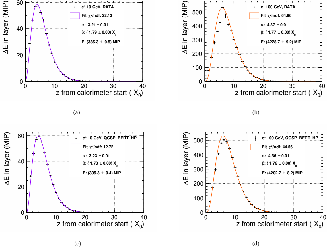
FIGURE 7.5: Fits performed to longitudinal shower profile shown by solid line using Eq. 7.1 (a) for 10 GeV electron shower and (b) for 100 GeV electron shower from testbeam data, and (c) for 10 GeV electron shower and (d) for 100 GeV electron shower from simulated data using QGSP_BERT_HP physics lists.
