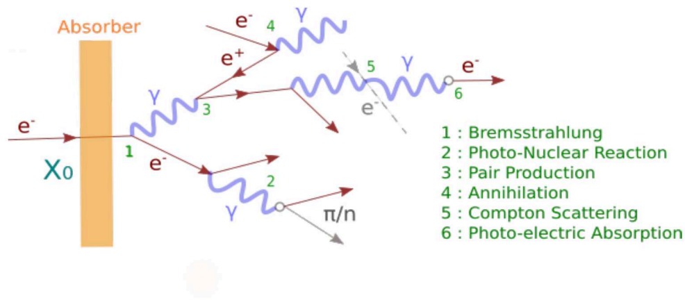
FIGURE 1.9: Schematic depiction of an electromagnetic shower induced by an electron. Electrons and positrons are represented with solid, red line, and photons with wiggly, blue line. Contribution from different processes are marked with numbers.
