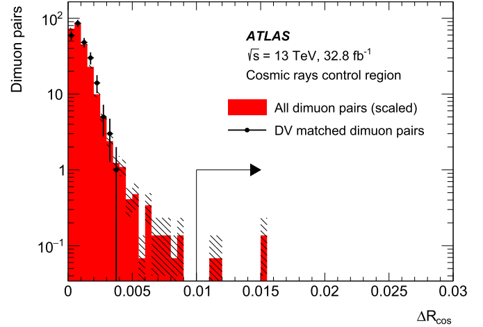
Fig. 1. \Delta R_{\cos} for dimuon events observed in the cosmic rays control region in collision data. The filled histogram includes all dimuon pairs, with the statistical uncertainties represented by the shaded bands. The dots indicate the subset forming a DV candidate. The distribution of all dimuon pairs is scaled to the DV distribution with \Delta R_{\cos} < 0.004 . The arrow illustrates the signal region requirement of \Delta R_{\cos} > 0.01 .
