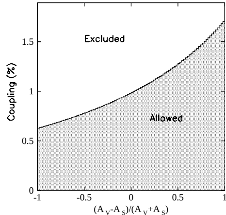
FIG. 4. Limit on the lepton number violation process \bar{\nu}_\mu e^- \rightarrow \mu^- \bar{\nu}_e as a function of the scalar and vector couplings (A_V - A_S)/(A_V + A_S) . The non-shaded region is excluded by this result.
