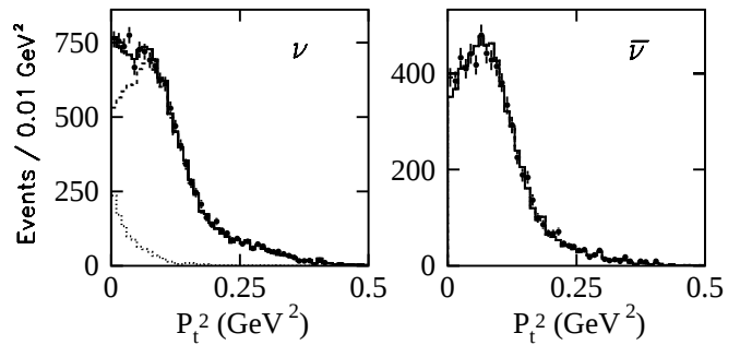
FIG. 2. Transverse momentum distributions for data (crosses) and Monte Carlo (solid) for right-sign neutrino events (left) and right-sign anti-neutrino events (right). The plot on the left is broken down into background only (dashed) and IMD signal (dotted). The plot on the right shows Monte Carlo background only.
