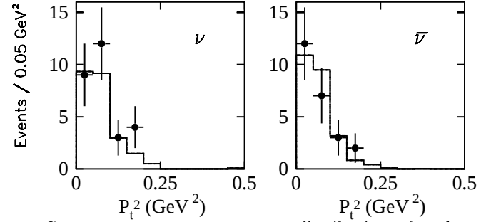
FIG. 3. Transverse momentum distributions for data (crosses) and Monte Carlo (solid) for neutrino events (left) and anti-neutrino events (right) with a wrong-sign muon. A LNV signal would appear as an excess of events in anti-neutrino mode.
